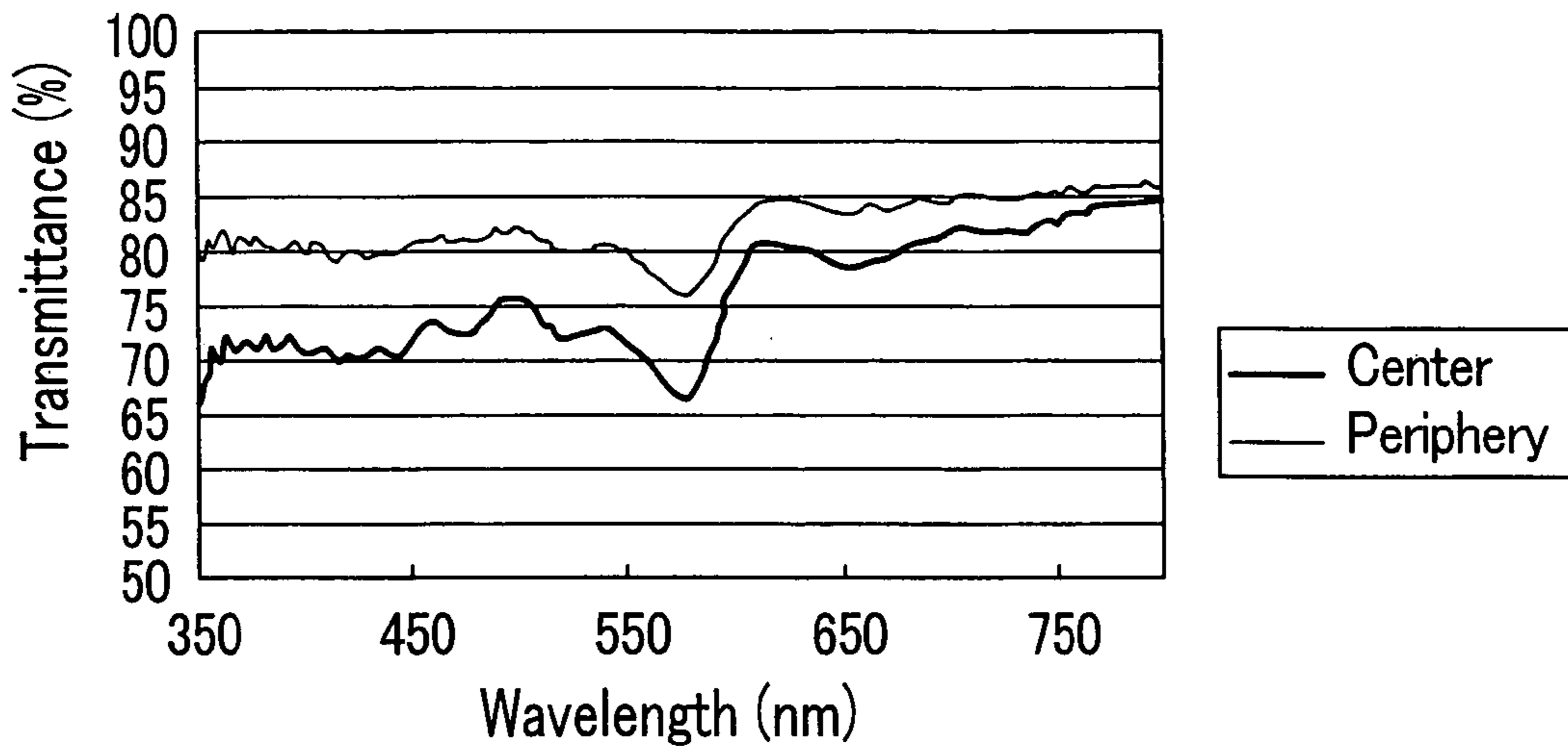
Transmission Spectra of Wavelength Selective Absorption Film for CDT
