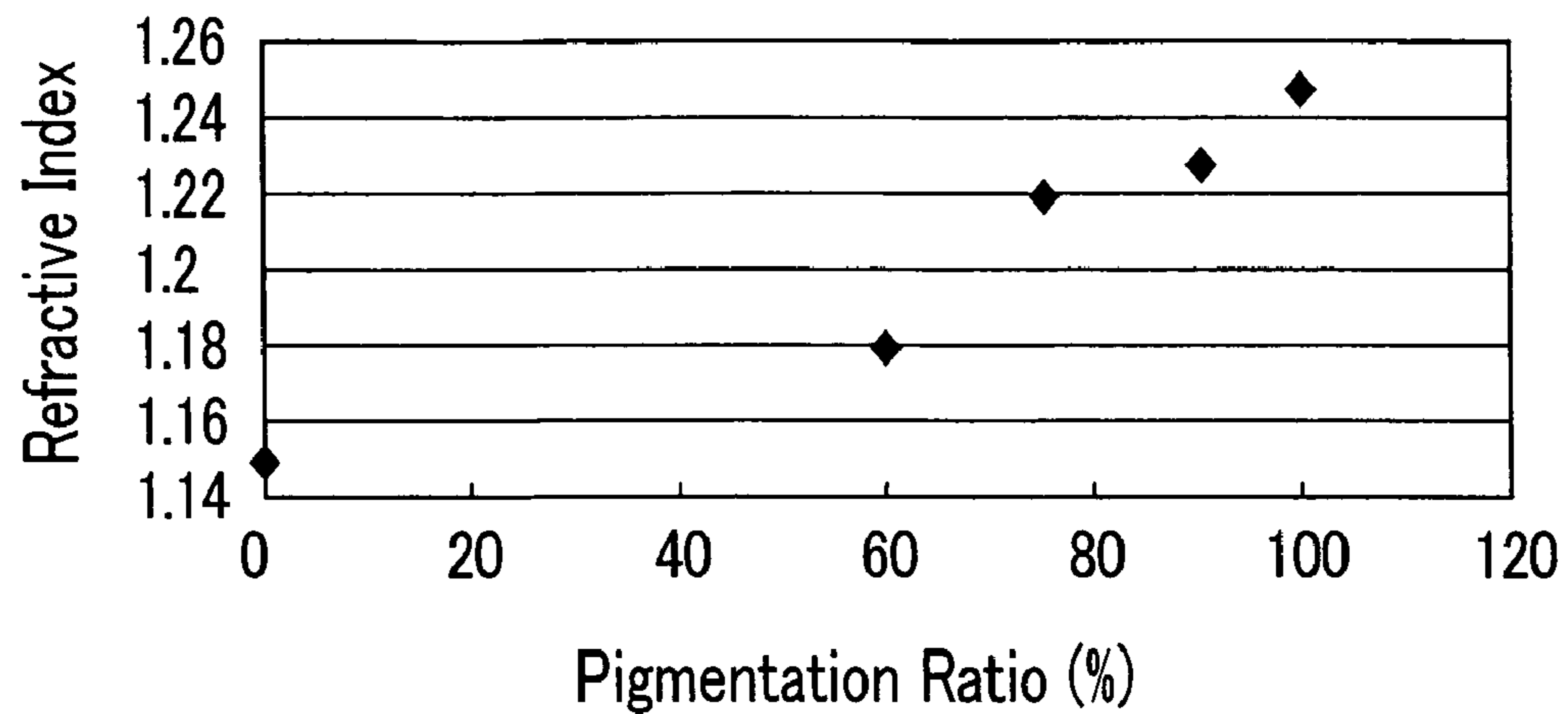
Relationship between Pigmentation Ratio and Refractive Index under Oxygen Plasma Irradiation
