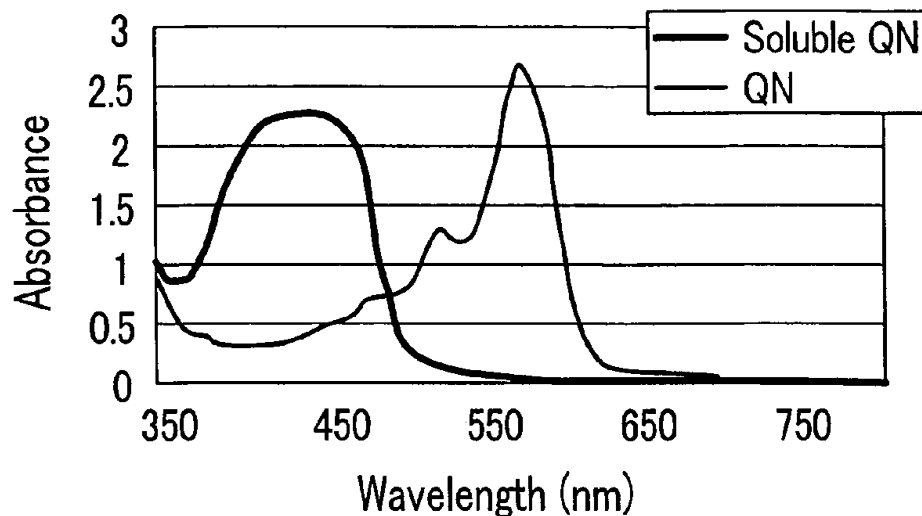
Spectral Change between Soluble Quinacridon and Insoluble Quinacridon
