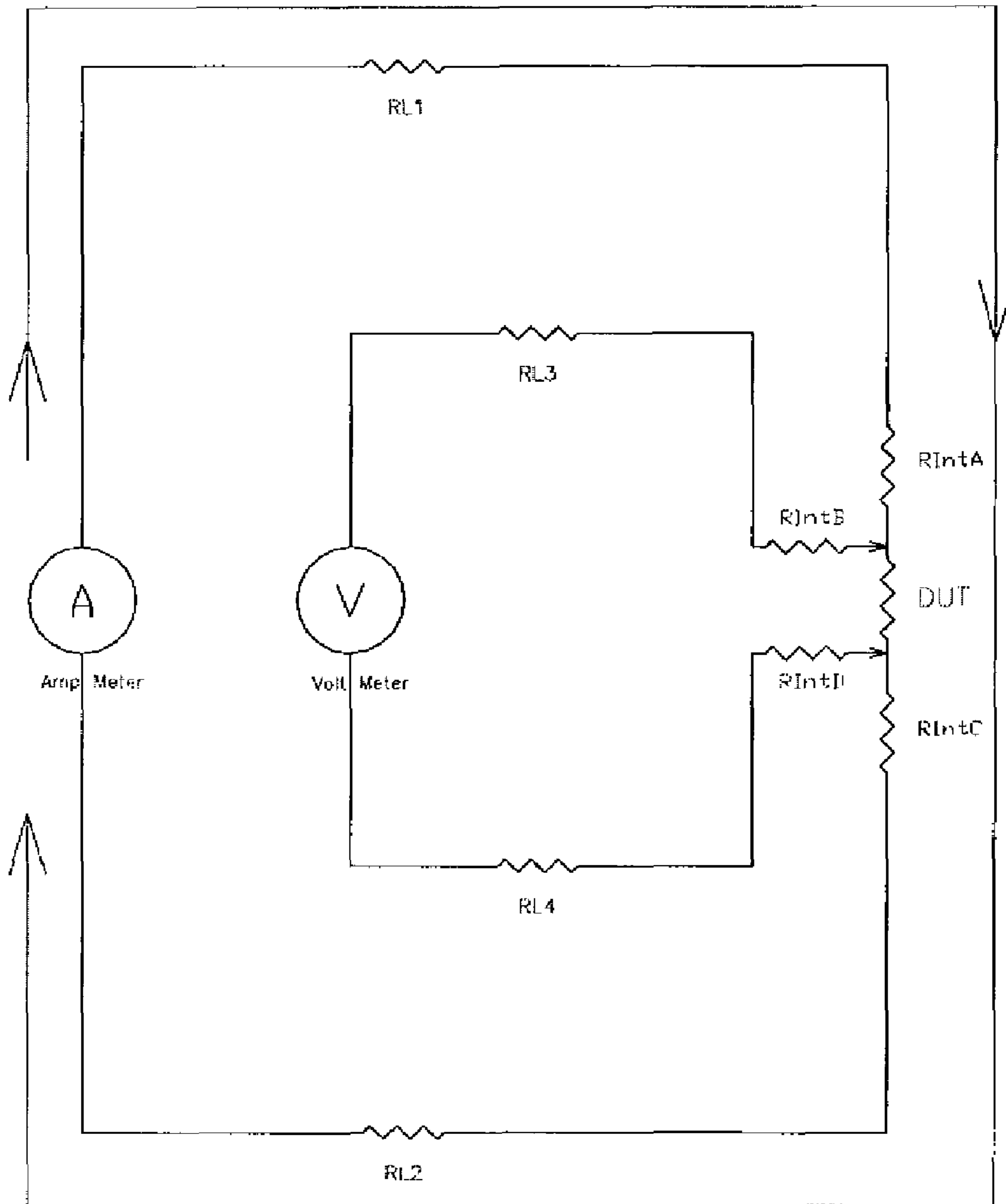
Figure 6 CurrentLoop 1
