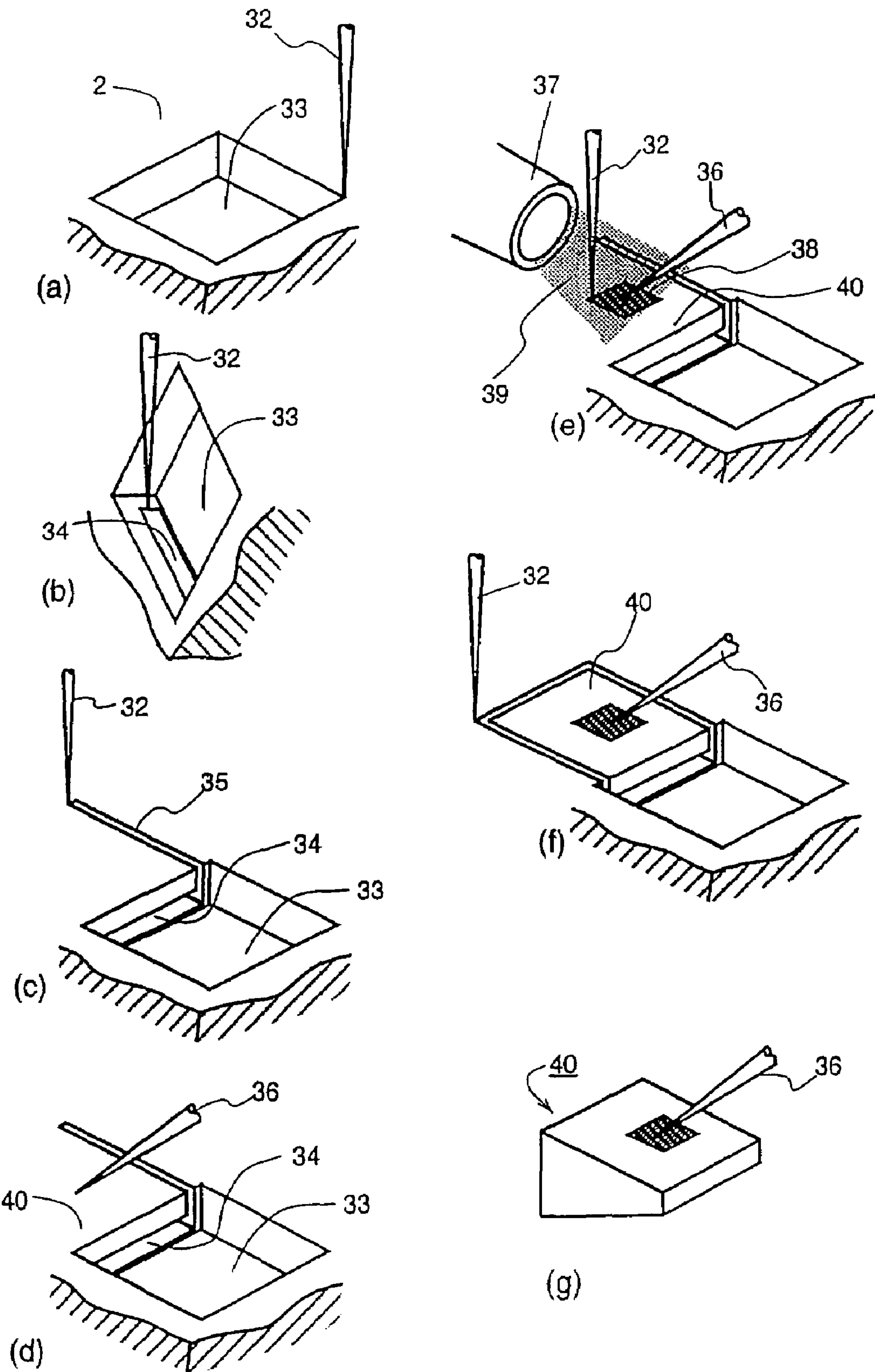
FIG.4 (PRIOR ART)
