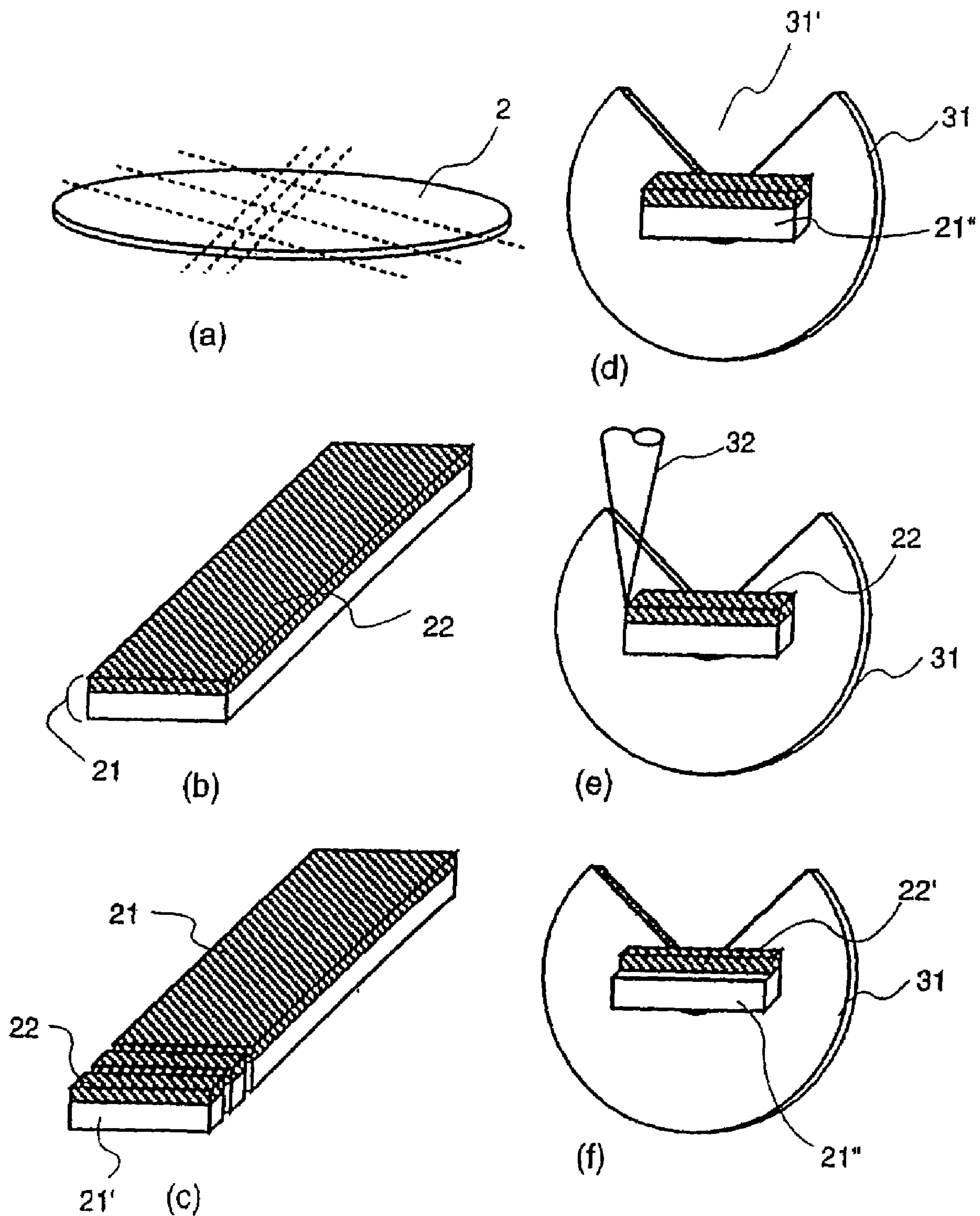
FIG.3 (PRIOR ART)
