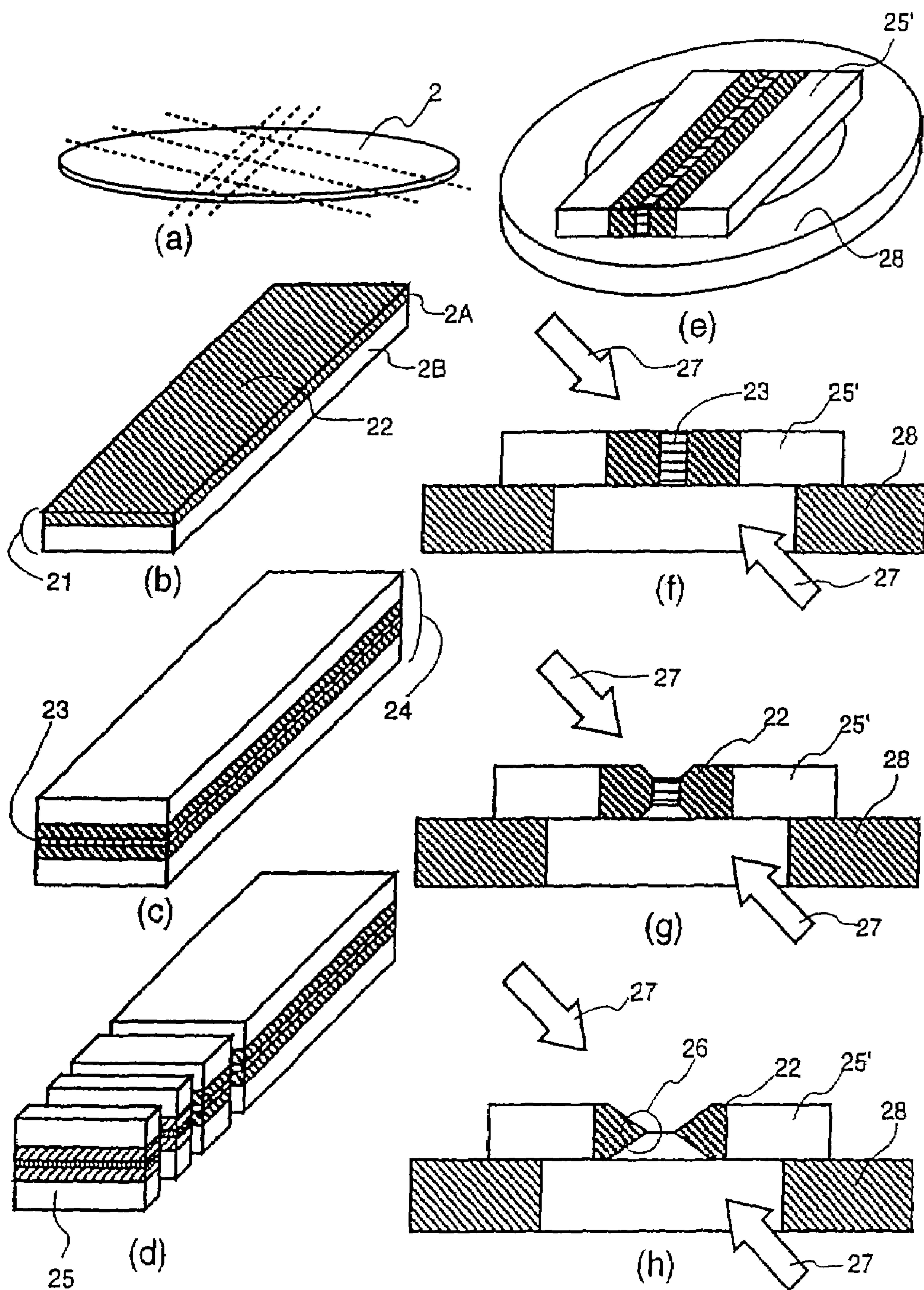
FIG.2 (PRIOR ART)
