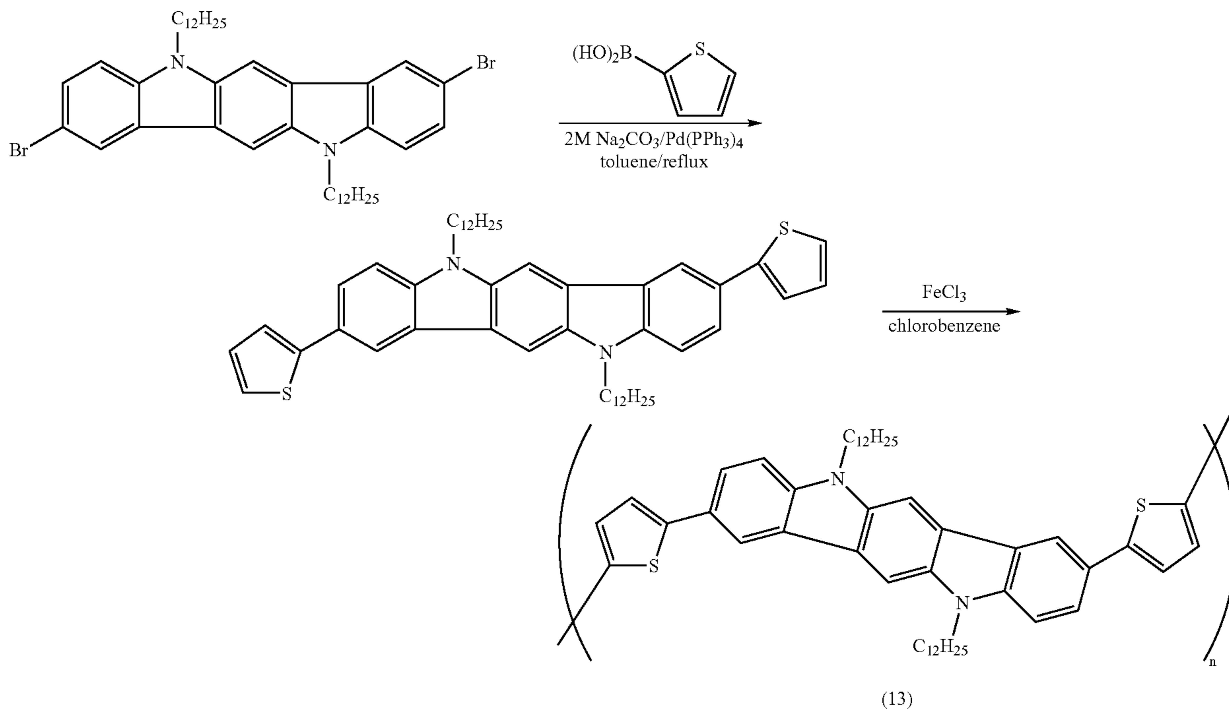
Scheme 3. Synthesis of polymer (13).
