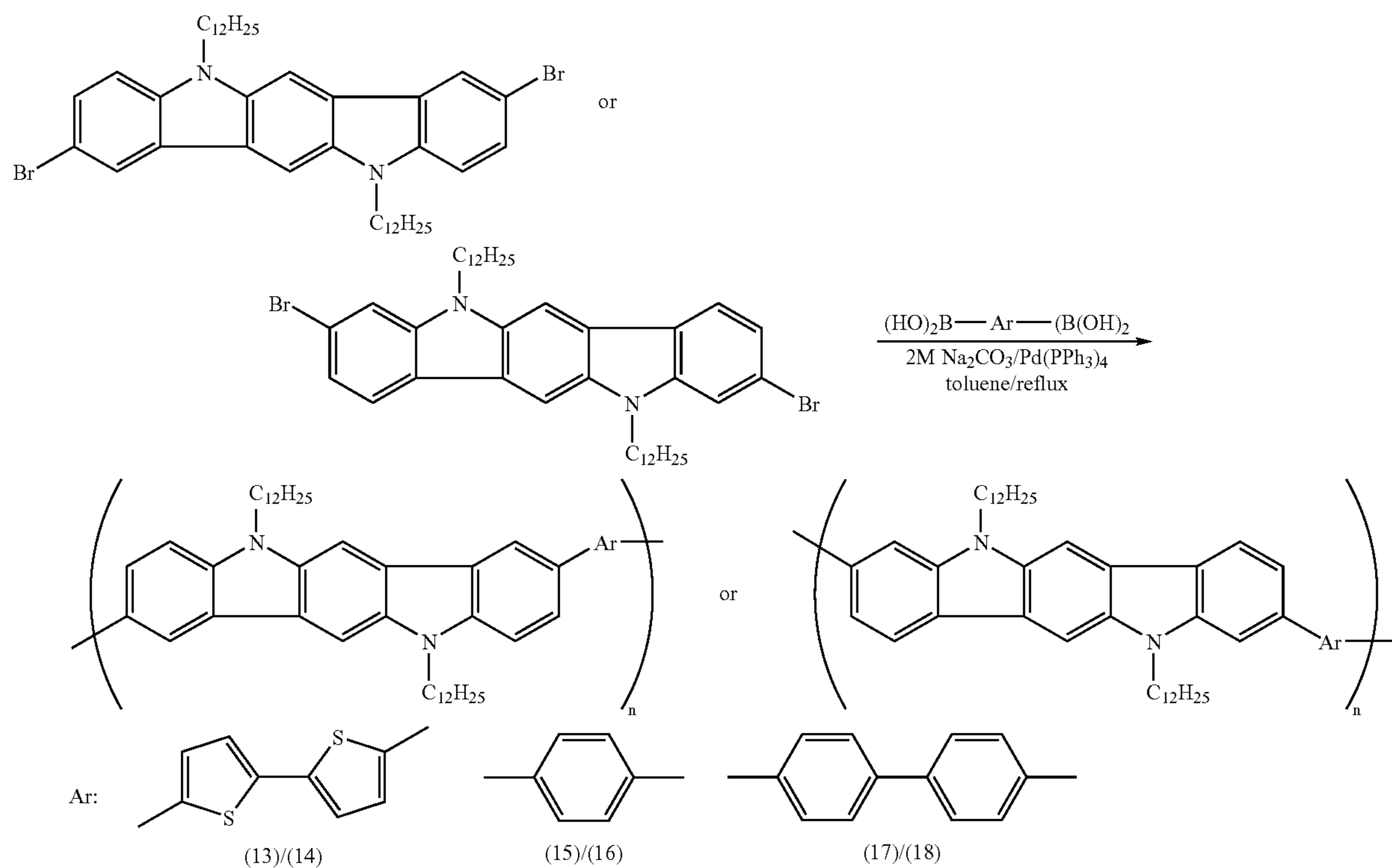
Scheme 2. Synthesis of polymer (13) through (18).
