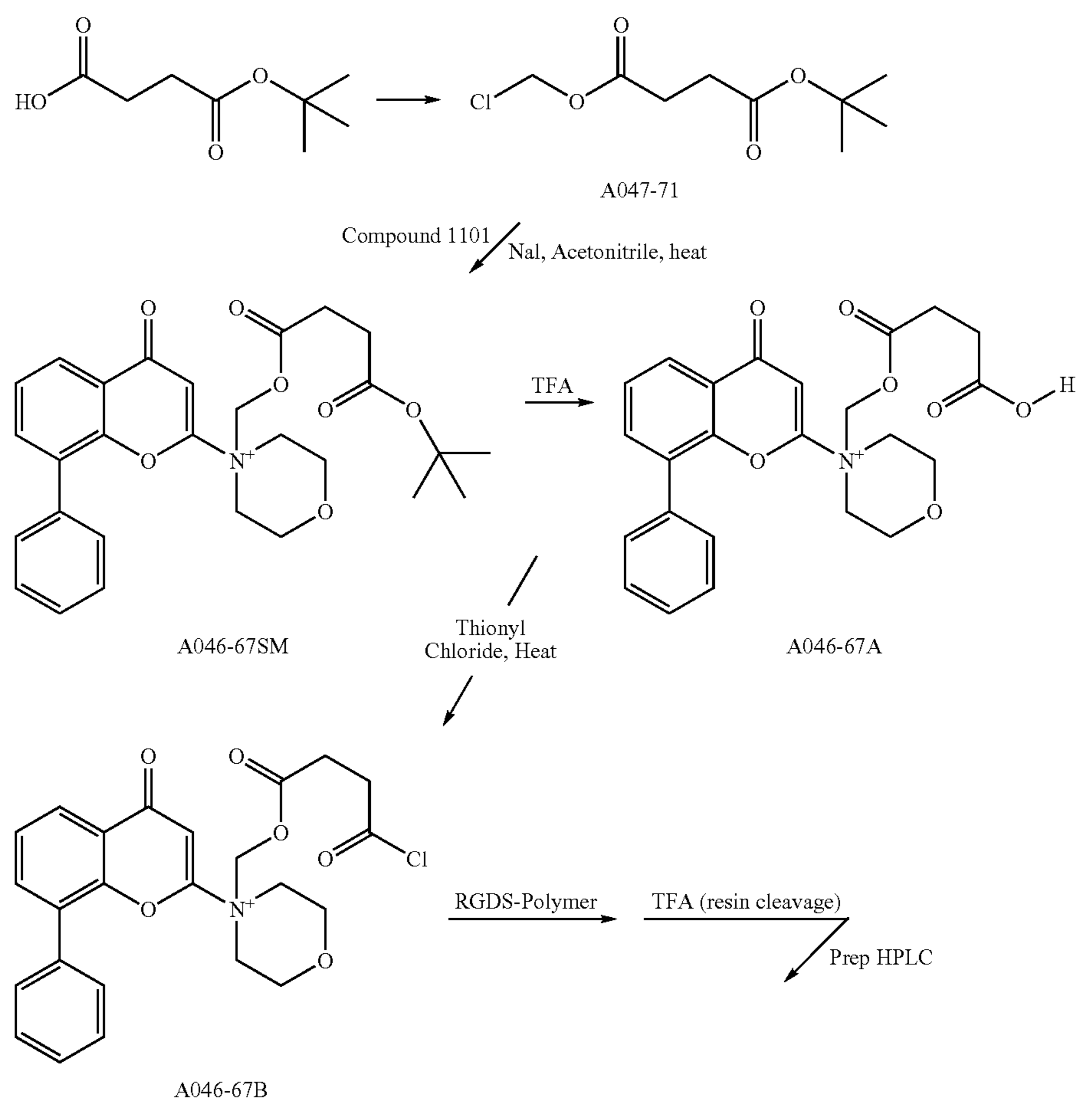
SCHEME 10
