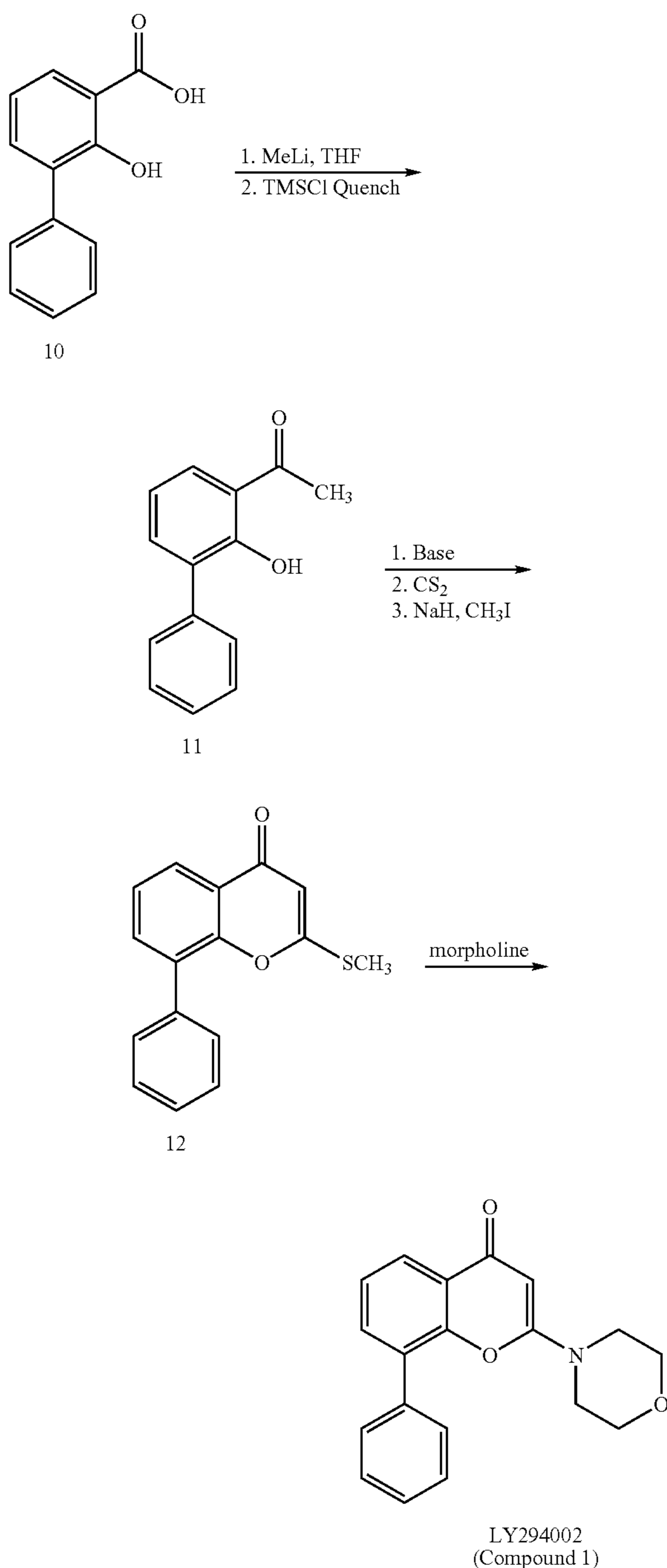
SCHEME 2
