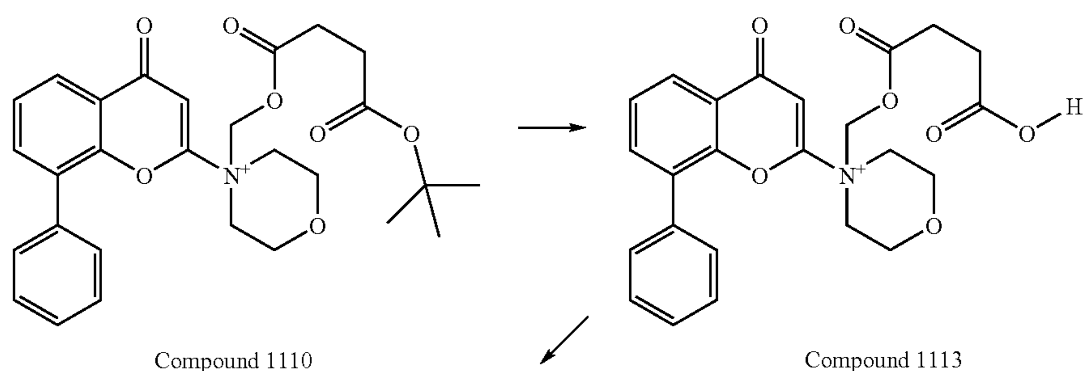
SCHEME 5
