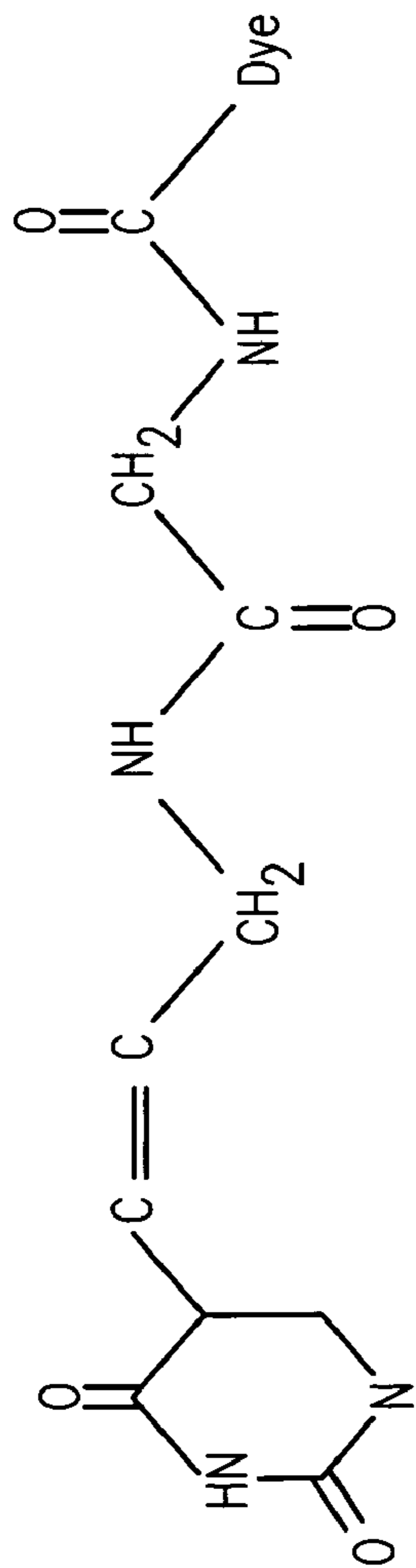
Diglycinylnyl linker
