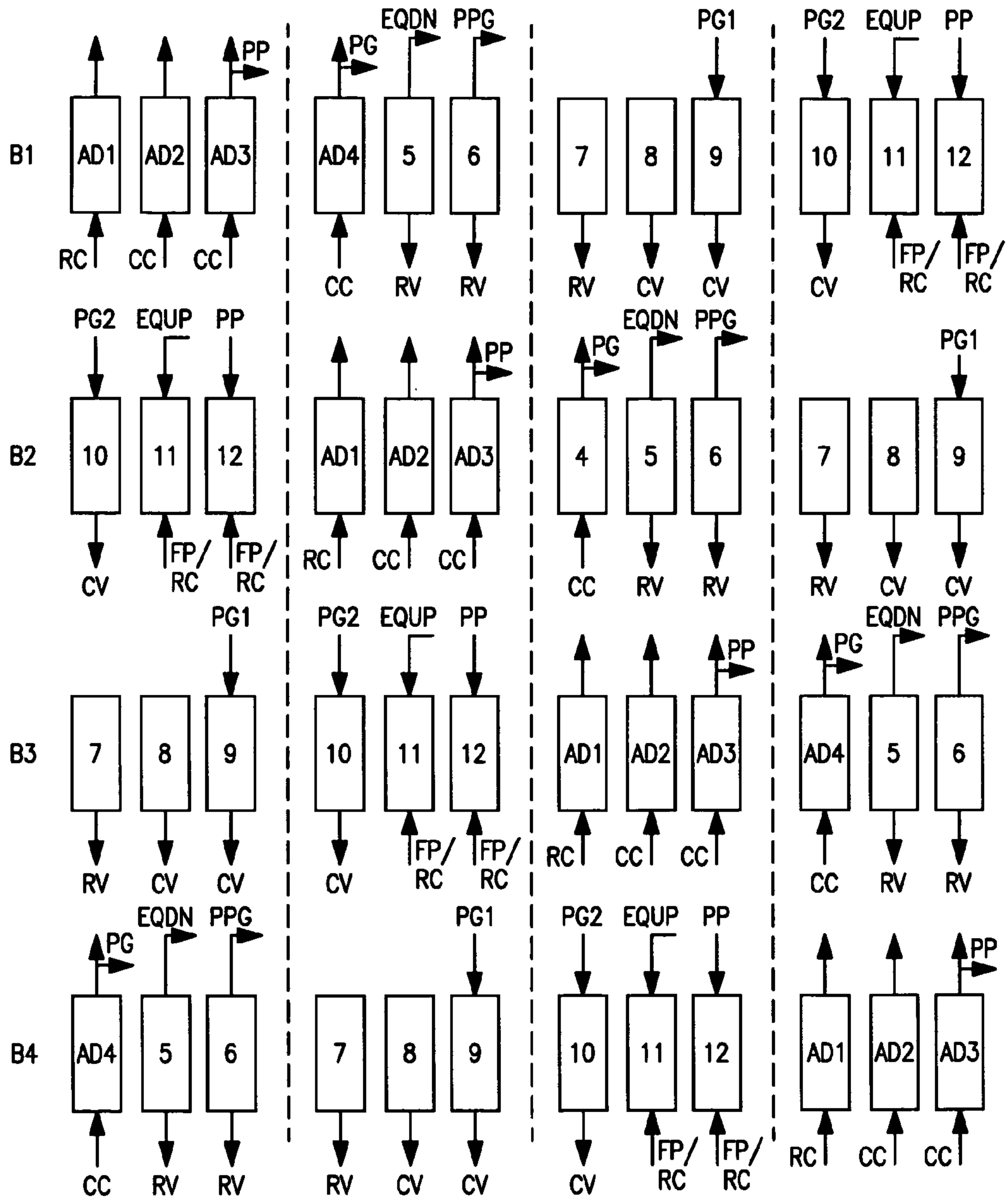
Four Bed VPSA Column Cycle Showing Two Beds Receiving Feed Gas Simultaneously.
