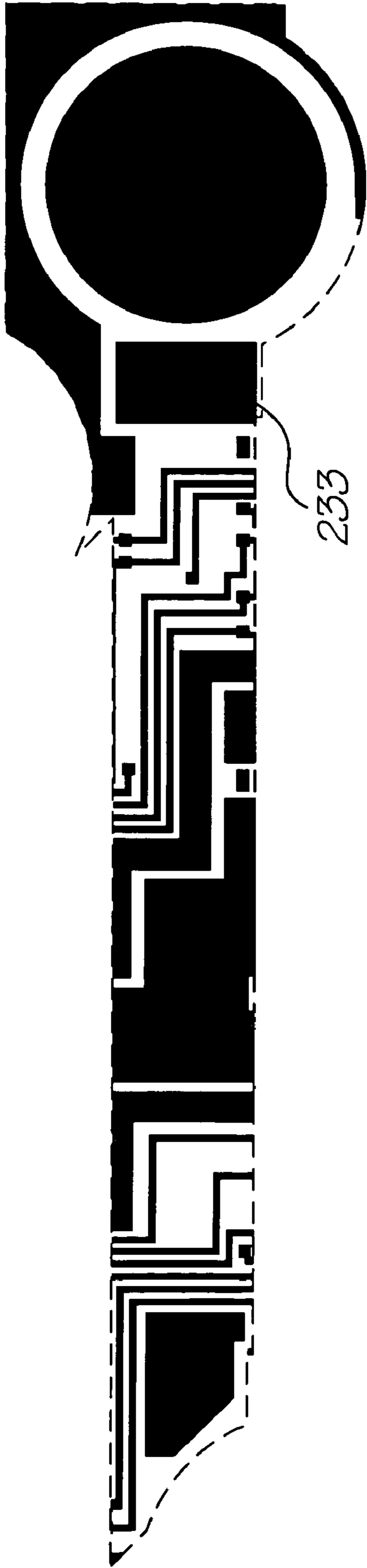
Metal 2 mask
