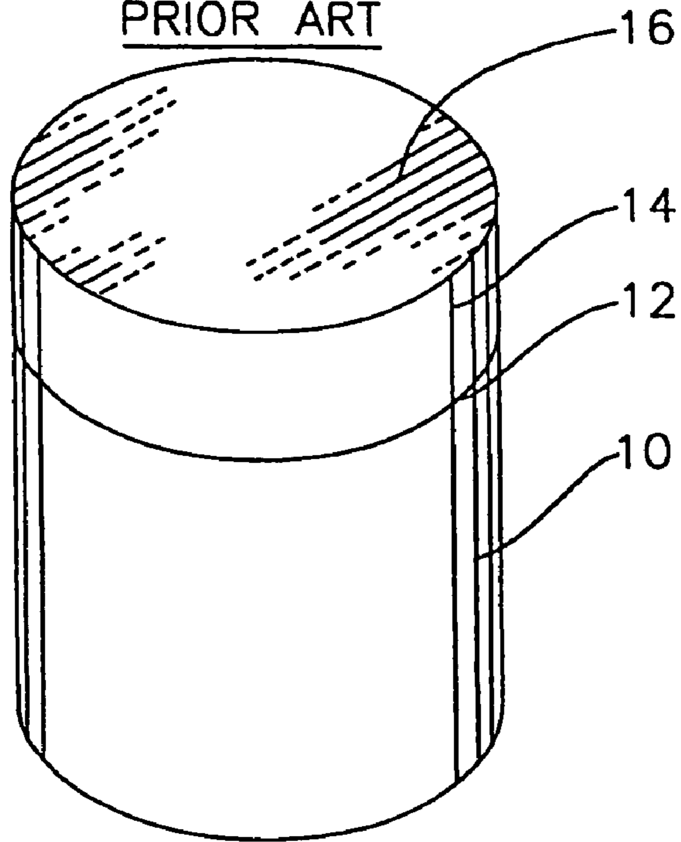
FIG. 3 PRIOR ART
