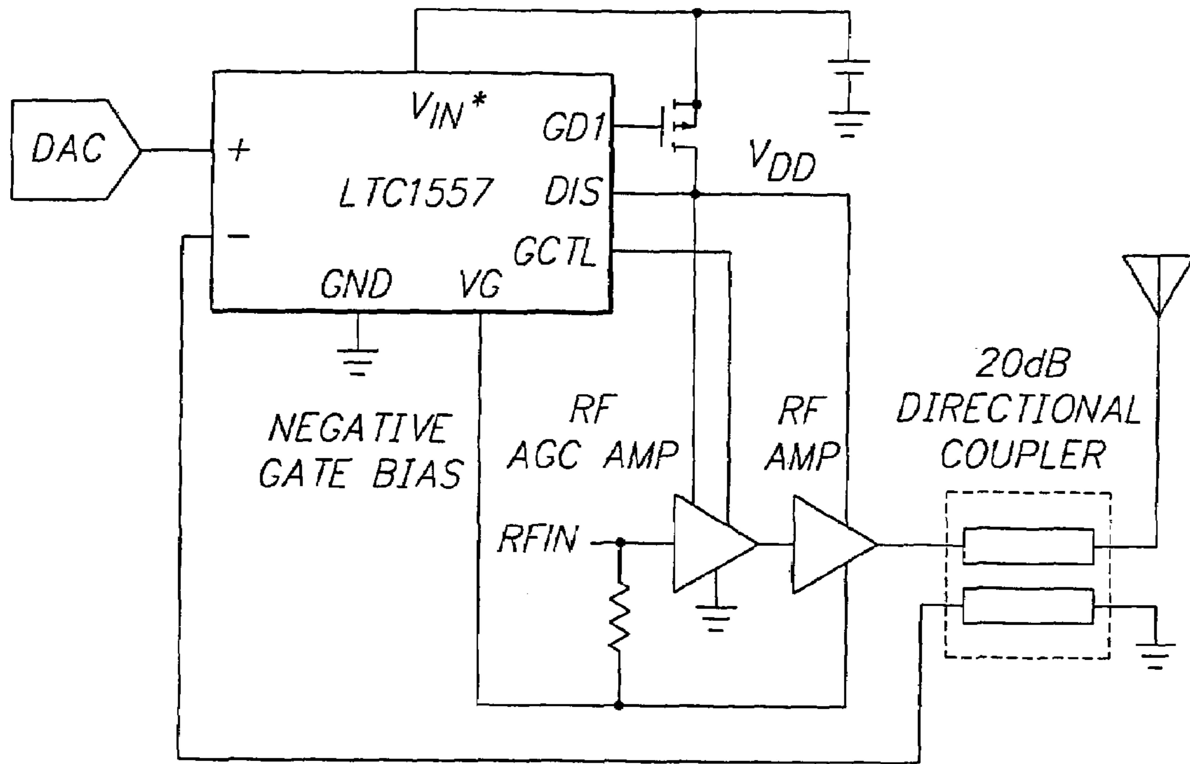
FIG. 1 (PRIOR ART)
