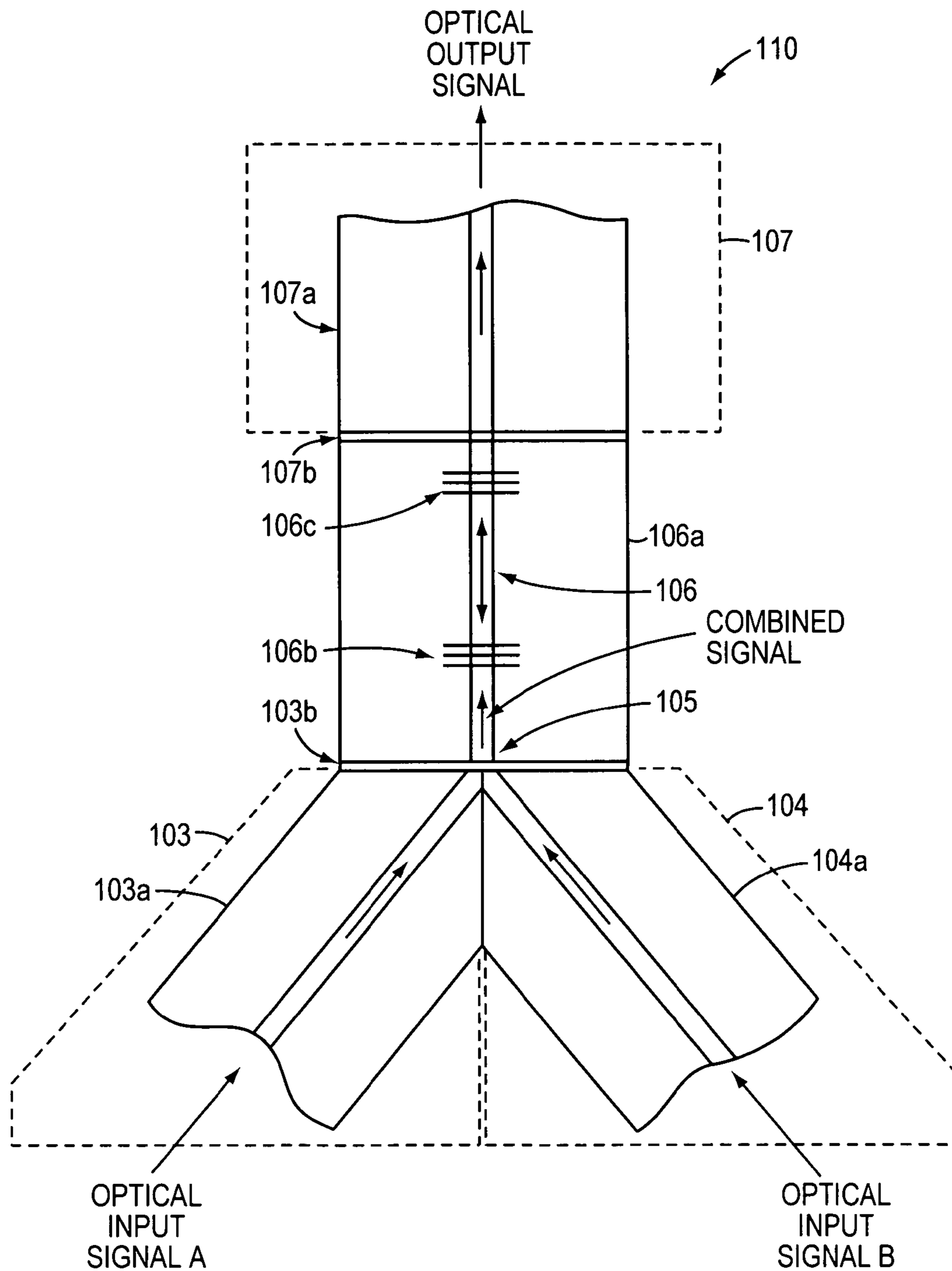
ALL-OPTICAL LOGICAL GATE IMPLEMENTED WITH OPTICAL FIBERS
