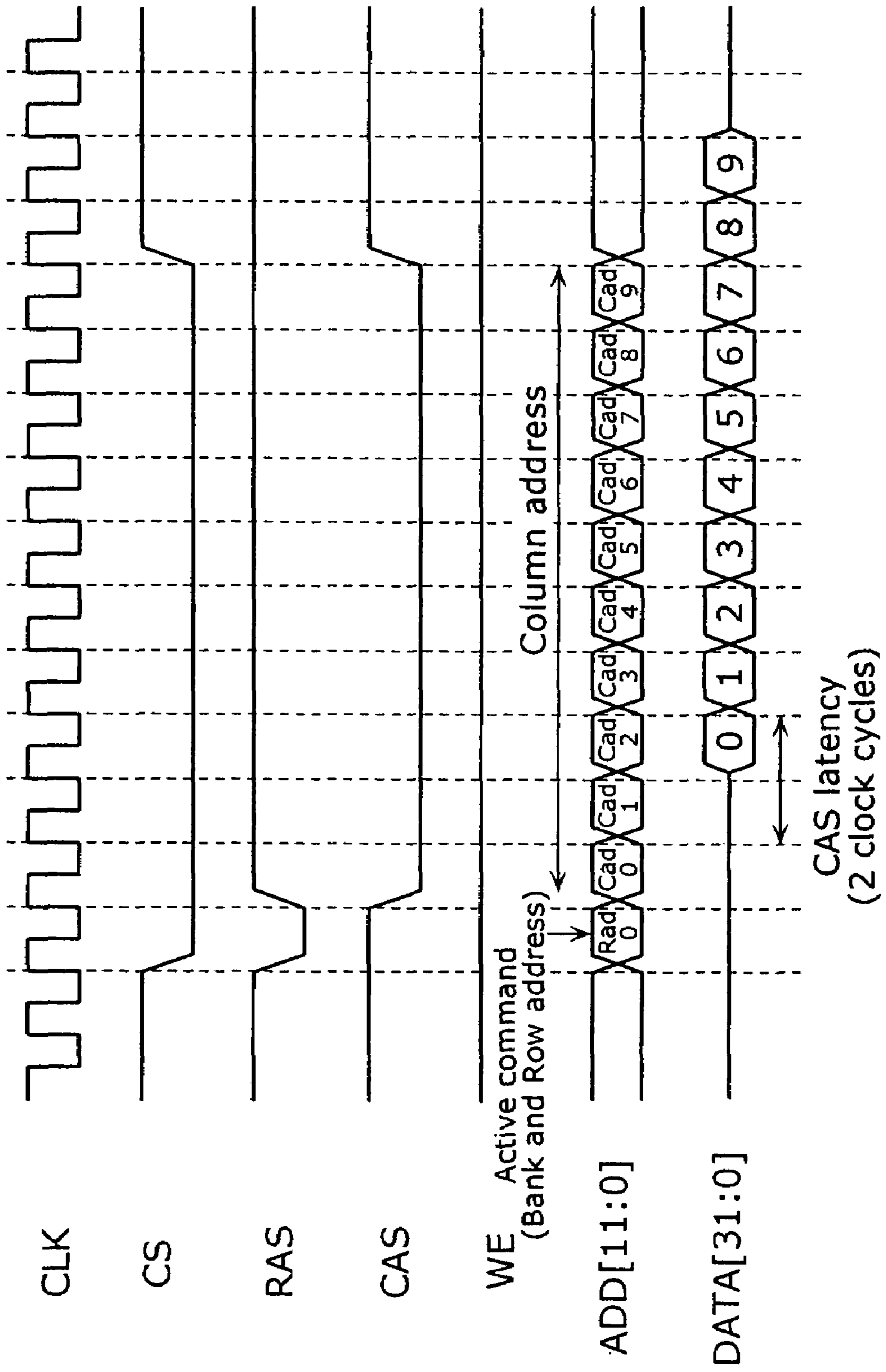
FIG. 6 Prior Art
