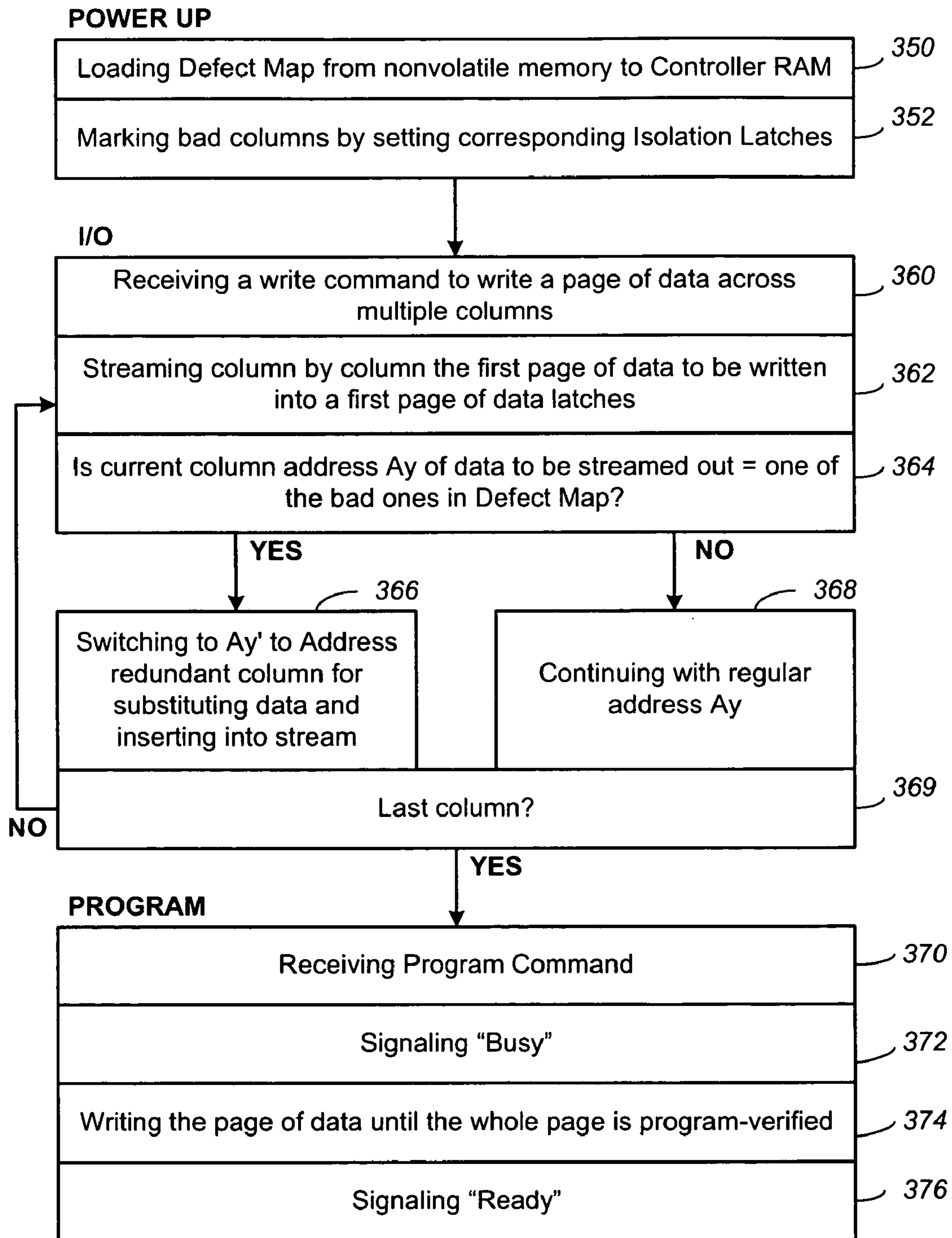
PROGRAM OPERATION (Prior Art)
