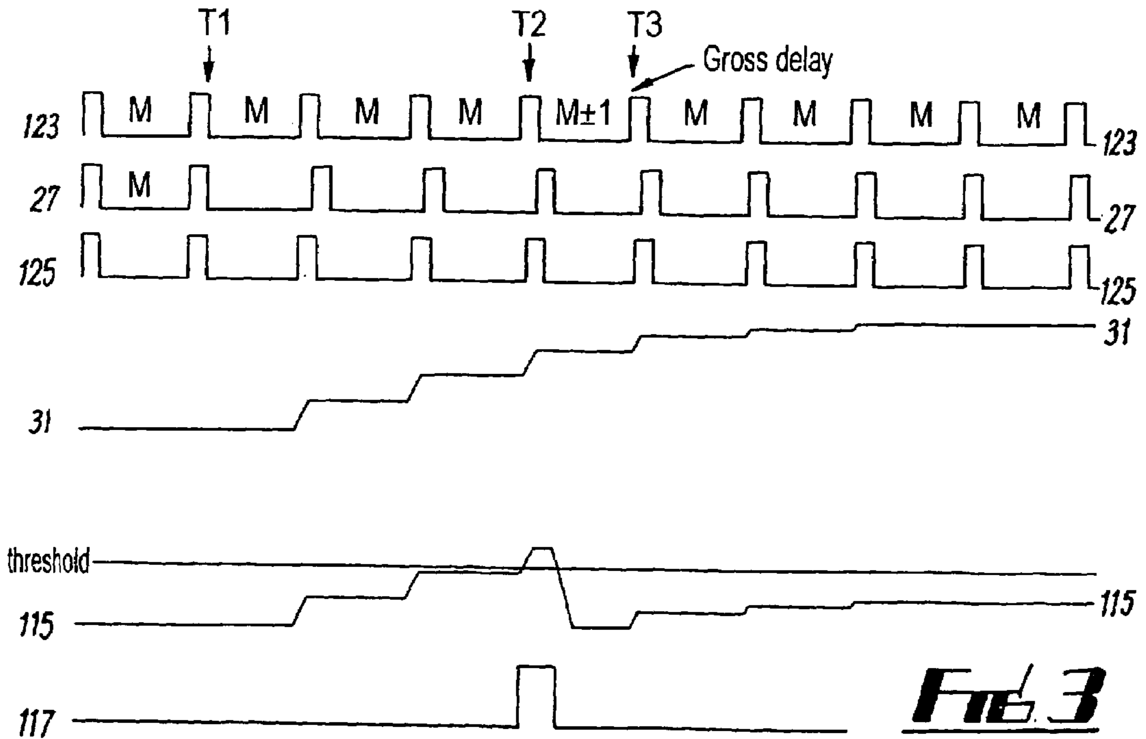
Signal timing diagram
