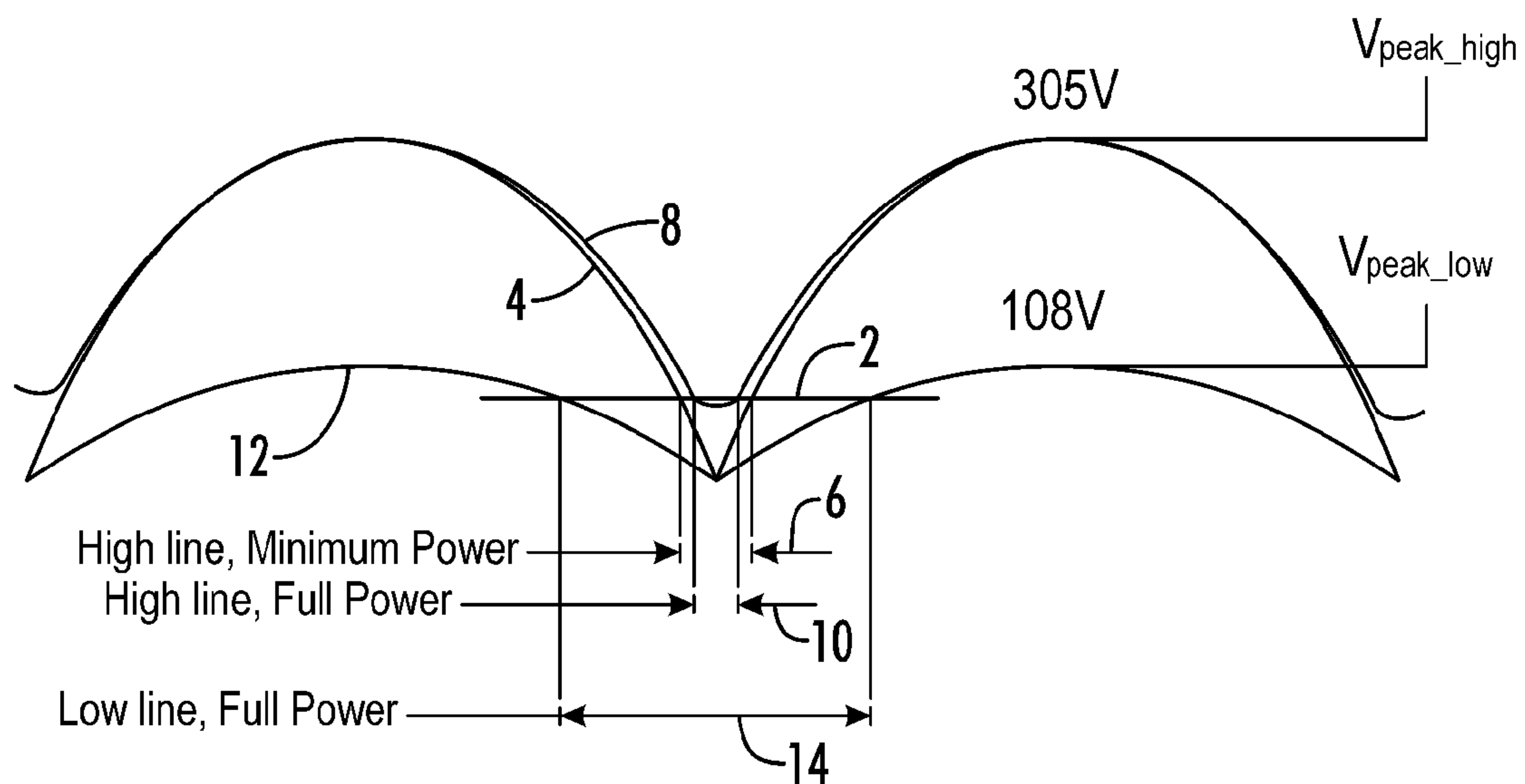
FIG. 1 (PRIOR ART)
