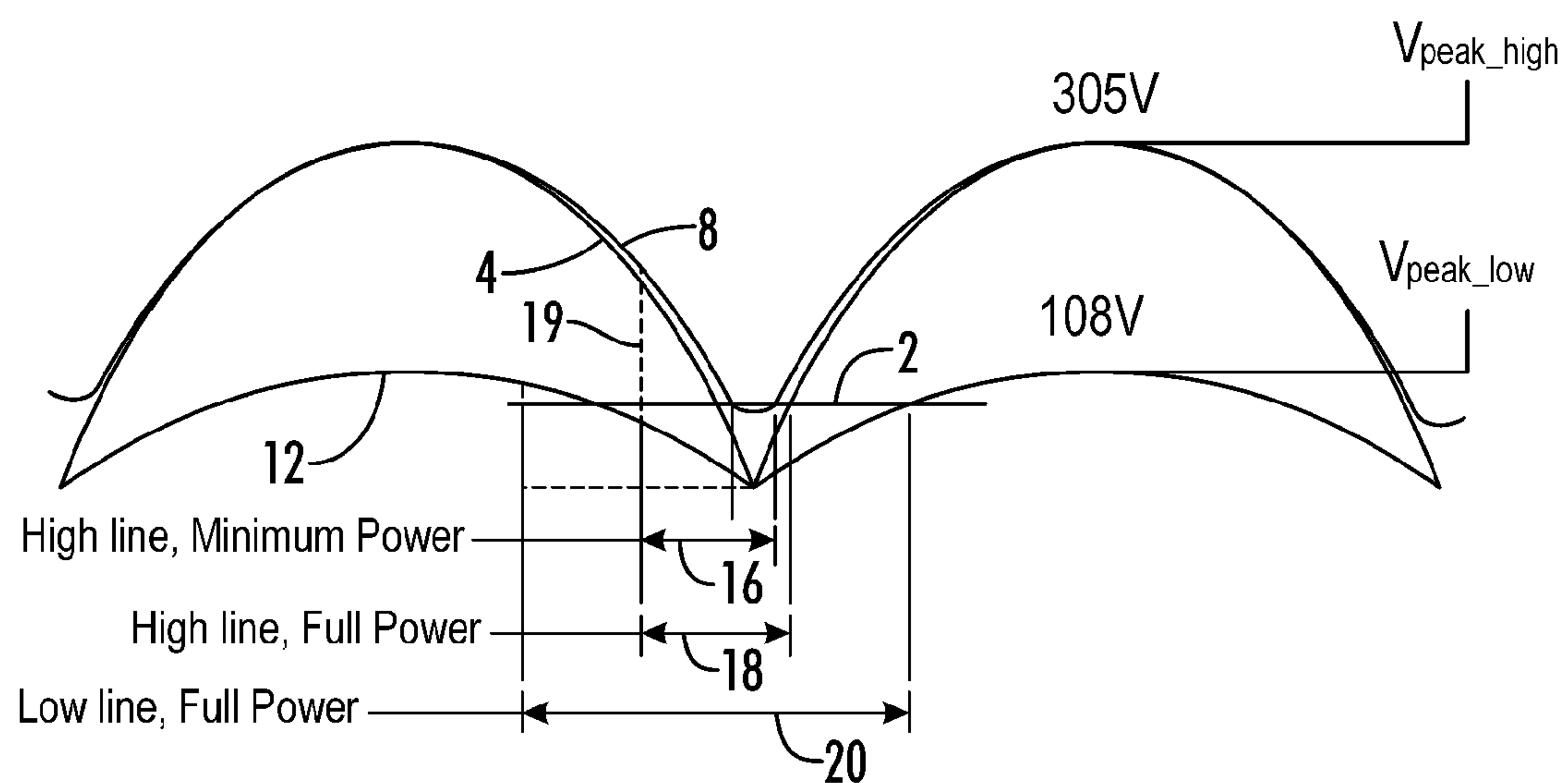
FIG. 2 (PRIOR ART)
