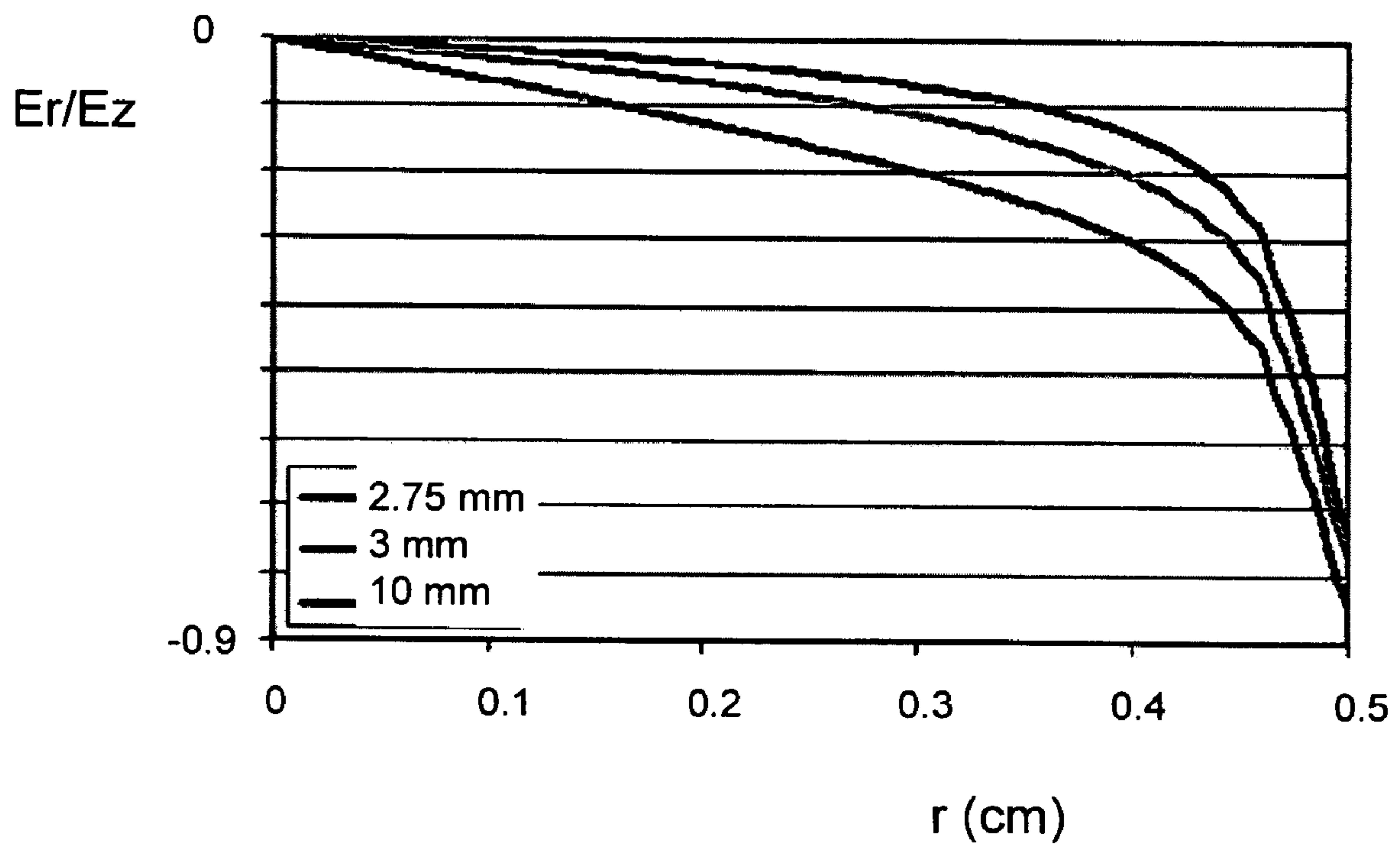
NORMALIZED FOCUSING FIELD AT CATHODE SURFACE
