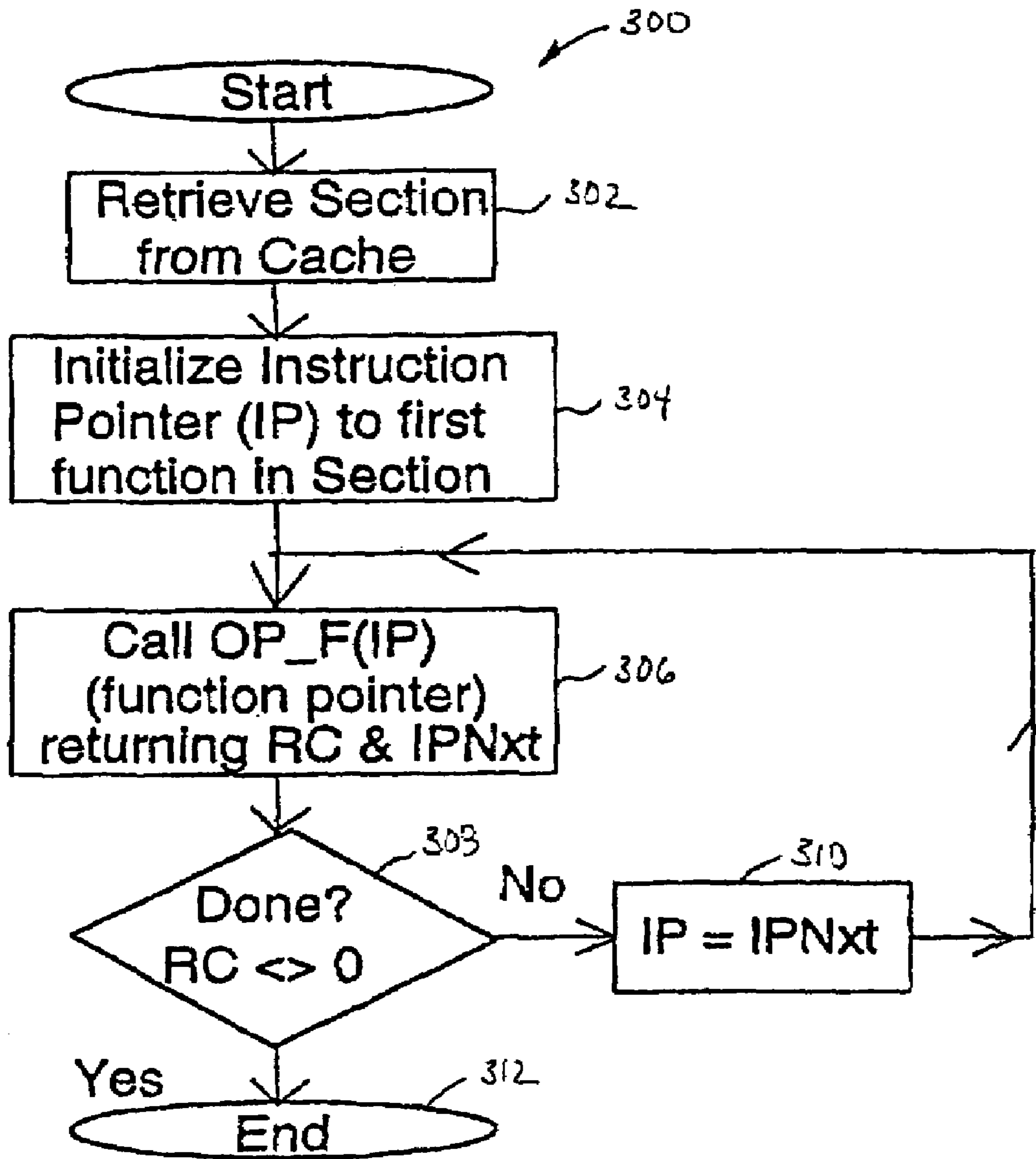
New implementation of Section Execution
