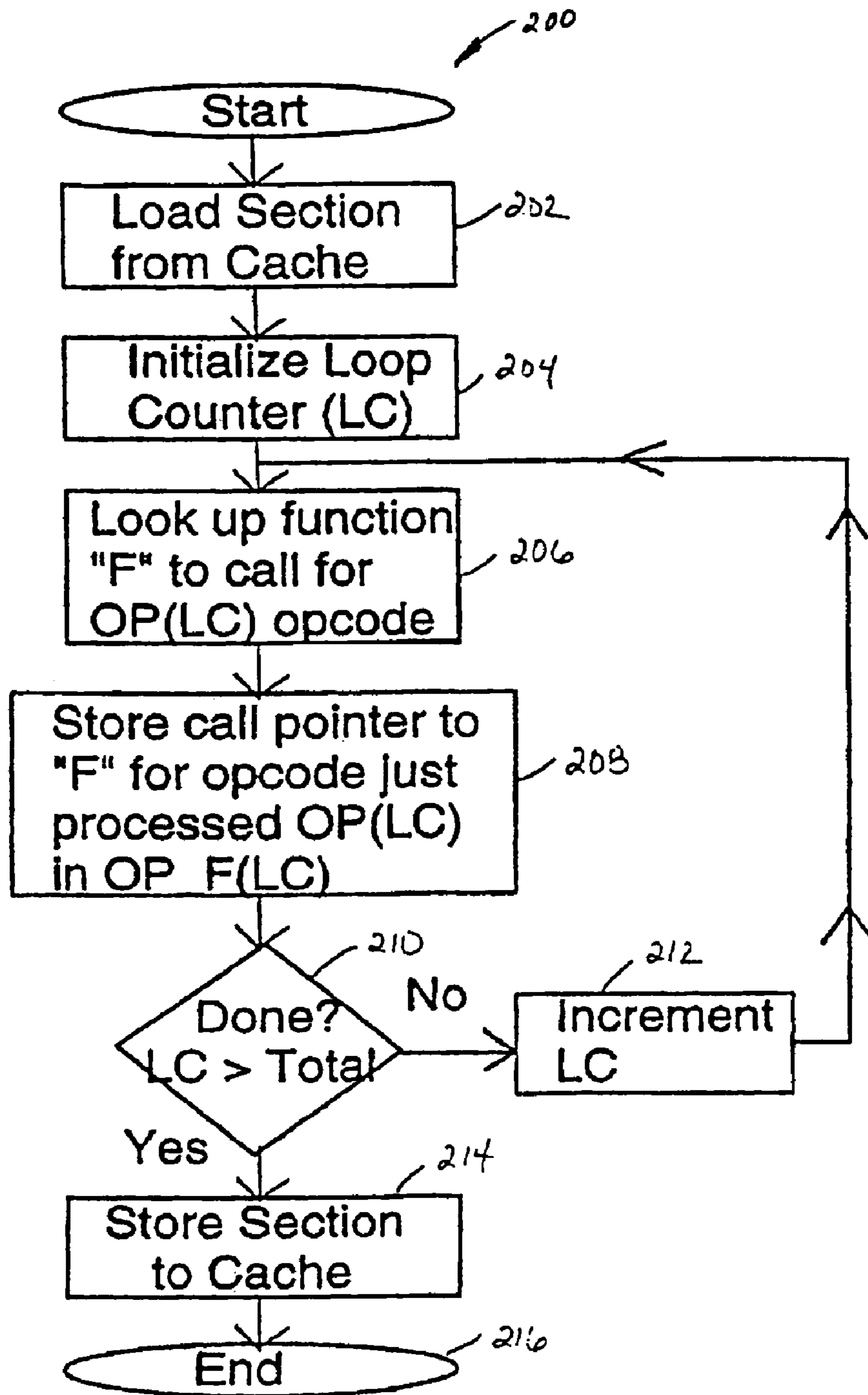
Translation of Opcode to Function Pointer
