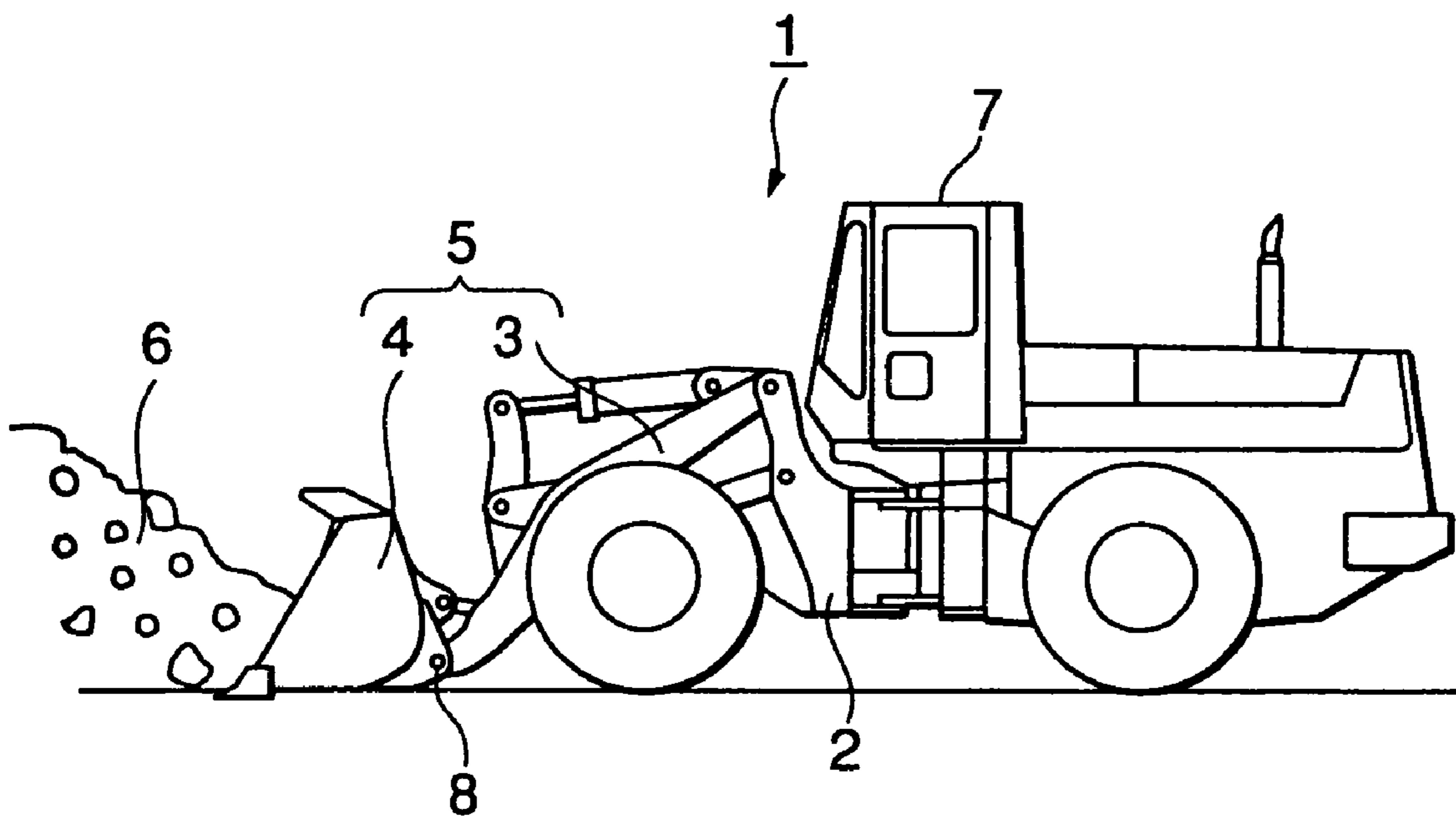
FIG.10 PRIOR ART
