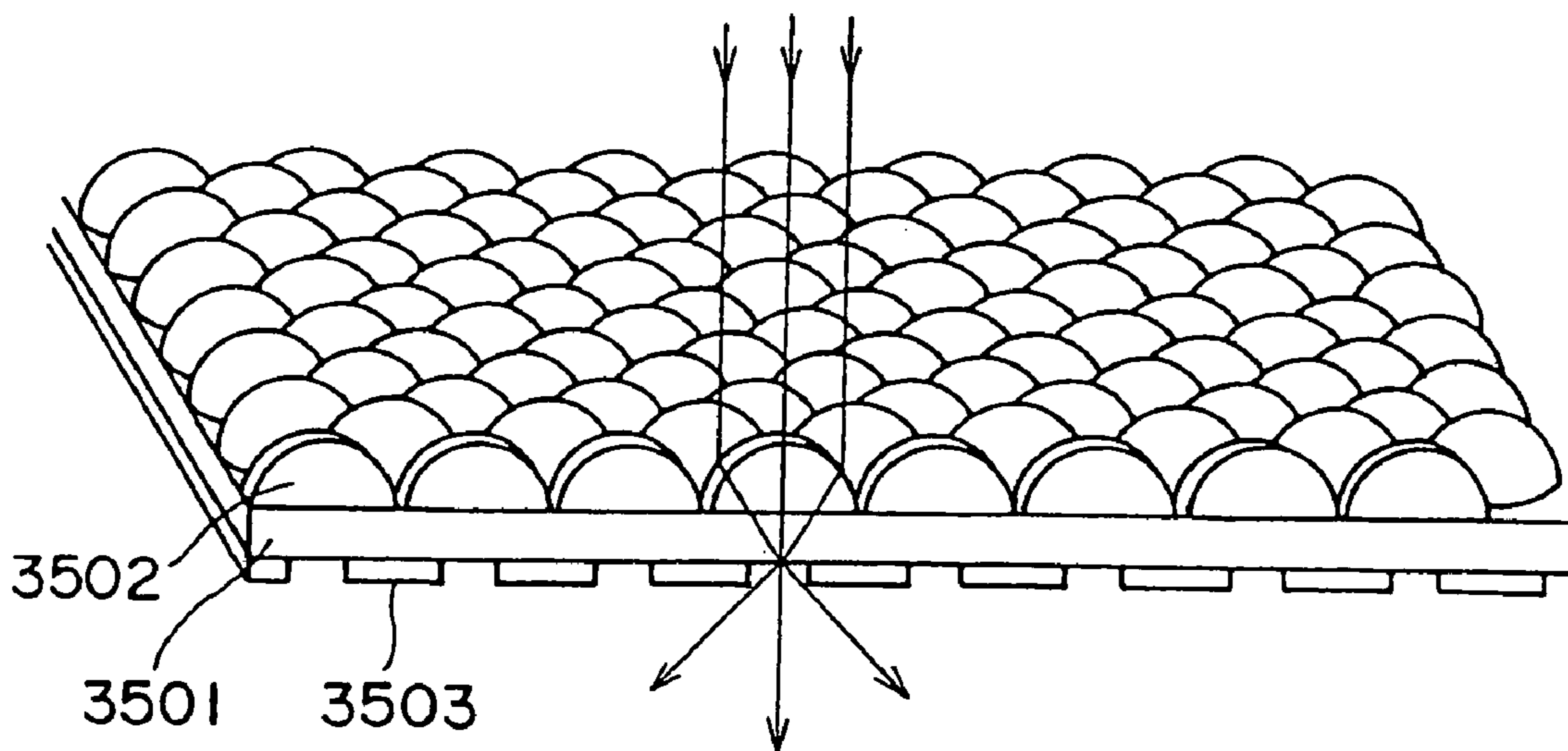
3501: TRANSPARENT BASE MEMBER 3502: MICRO-LENS 3503: LIGHT ABSORBING LAYER
