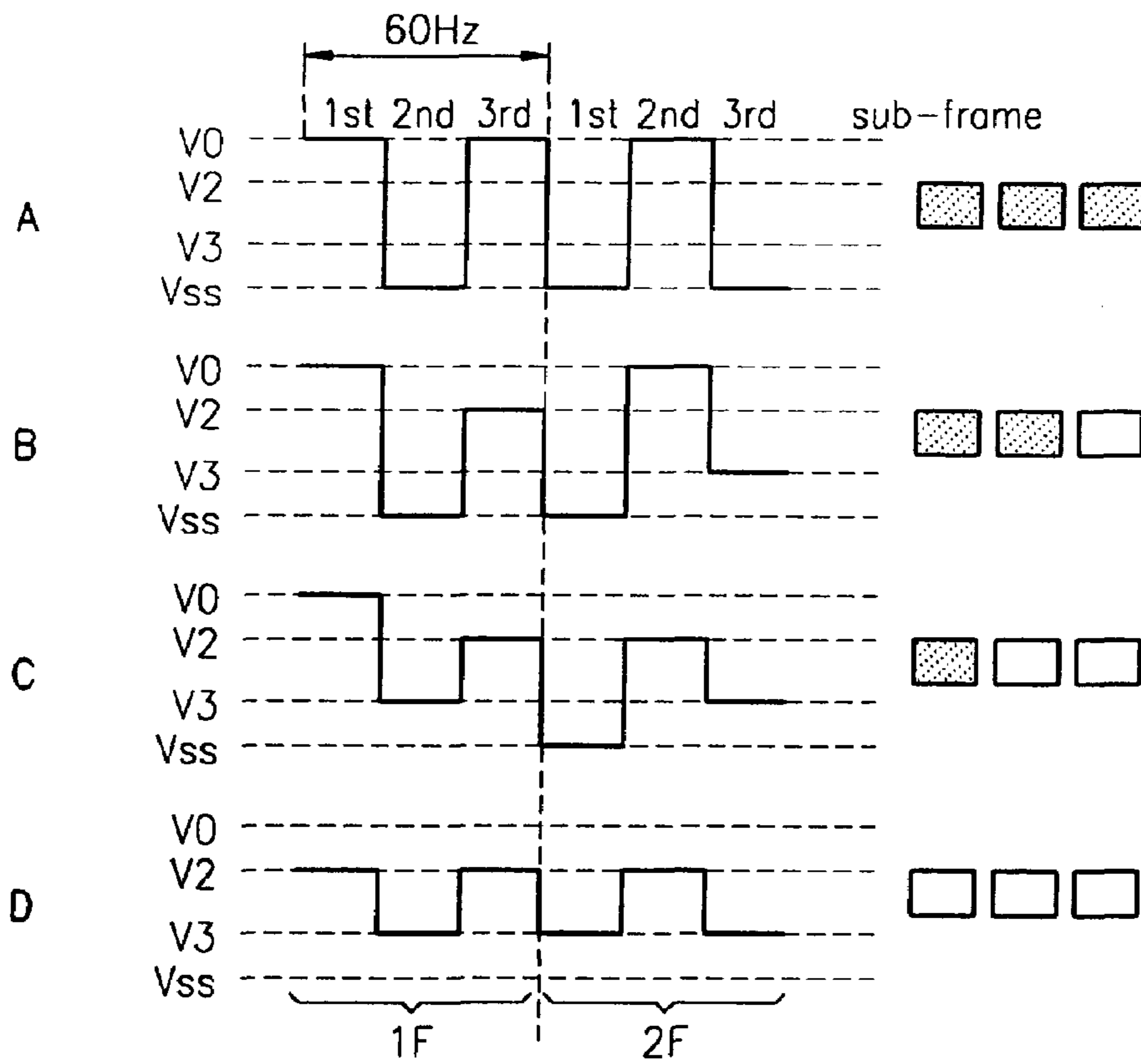
FIG. 2 (PRIOR ART)
