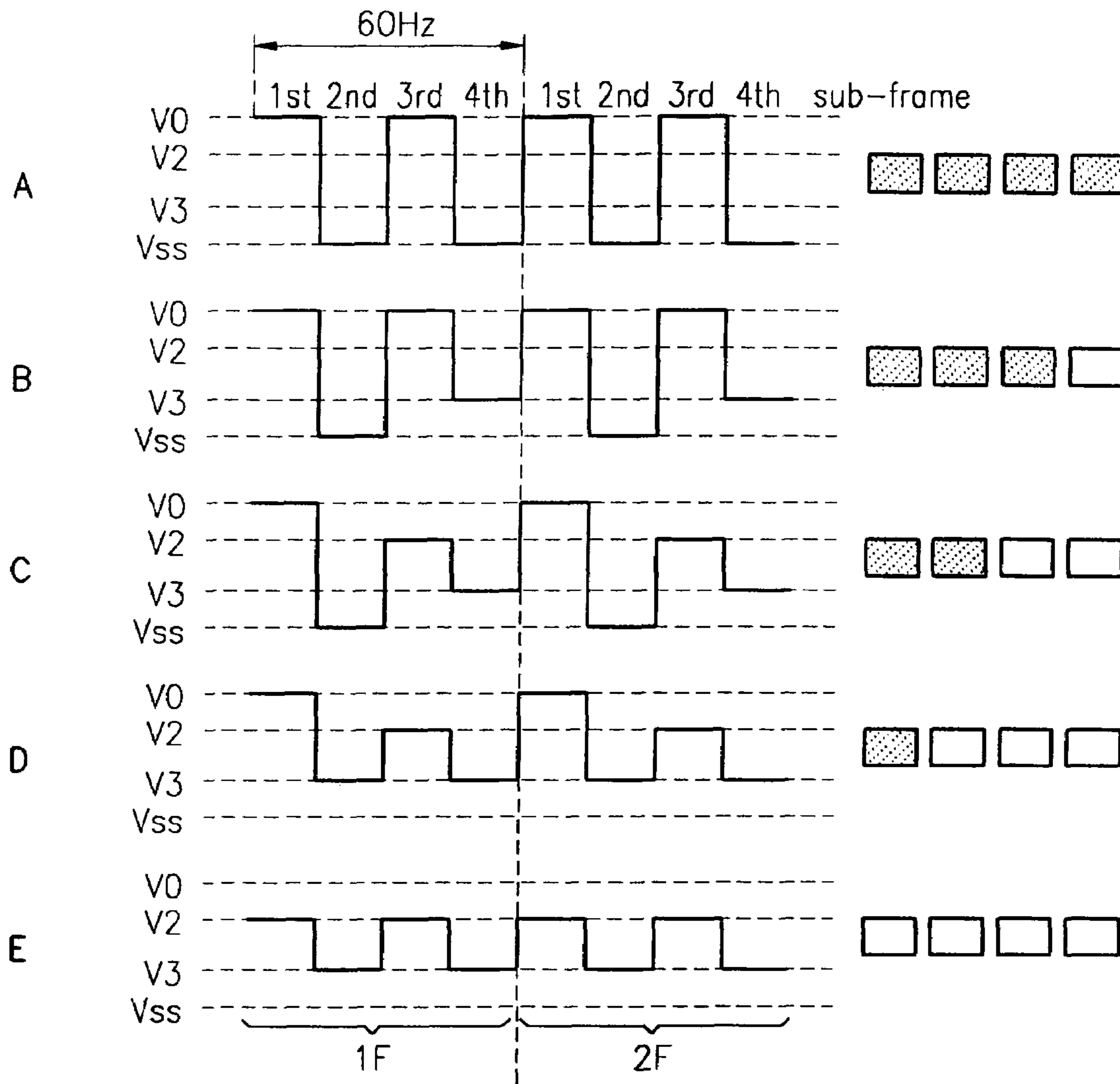
FIG. 3 (PRIOR ART)
