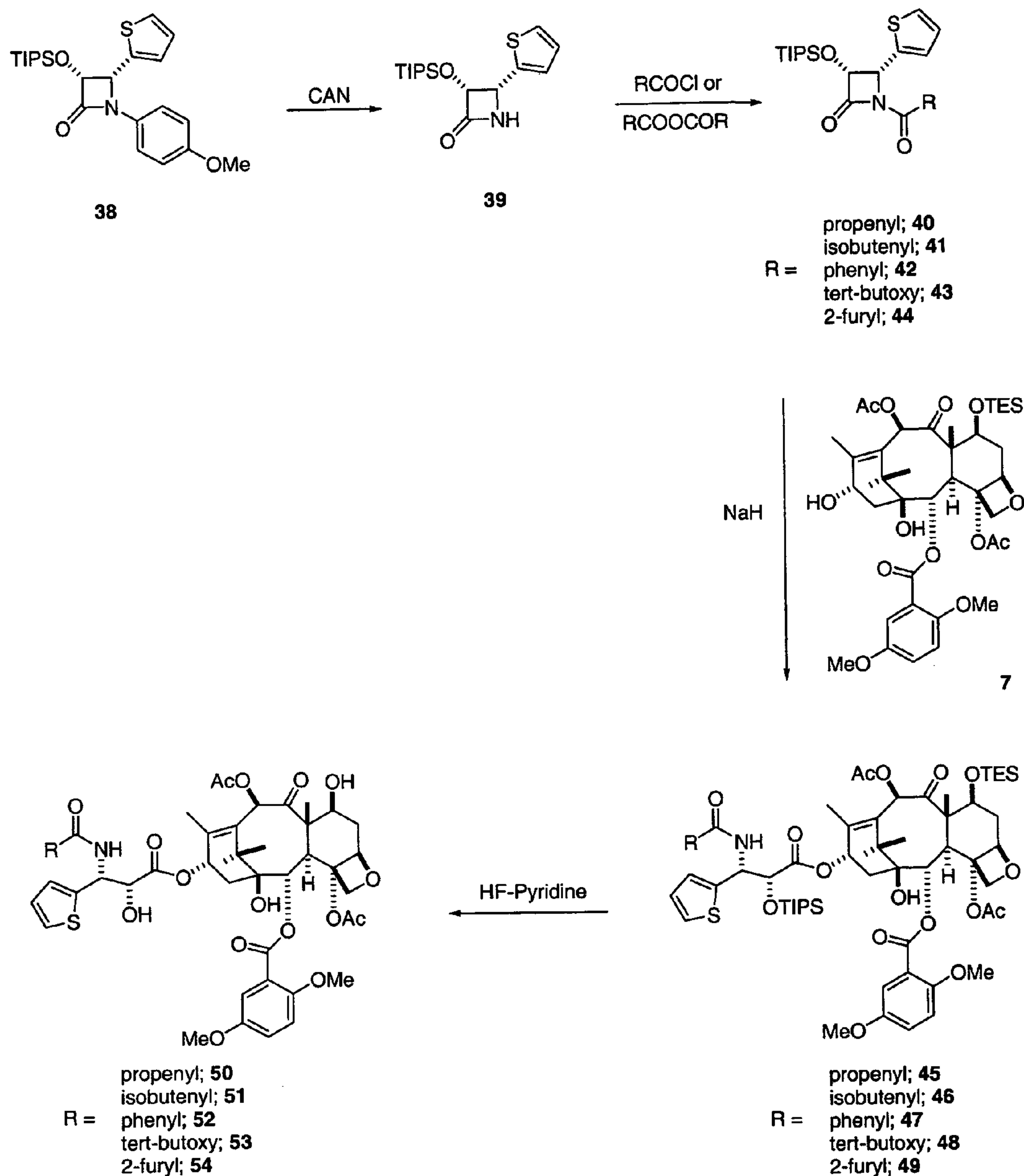
Figure 16c Synthesis of New Taxanes
