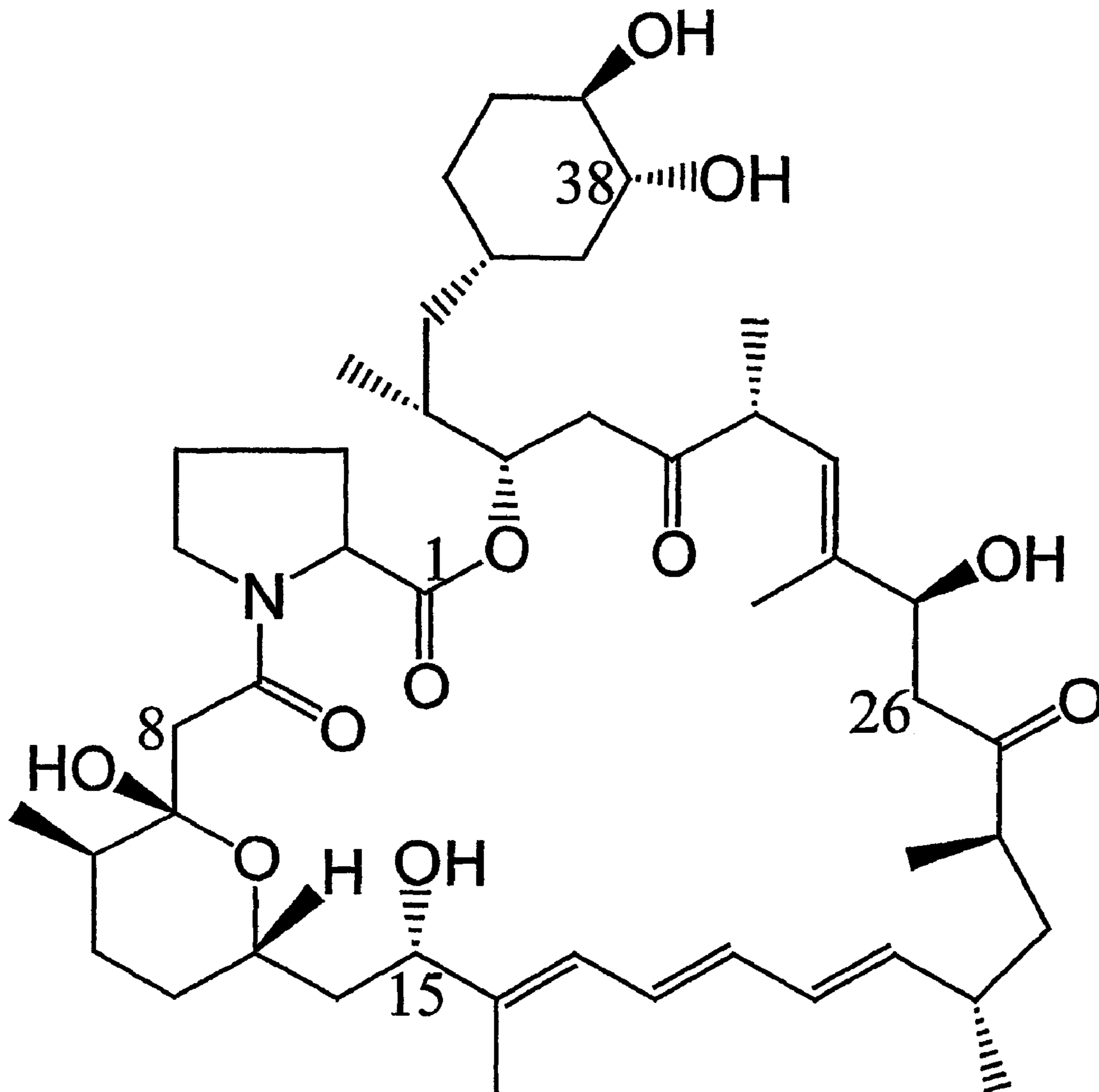
8-deoxy-15-O-desmethyl-26-desmethoxy-38-O-desmethyl prolylrampamycin
