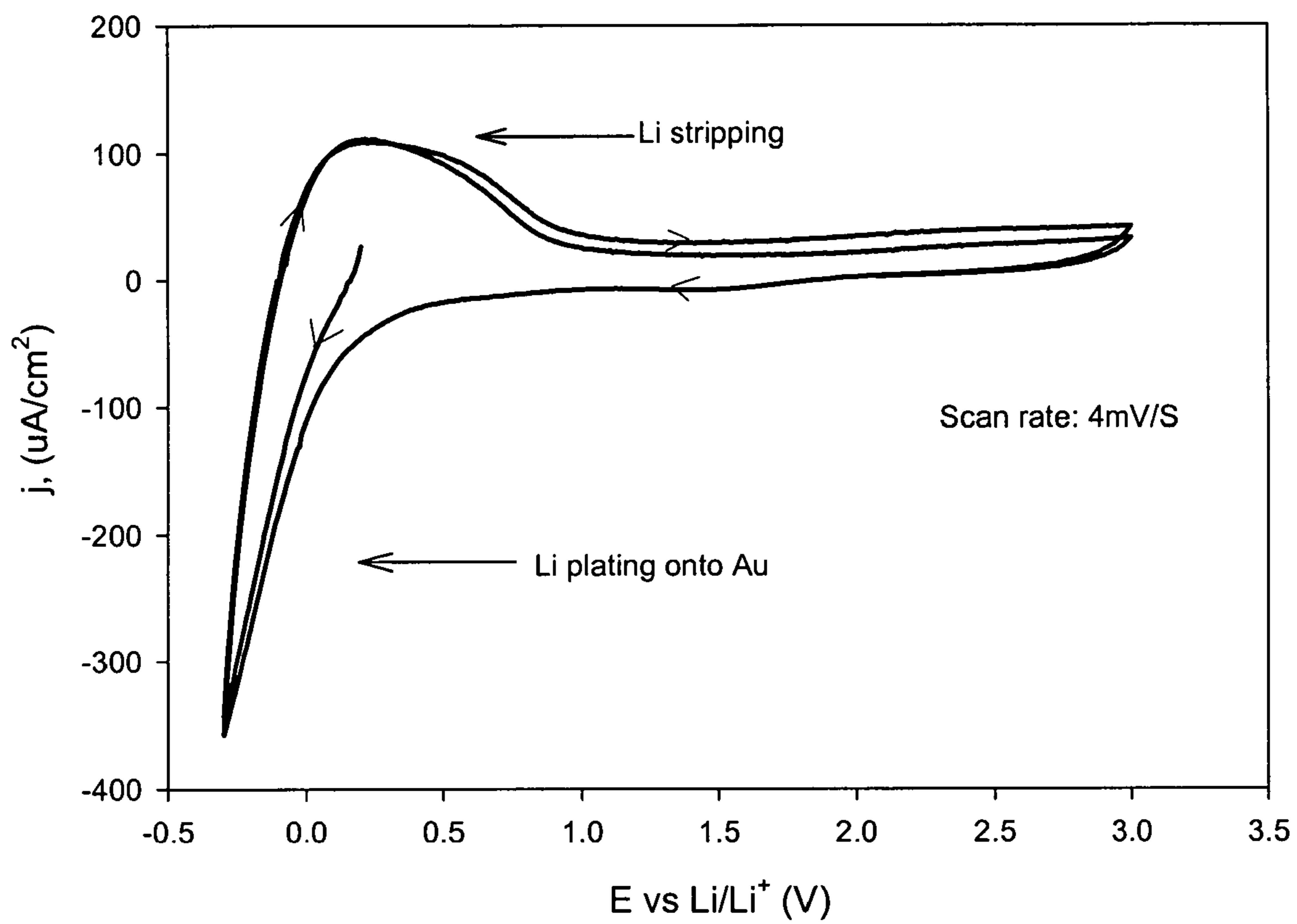
Cyclic Voltammetry for Solid State Cell: Li | Cu 3 N | OHARA plate | Au
