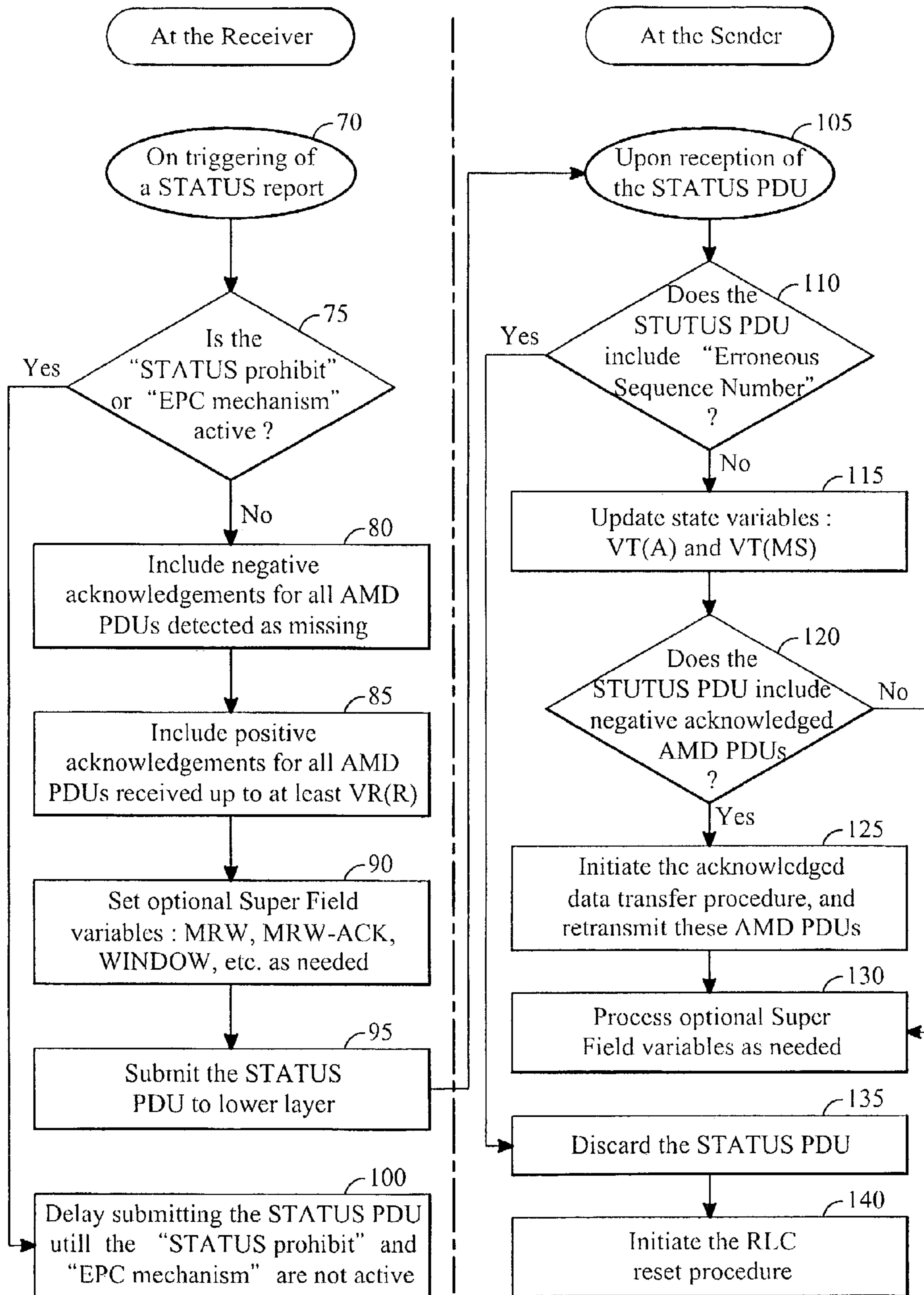
FIGURE 4 (Prior Art)
