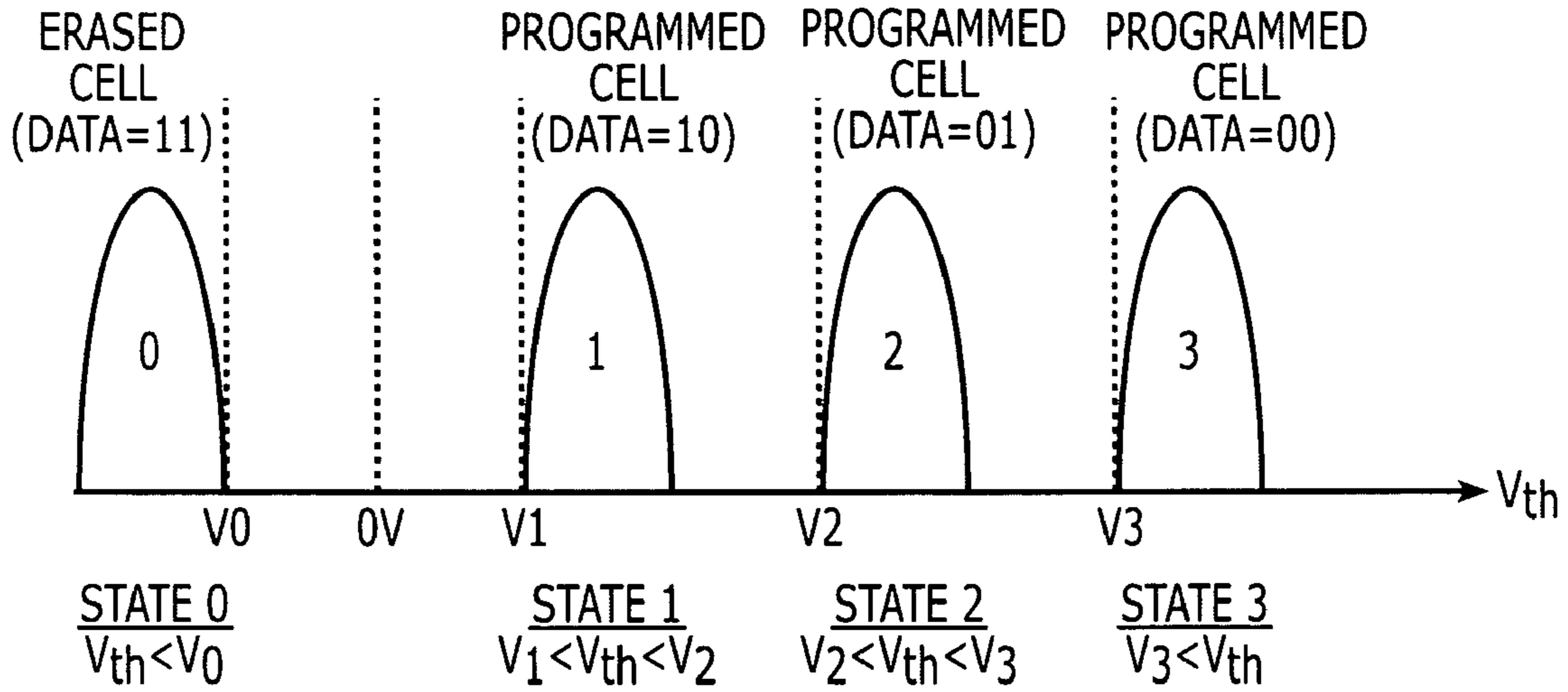
FIG. 2 (PRIOR ART)
