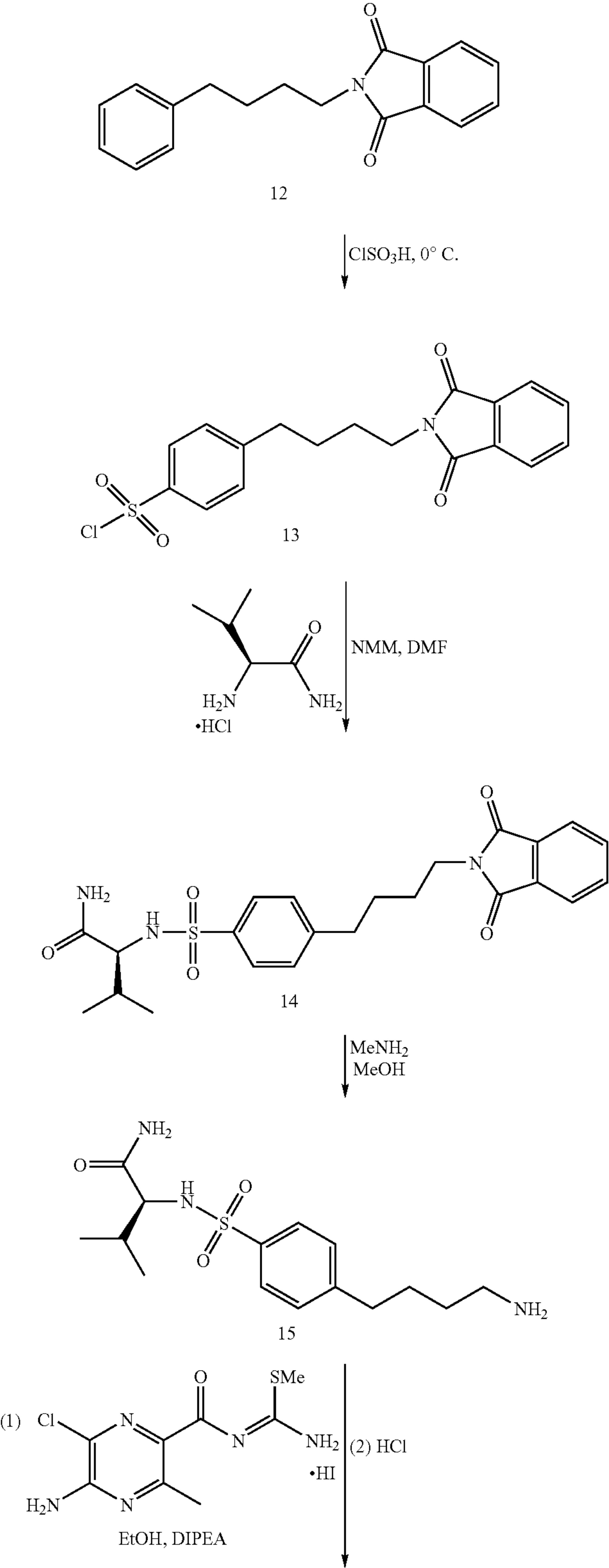
Scheme 3. Synthese of PSA 19008
