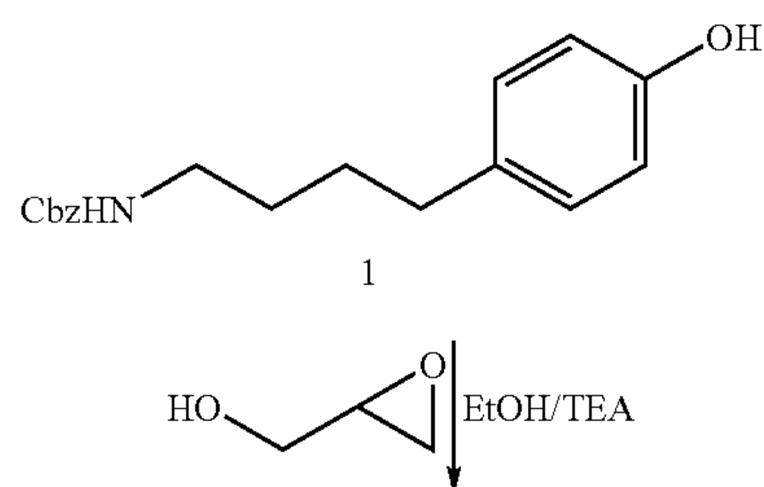
Scheme 11. Synthesis of PSA 15143
