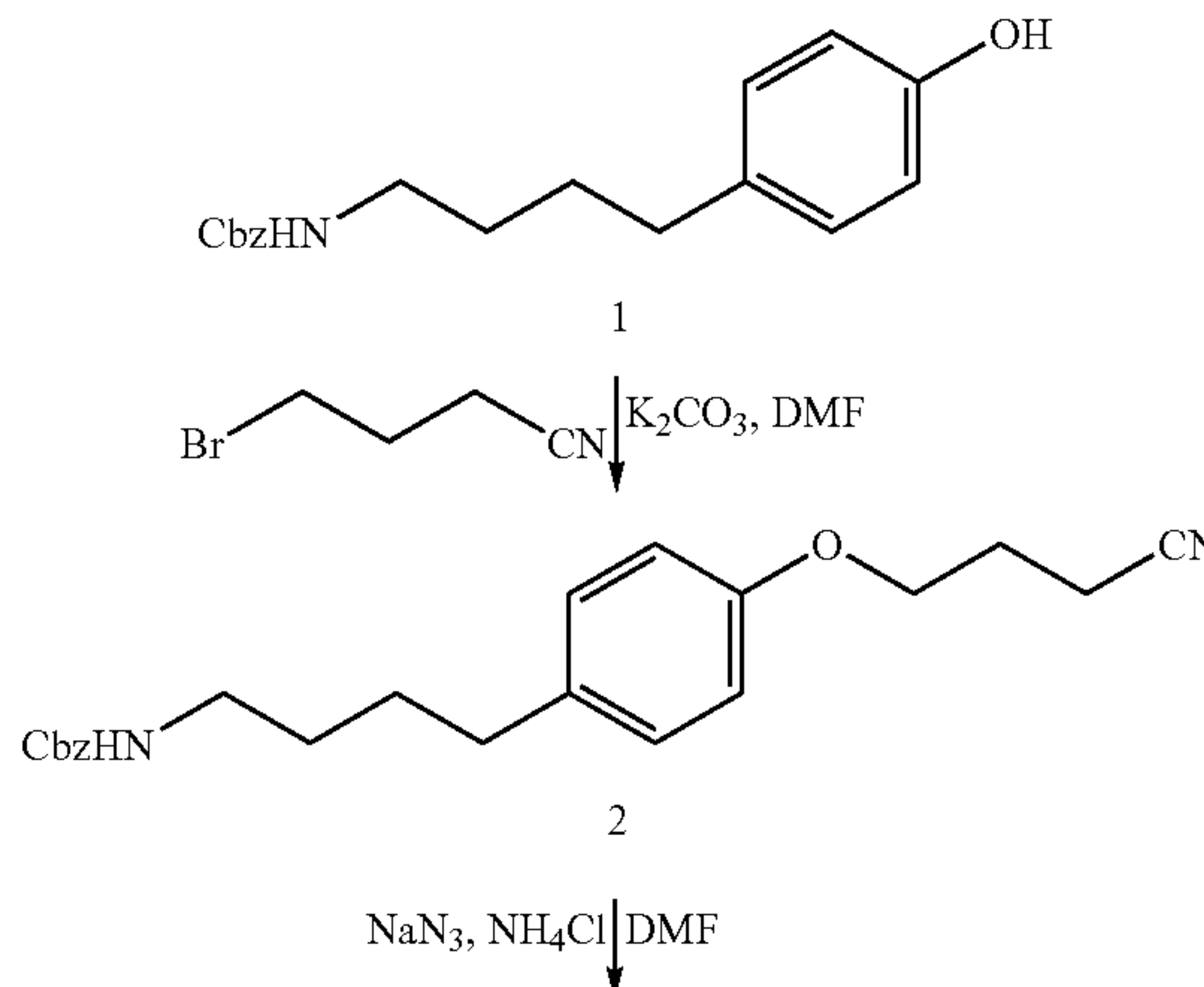
Scheme 1. Synthesis of PSA 17926
