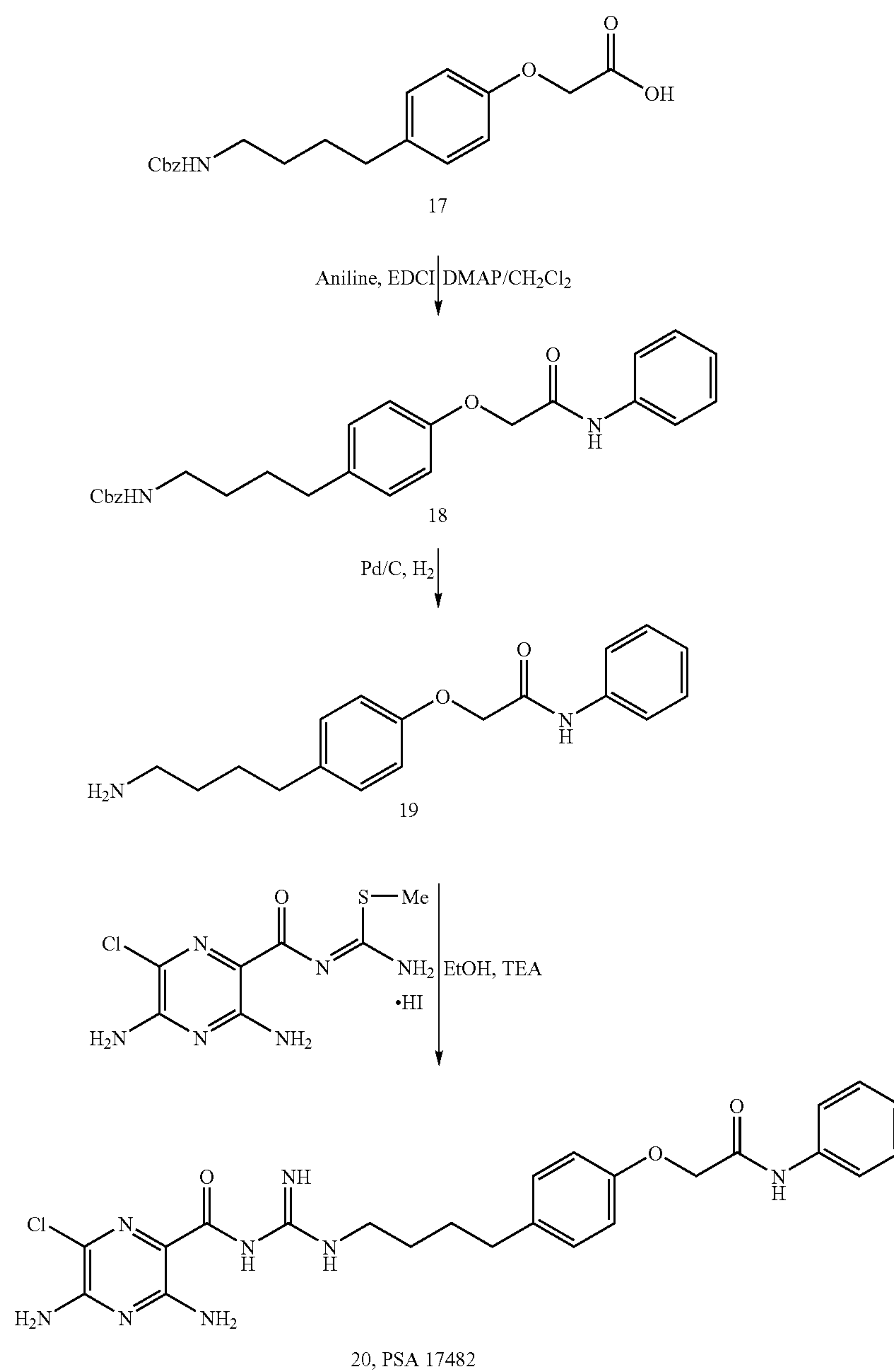
Scheme 4. Synthesis of PSA 17482
