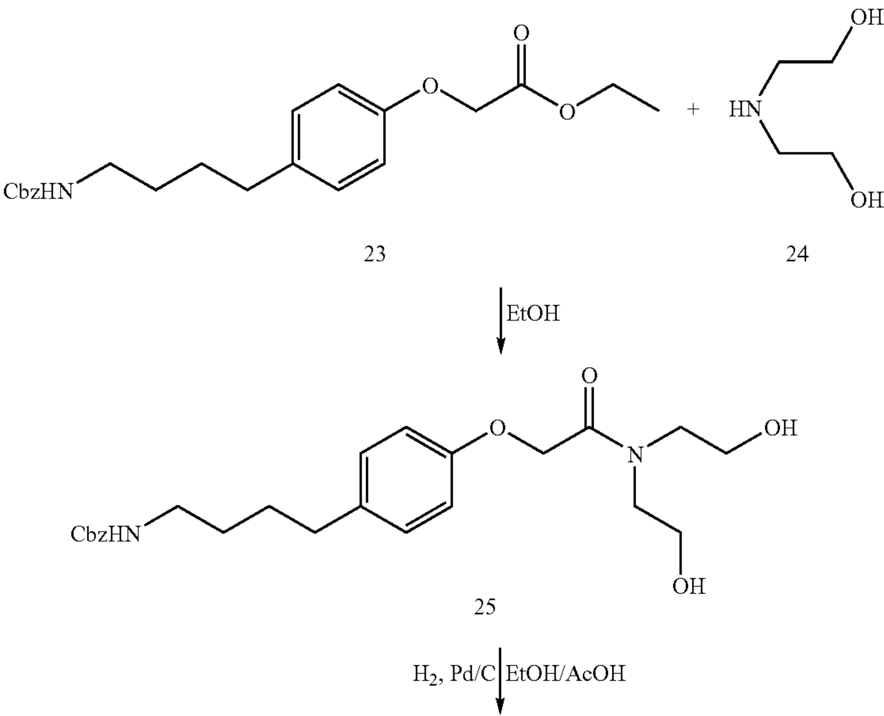
Scheme 6. Synthesis of PSA 16826
