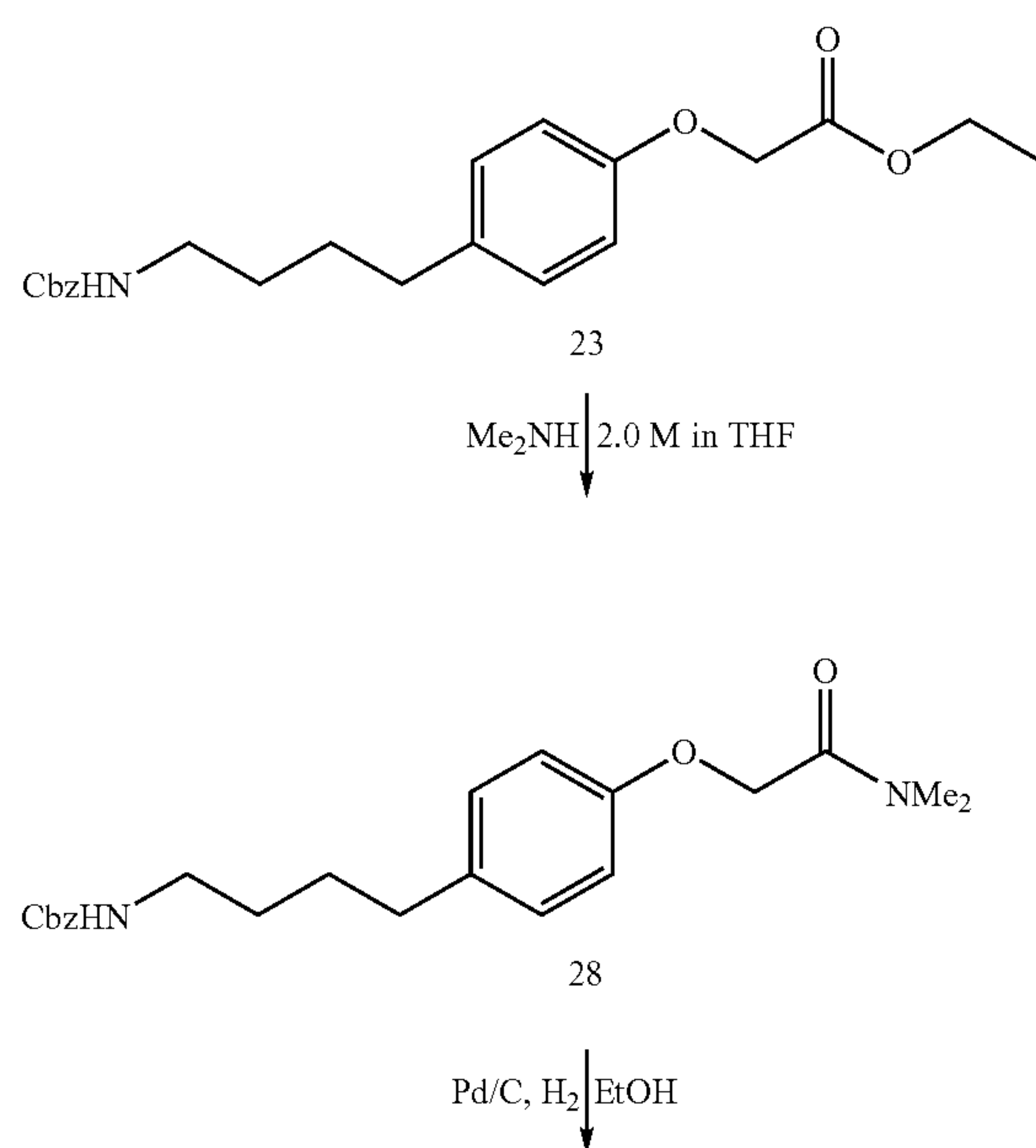
Scheme 7. Synthesis of PSA 16313
