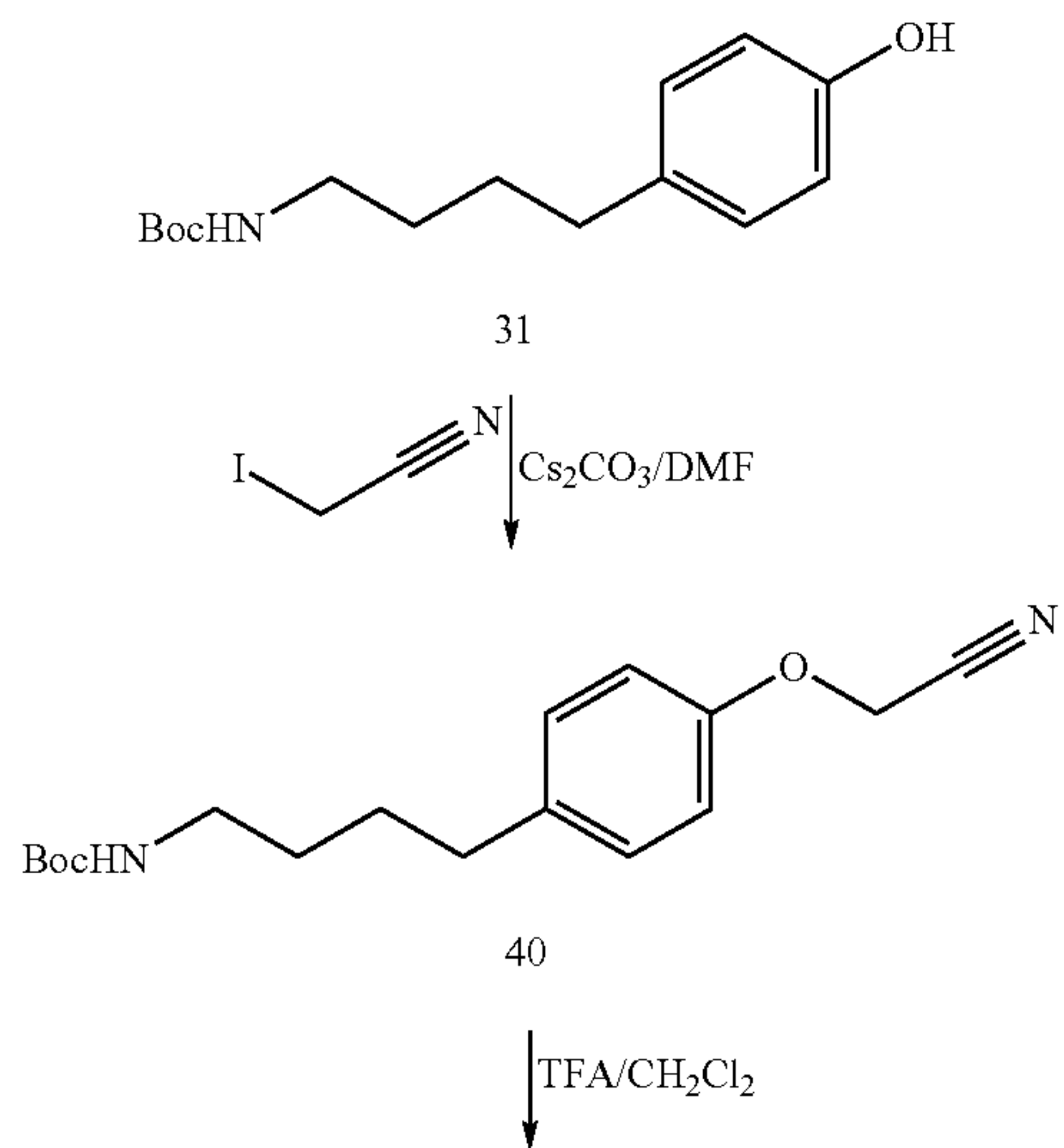
Scheme 10. Synthesis of PSA 16208
