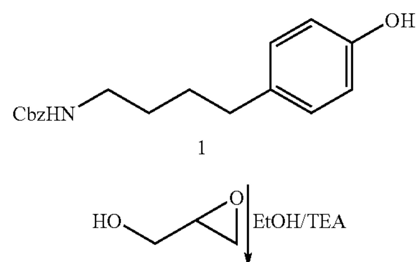
Scheme 11. Synthesis of PSA 15143
