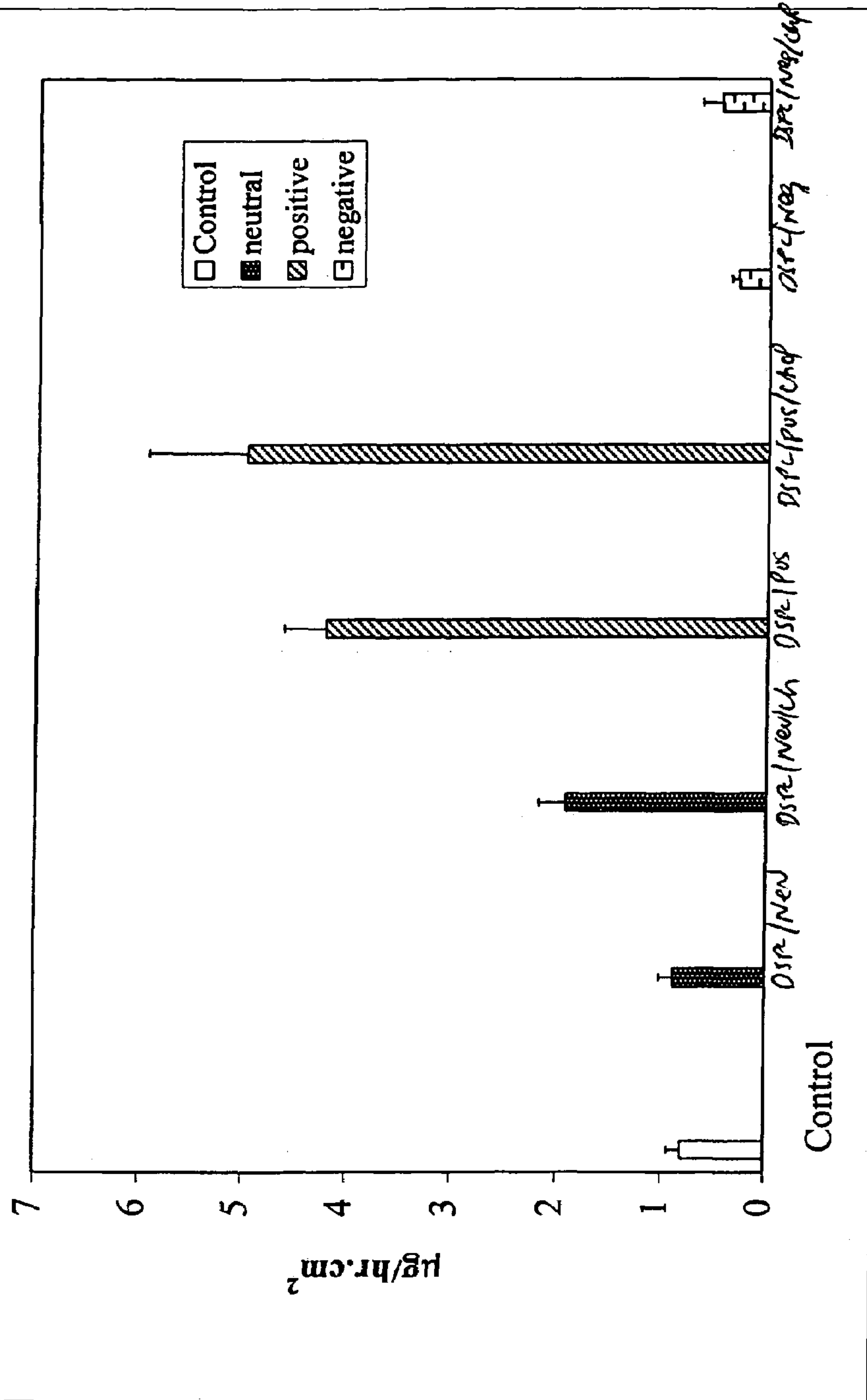
Figure 2. Glyburide flux across Caco-2 cells in DSPC formulations
