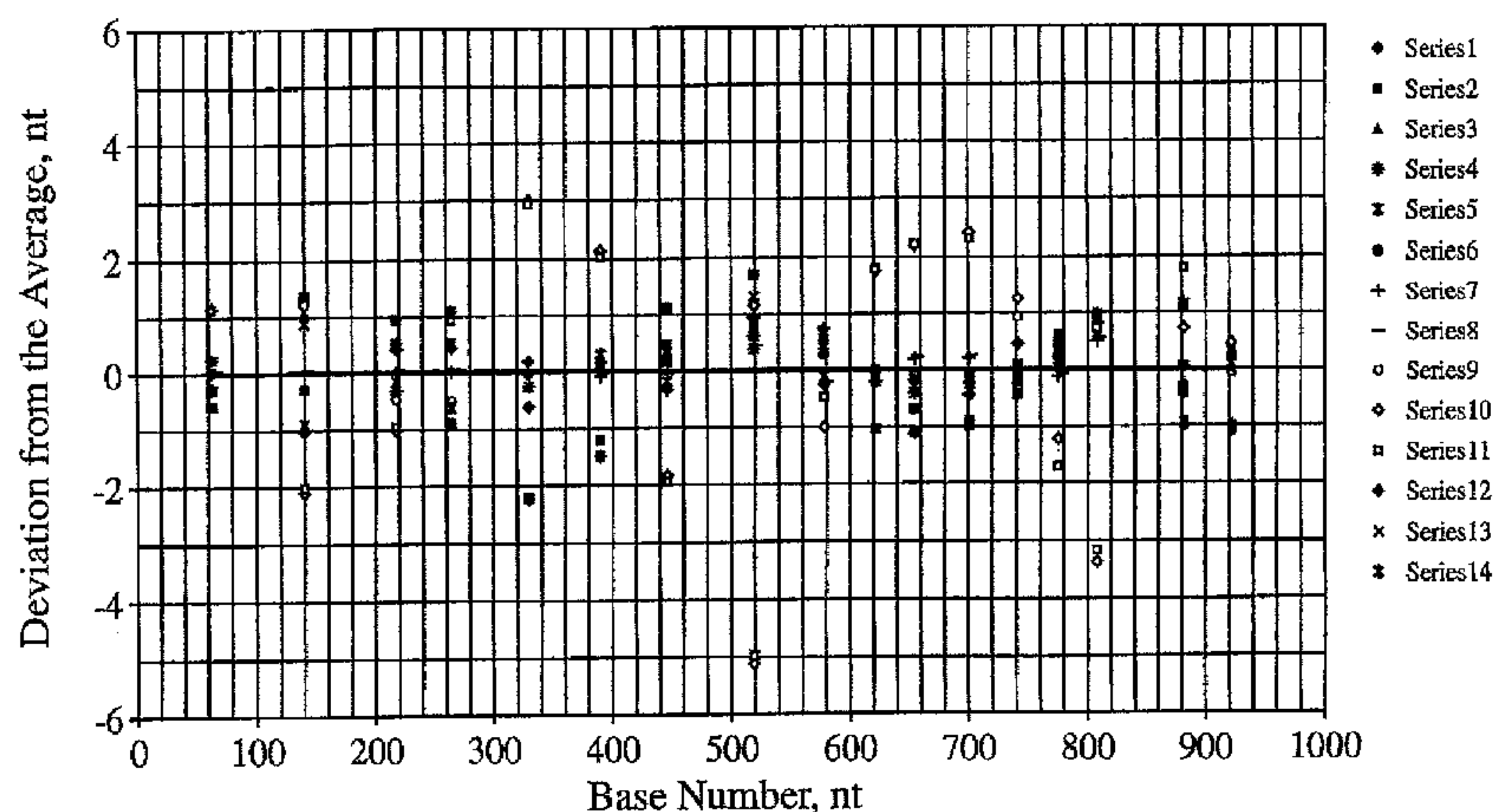
Deviation of the Peak Position (in Number of Bases) from the Average as a Function of Base Number in the Traces Aligned with Internal Standards (long gel, M13, 17 peaks, 5-th degree polynomial)
