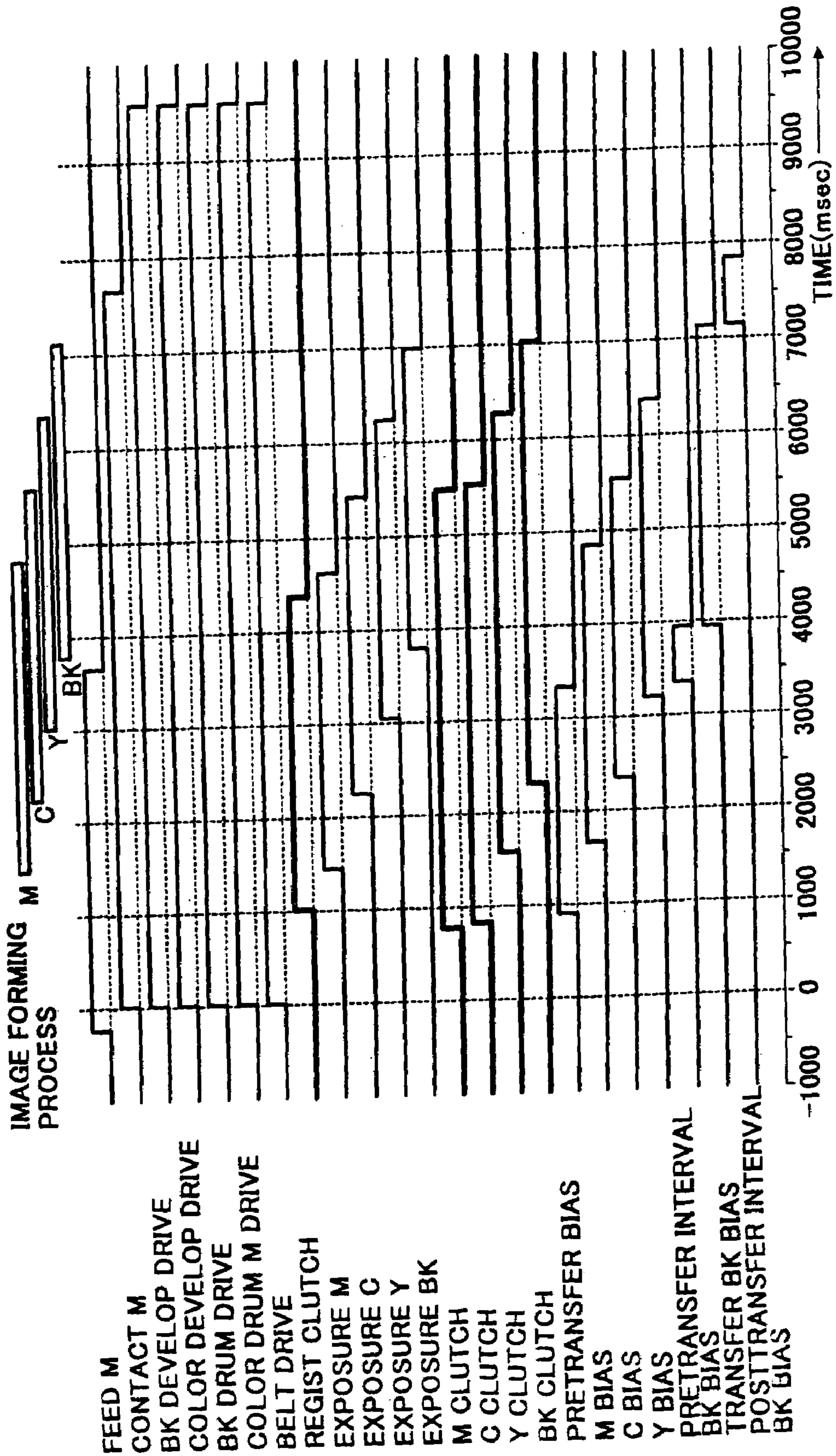
FIG. 1 PRIOR ART
