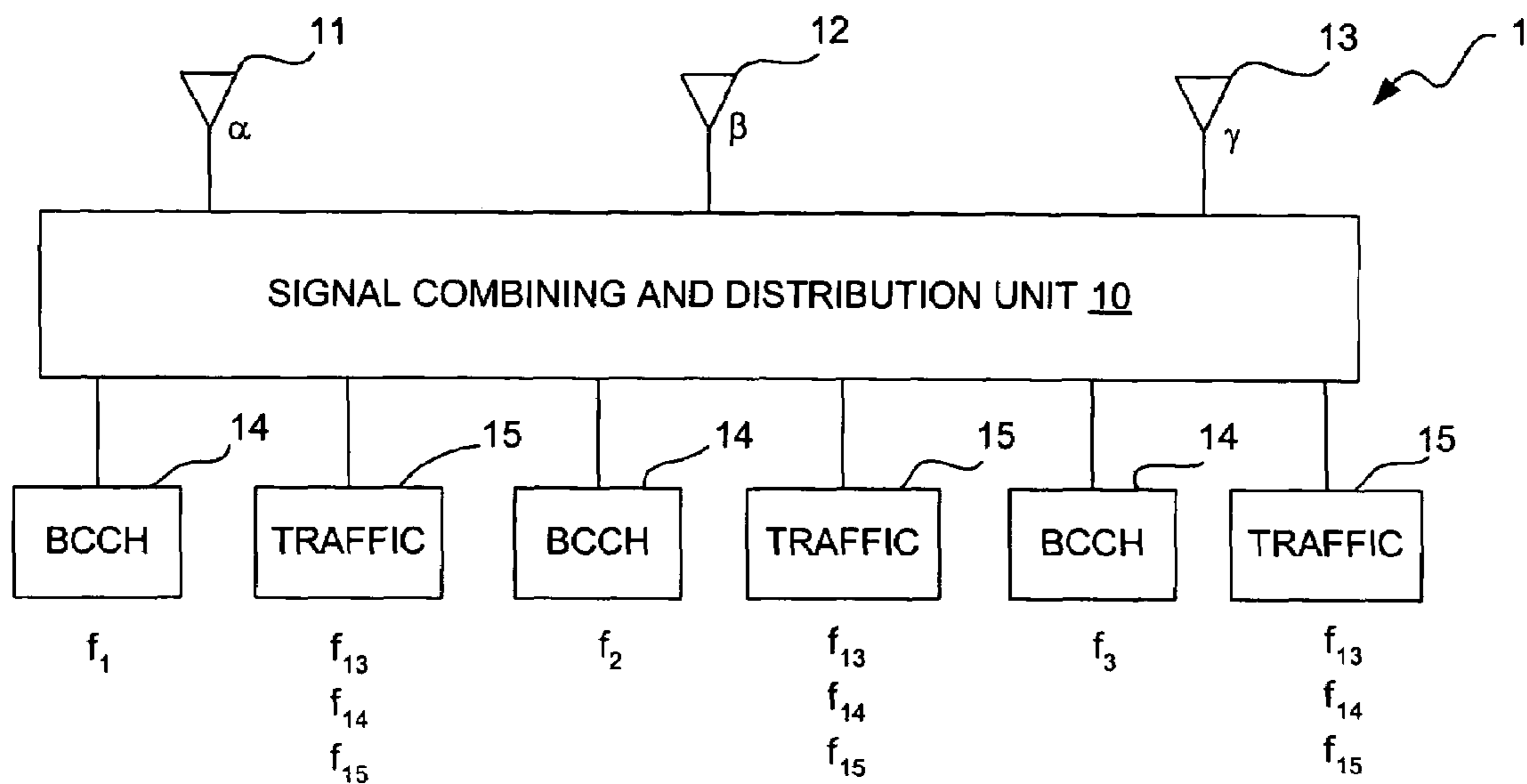
FIG. 2 (PRIOR ART)
