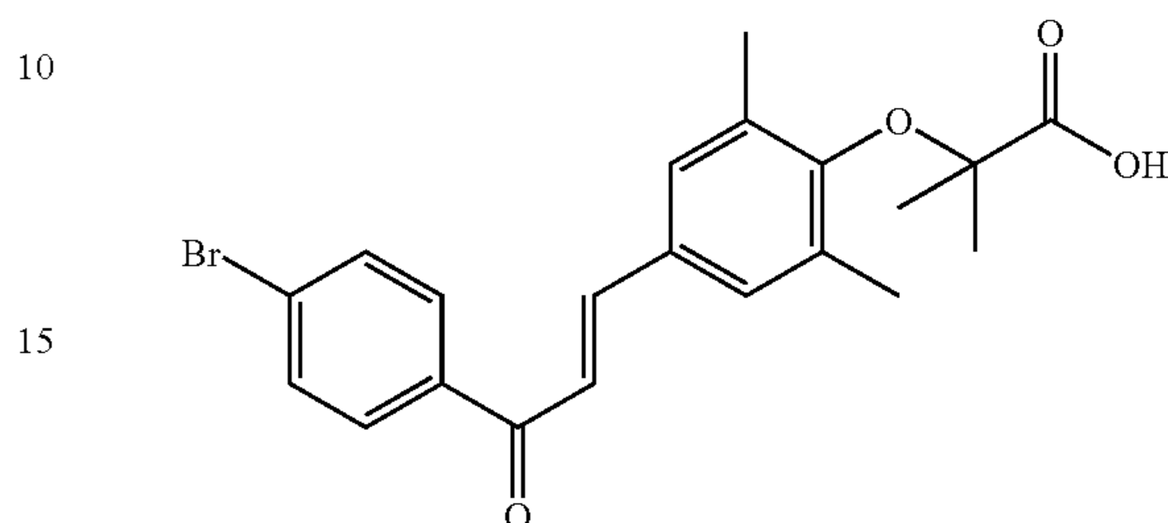
1-[4-bromophenyl]-3-[3,5-dimethyl-4-carboxydimethylmethoxyphenyl]prop-2-en-1-one (Compound 18)
