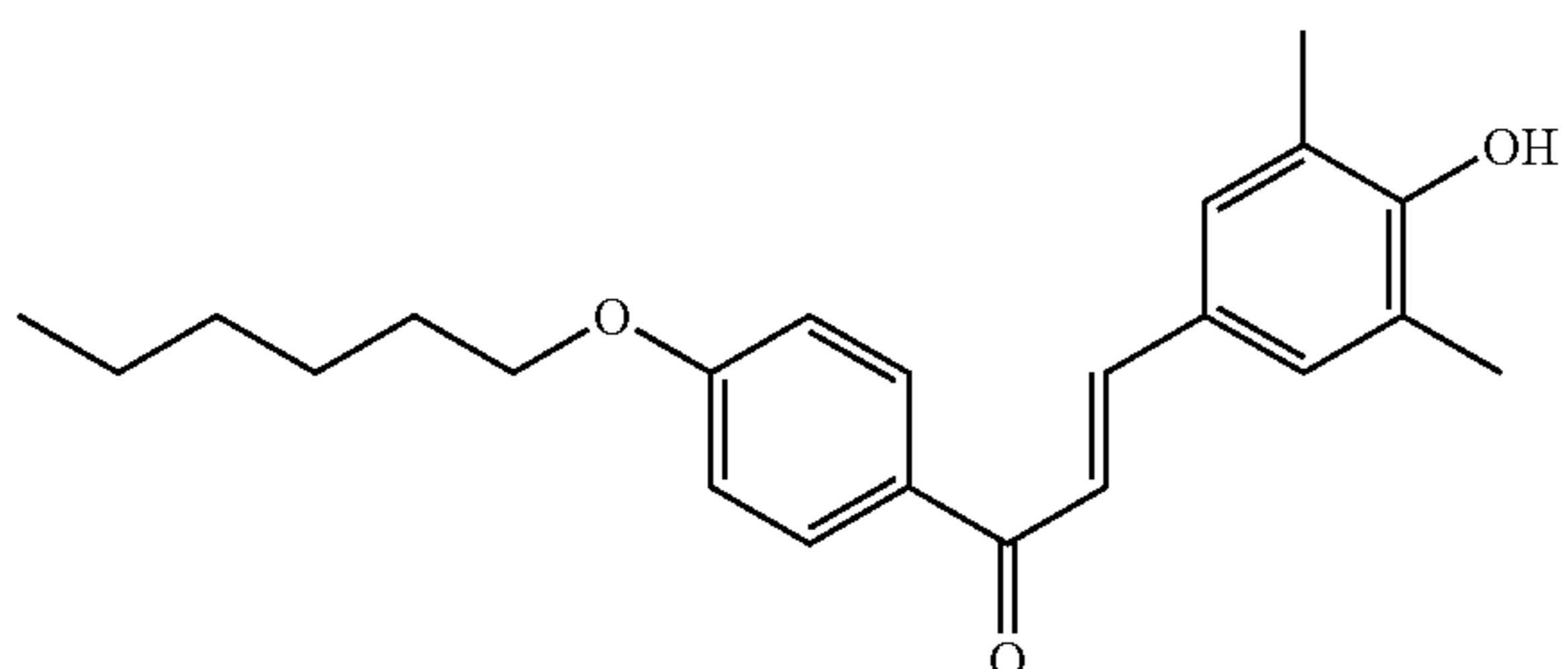
1-[4-hexyloxyphenyl]-3-[3,5-dimethyl-4-hydroxydimethylmethoxyphenyl]prop-2-en-1-one (Compound 10)
