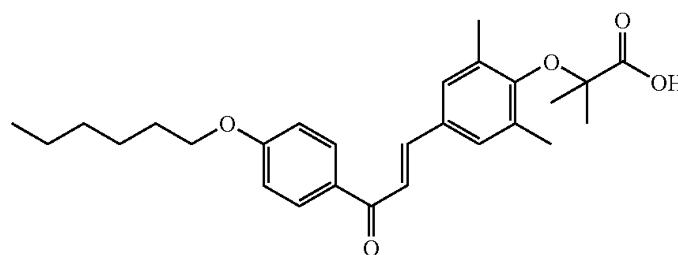
1-[4-hexyloxyphenyl]-3-[3,5-dimethyl-4-carboxydimethylmethoxyphenyl]prop-2-en-1-one (Compound 12)
