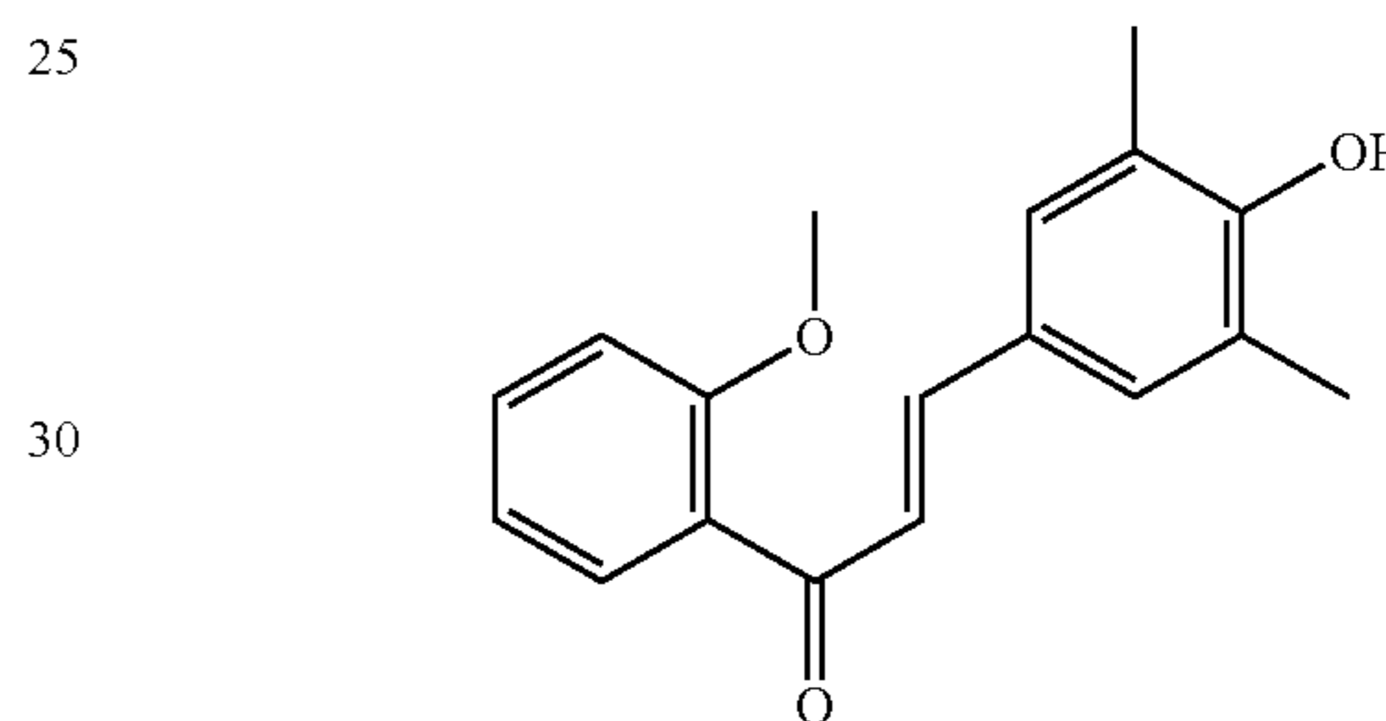
1-[2-methoxyphenyl]-3-[3,5-dimethyl-4-hydroxyphenyl]prop-2-en-1-one (Compound 4)
