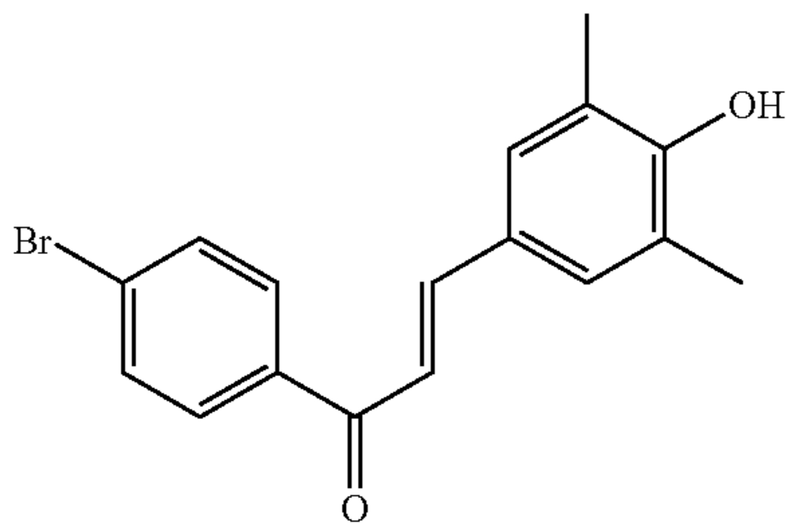
1-[4-bromophenyl]-3-[3,5-dimethyl-4-hydroxyphenyl]prop-2-en-1-one (Compound 16)
