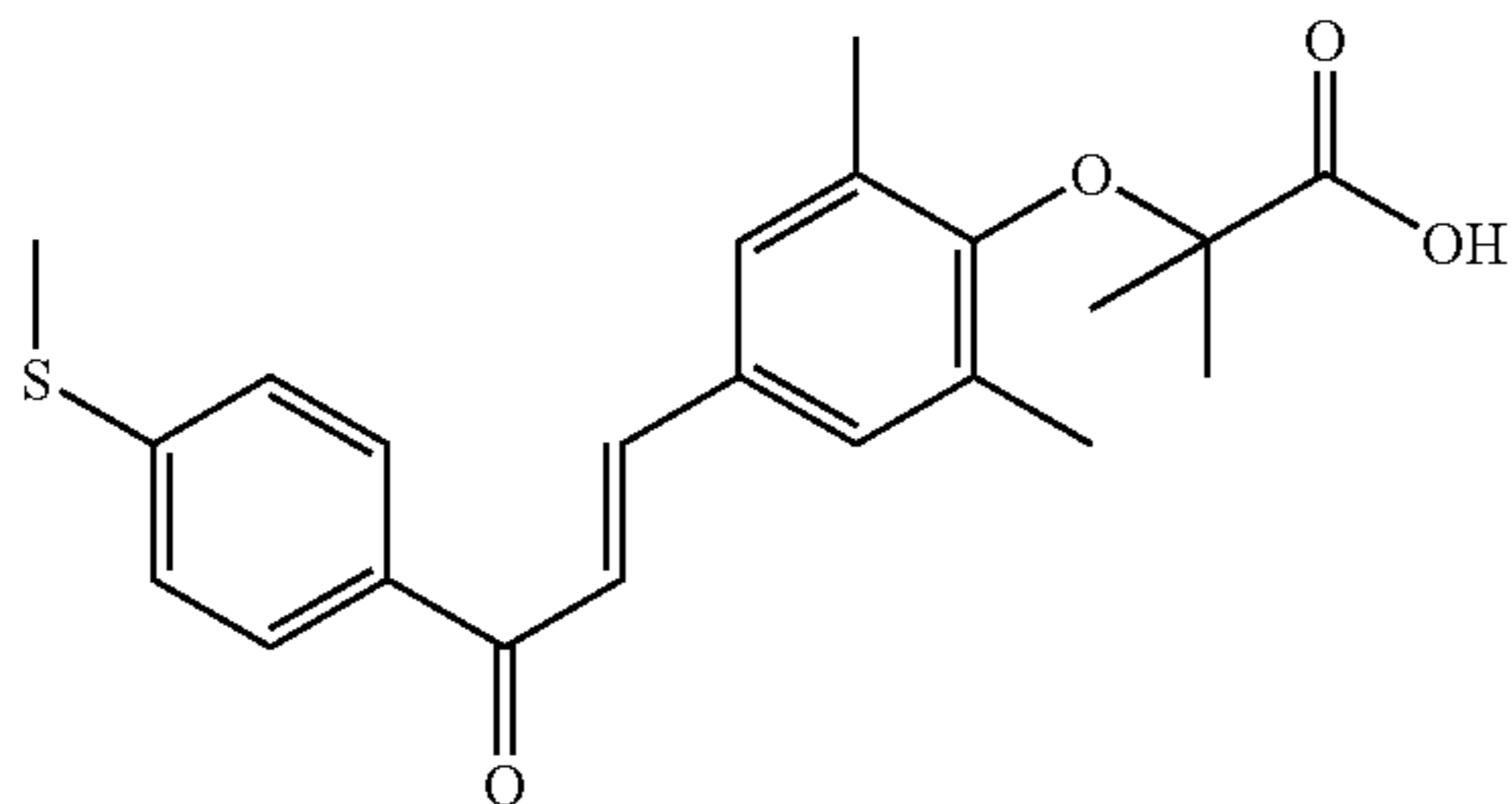
1-[4-methylthiophenyl]-3-[3,5-dimethyl-4-carboxydimethylmethoxyphenyl]prop-2-en-1-one (Compound 9)
