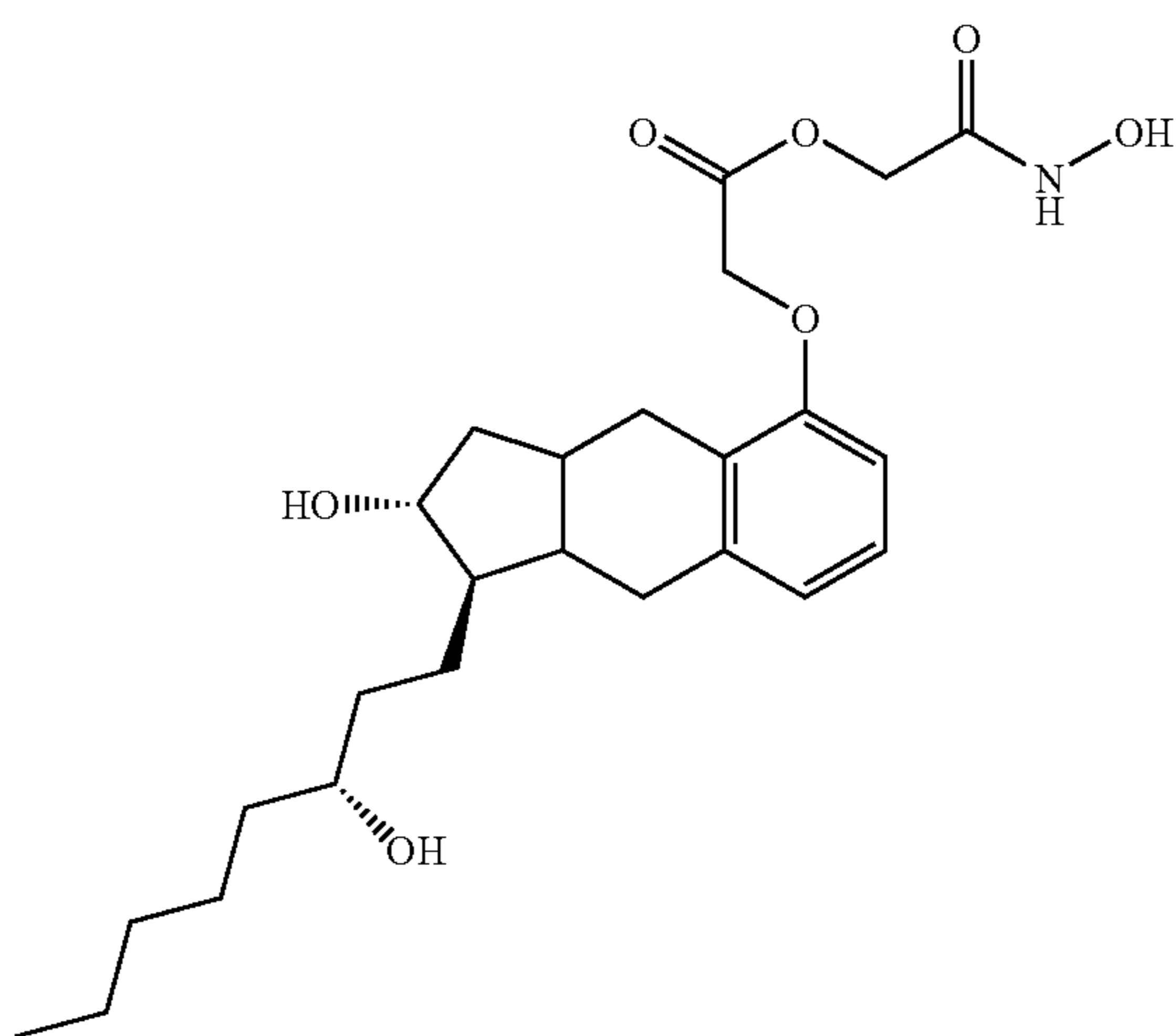
C_{25}H_{37}NO_7 Exact Mass: 463.26 Mol. Wt.: 463.56 C, 64.77; H, 8.05; N, 3.02; O, 24.16 Treprostinil N-hydroxy glycolamide ester D
