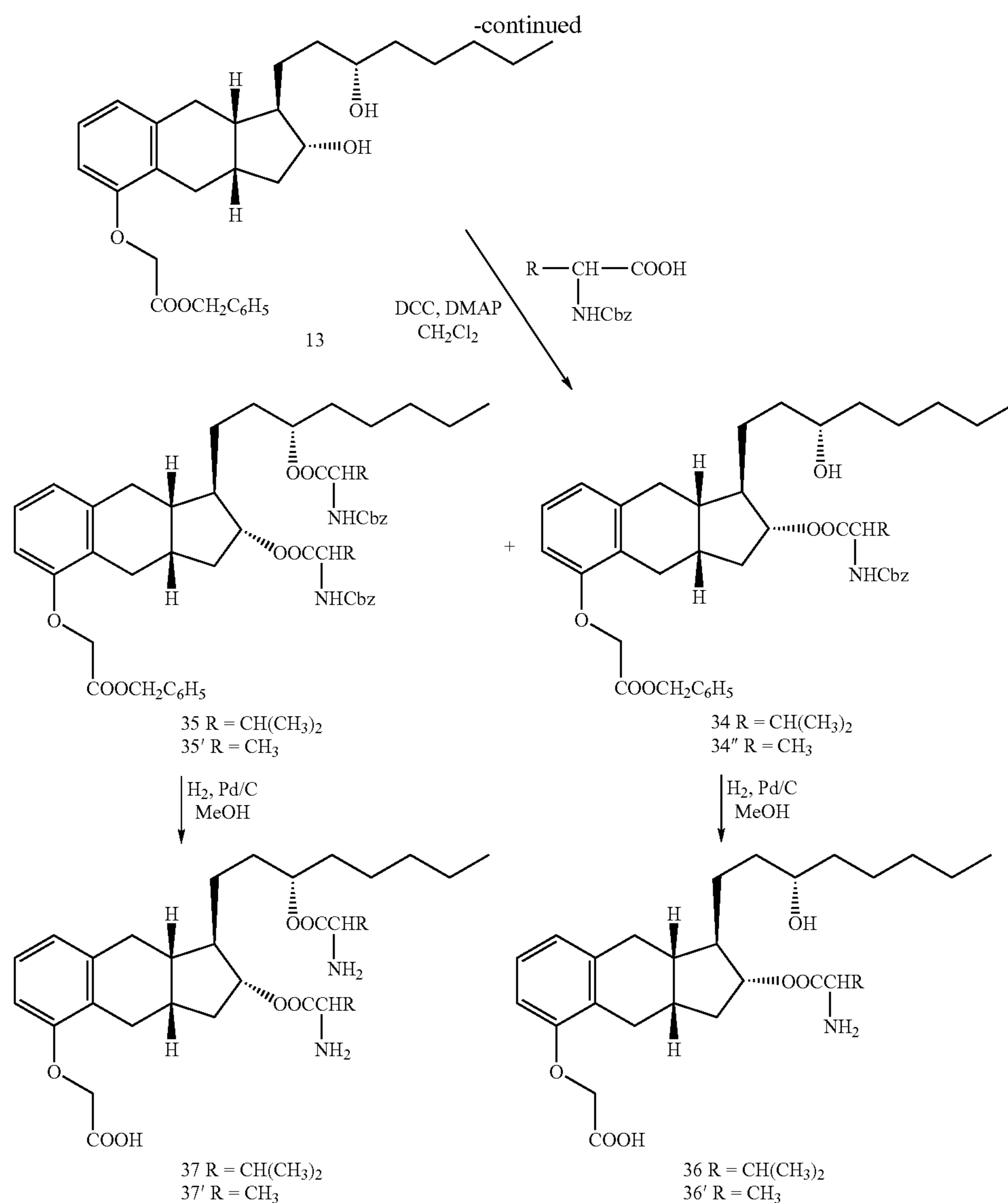
Synthesis of 2-N-Cbz-L-valine Ester of Treprostinil Benzyl Ester 34 and bis-N-Cbz-L-valine Ester of Treprostinil Benzyl Ester 35
