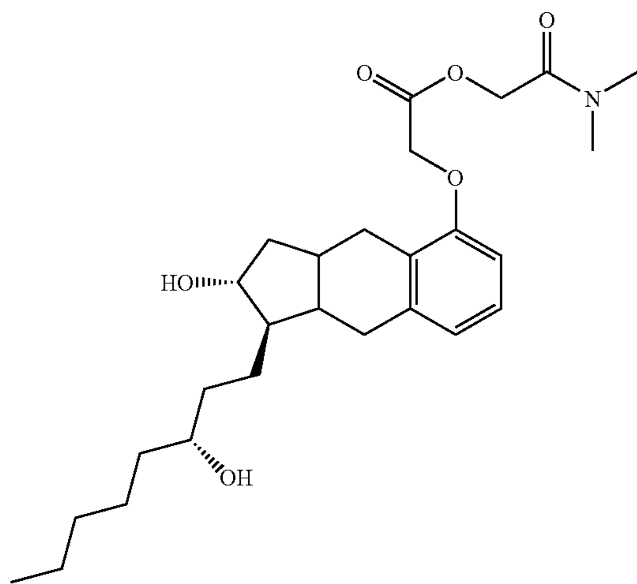
C_{27}H_{41}NO_6 Exact Mass: 475.29 Mol. Wt.: 475.62 C, 68.18; H, 8.69; N, 2.94; O, 20.18 Treprostinil N,N-dimethyl glycolamide C
