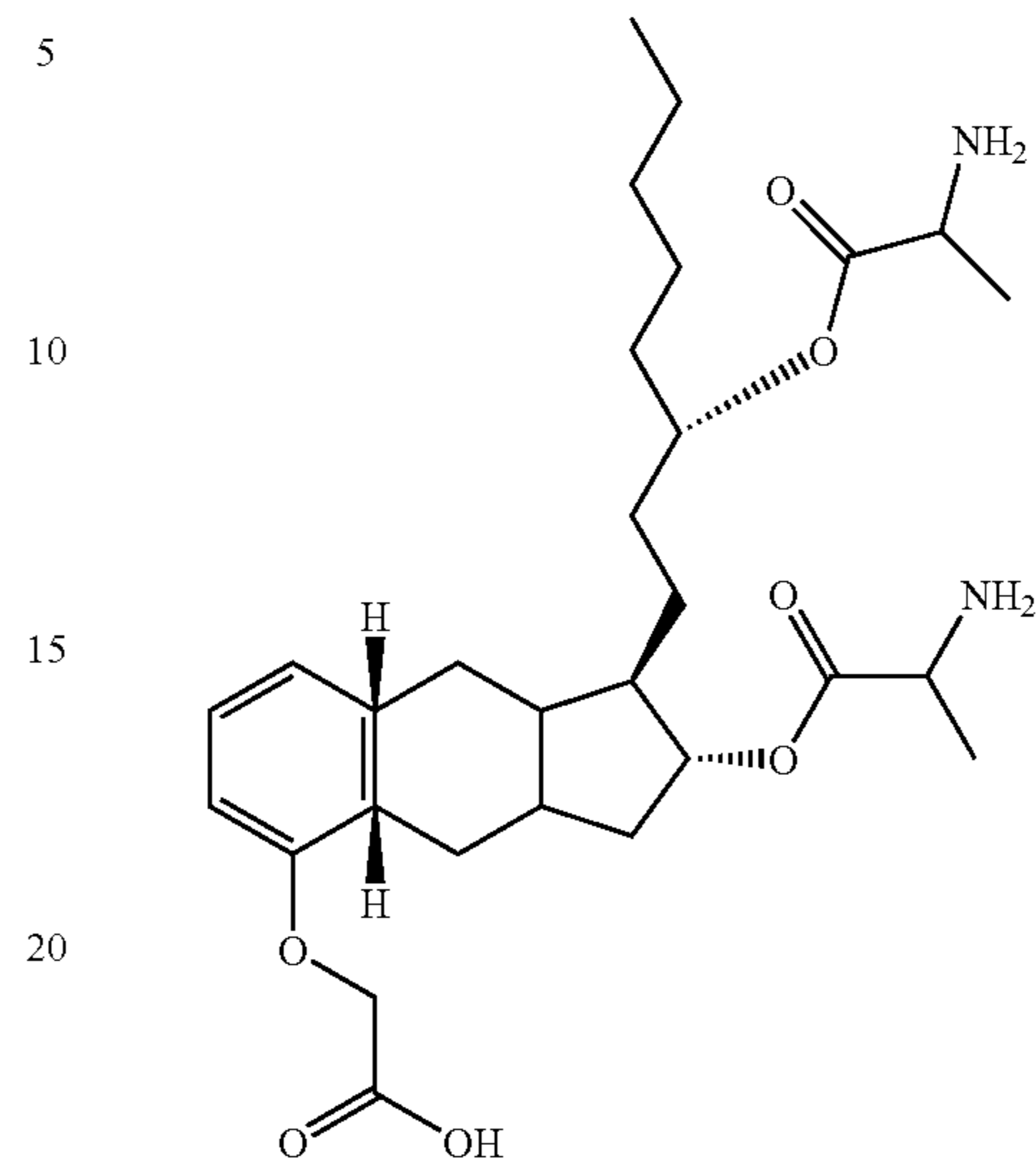
C_{29}H_{44}N_2O_7 Exact Mass: 532.31 Mol. Wt.: 532.67 C, 65.39; H, 8.33; N, 5.26; O, 21.03 P
