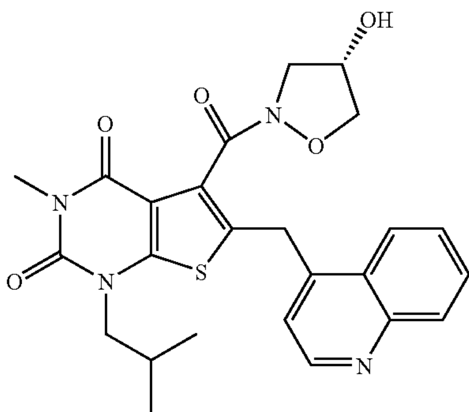
a) (S) Methyl 2-[4-hydroxyisoxazolidin-2-yl]carbonylbenzoate
