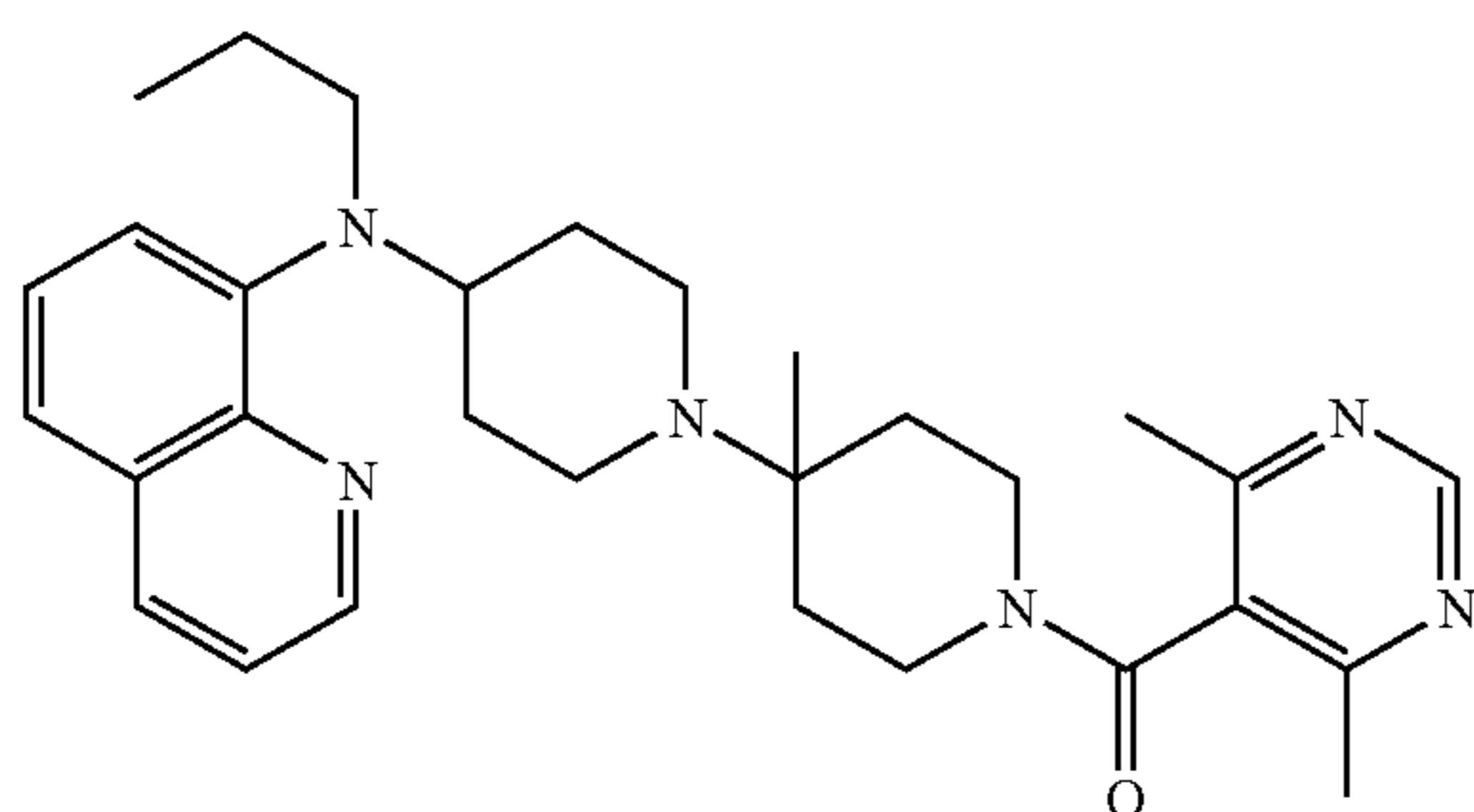
Compound 110
