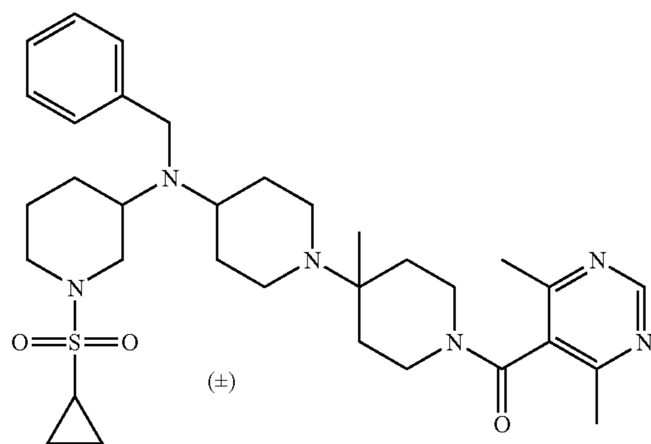
Compound 112
