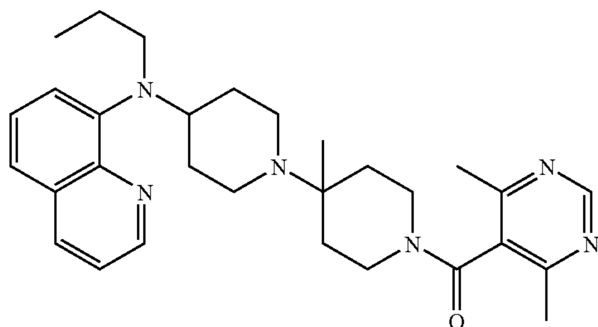
Compound 110
