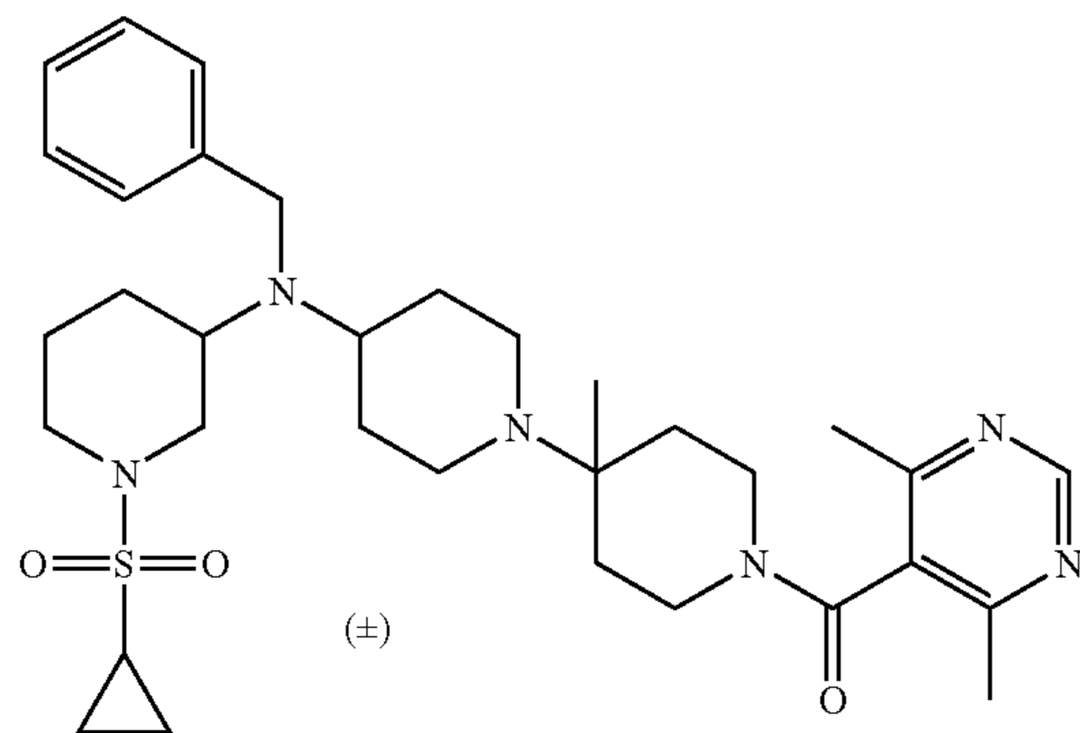
Compound 112
