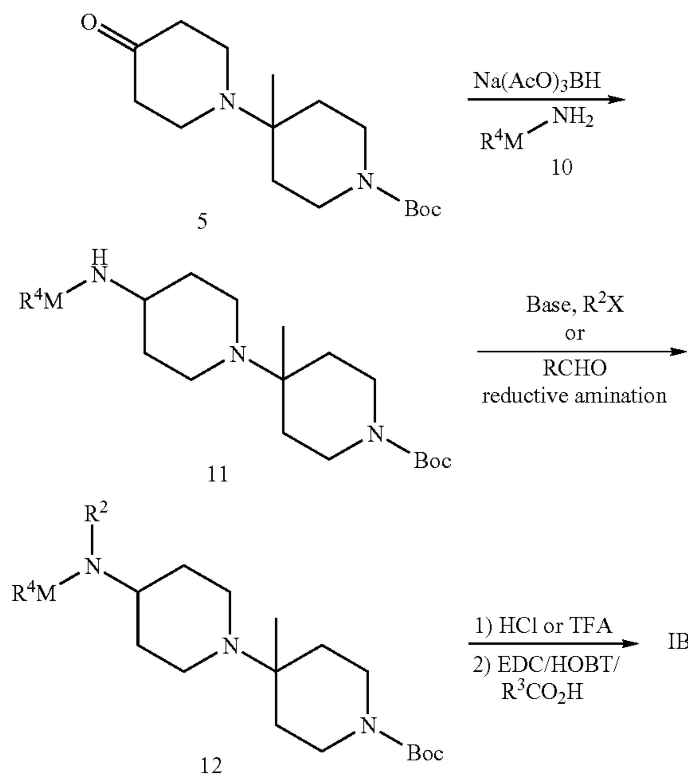
Scheme B
