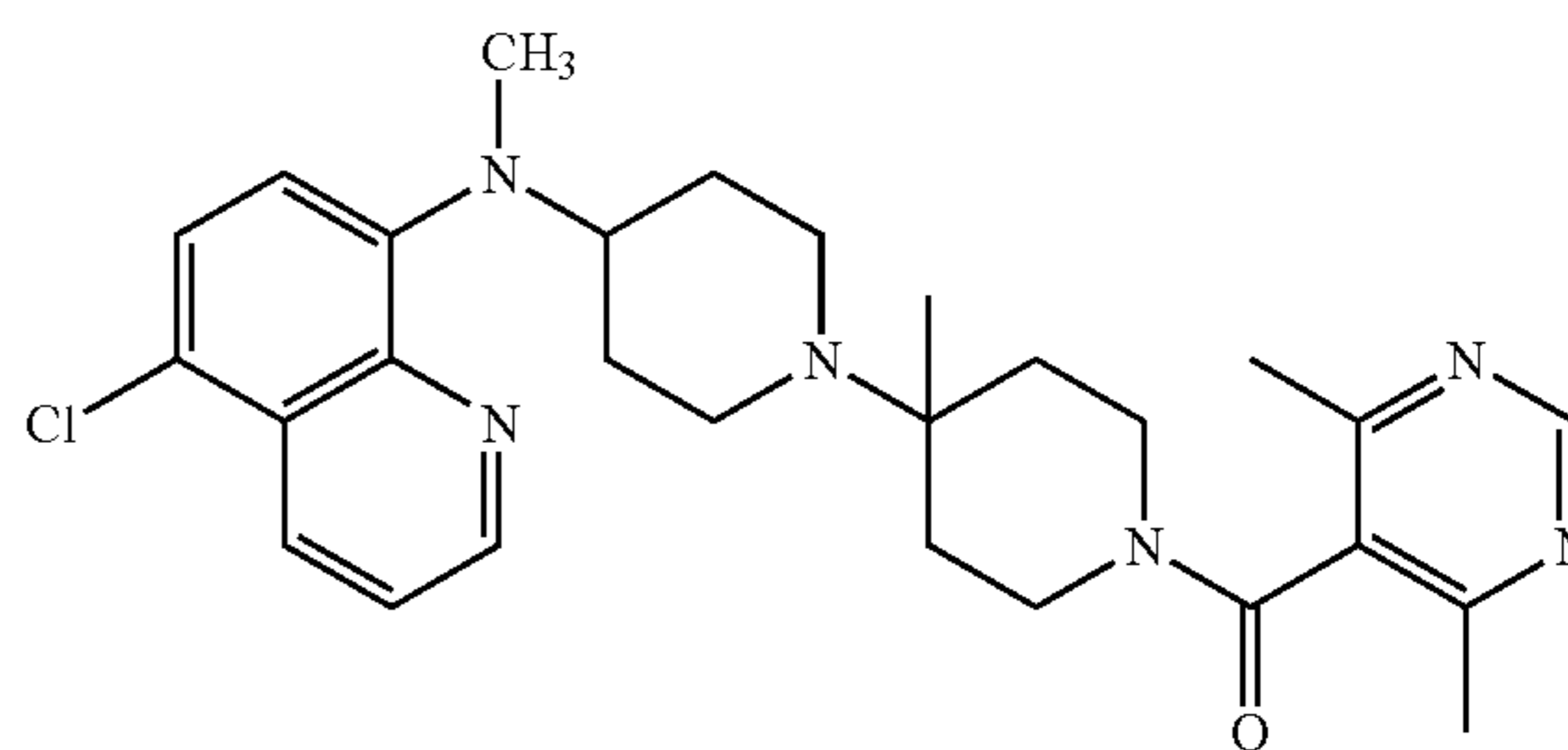
Compound 111
