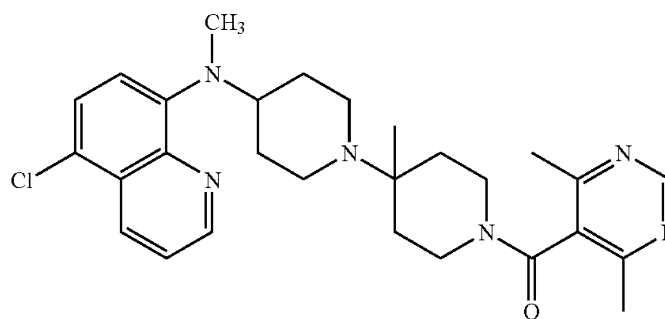
Compound 111
