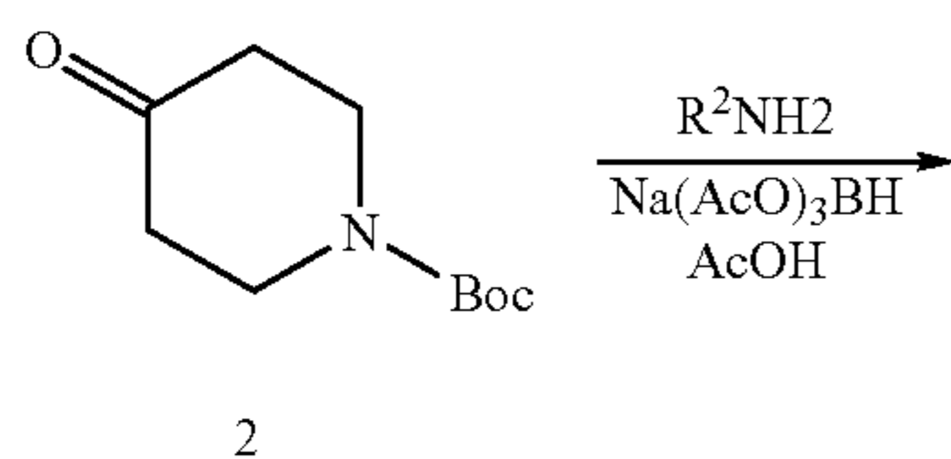
Scheme C
