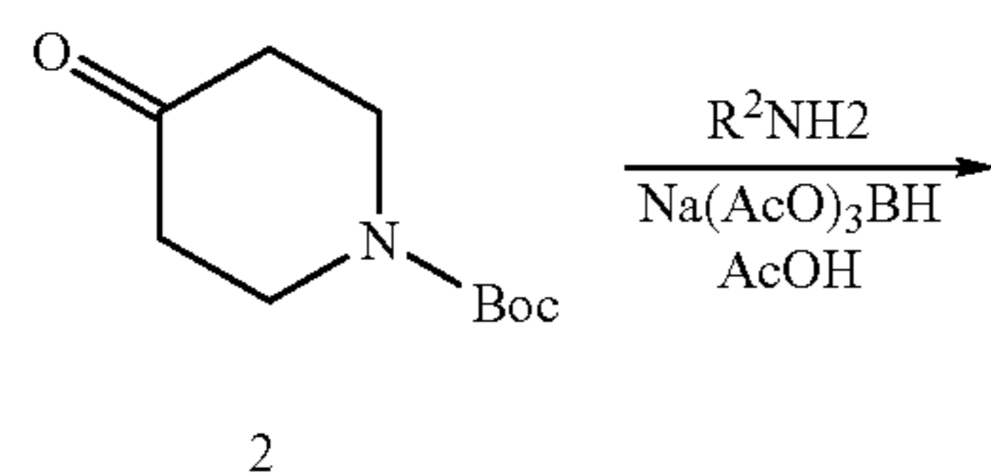
Scheme C
