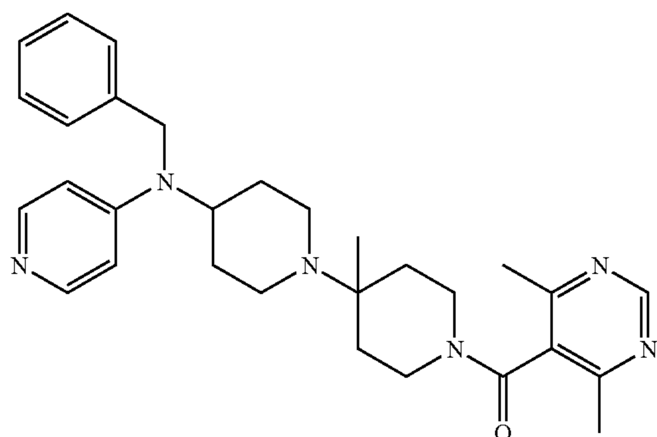
Compound 108
