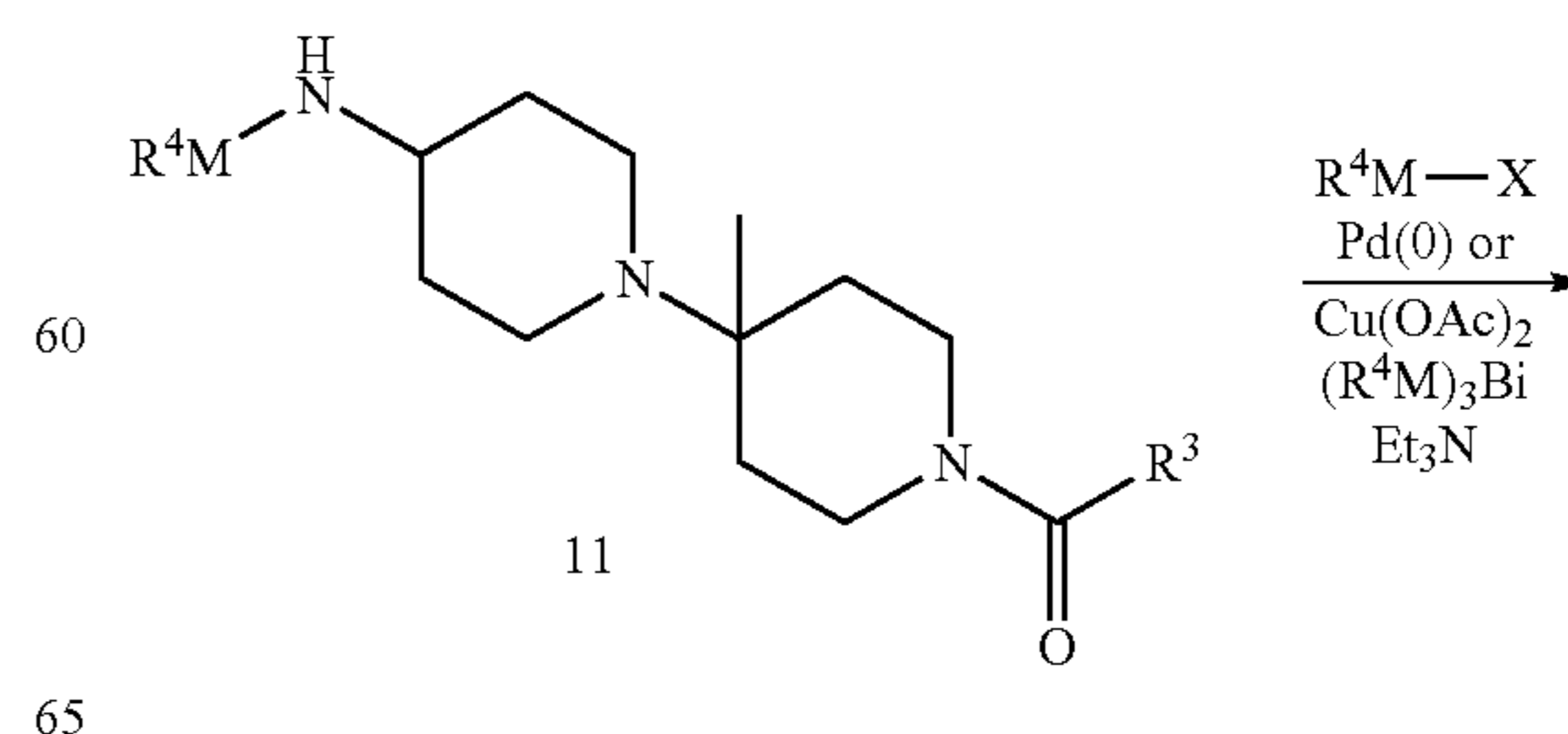
Scheme D
