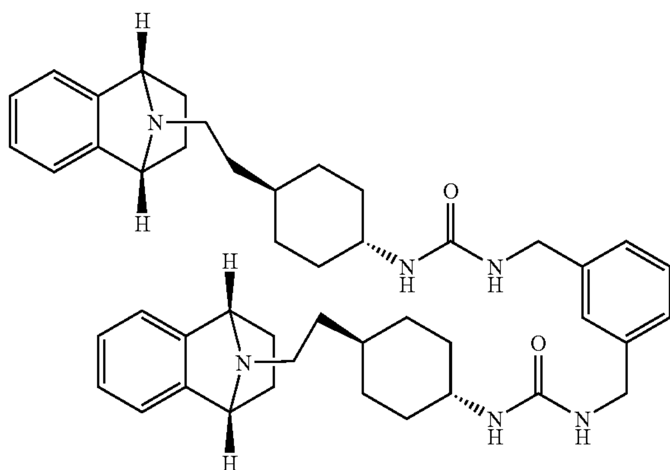
N,N''-(benzene-1,3-diylidimethanediyl)bis[N-(trans-4-{2-[(1R,8S)-11-azatricyclo[6.2.1.0 2,7 ]undeca-2,4,6-trien-11-yl]ethyl}cyclohexyl)urea]
