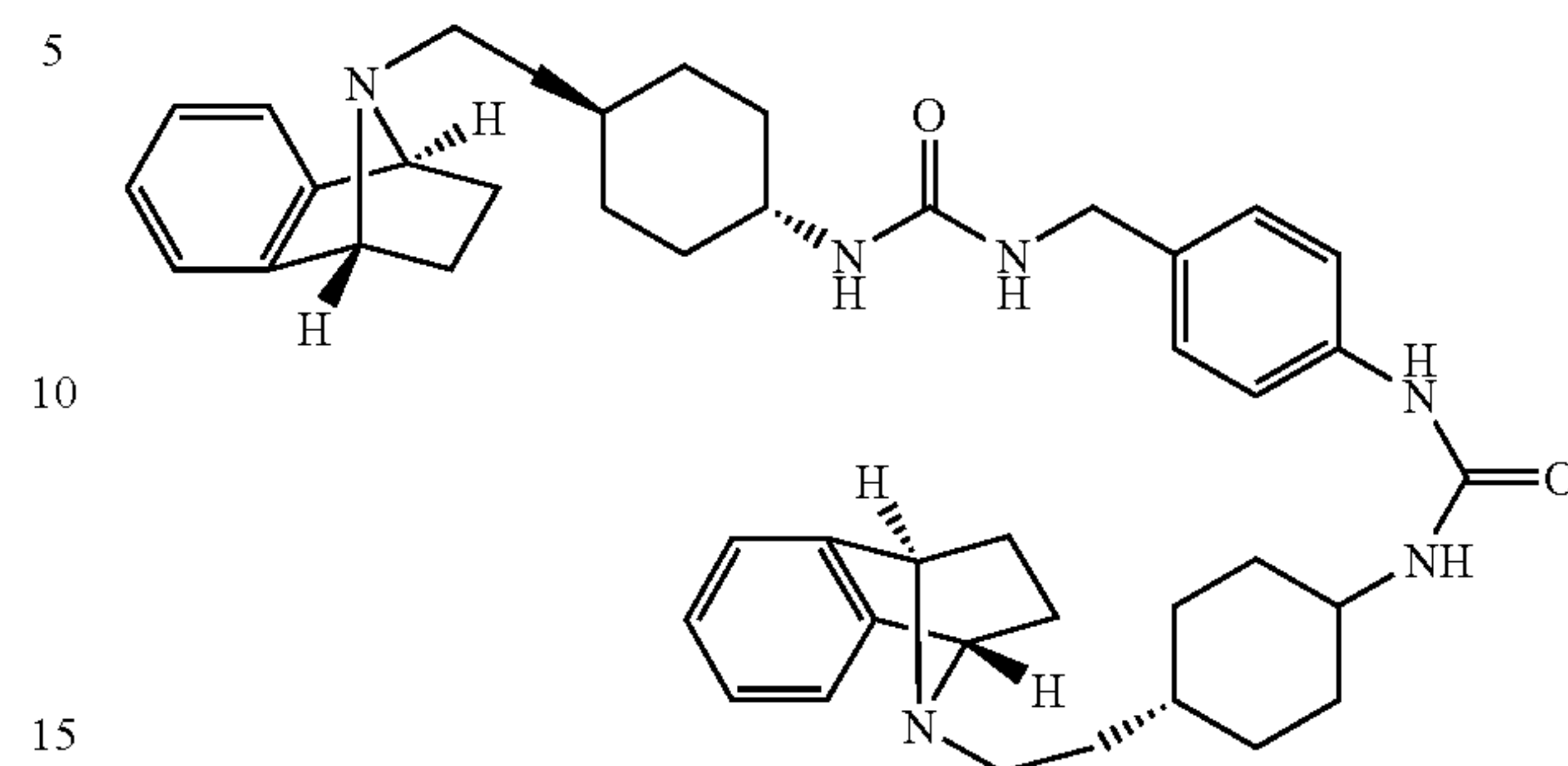
N-(trans-4-{2-[(1R,8S)-11-azatricyclo[6.2.1.0 2,7 ]undeca-2,4,6-trien-11-yl]ethyl}cyclohexyl)-N-{4-[(trans-4-{2-[(1R,8S)-11-azatricyclo[6.2.1.0 2,7 ]undeca-2,4,6-trien-11-yl]ethyl}cyclohexyl)amino]carbonyl}amino)methyl]phenyl}urea
