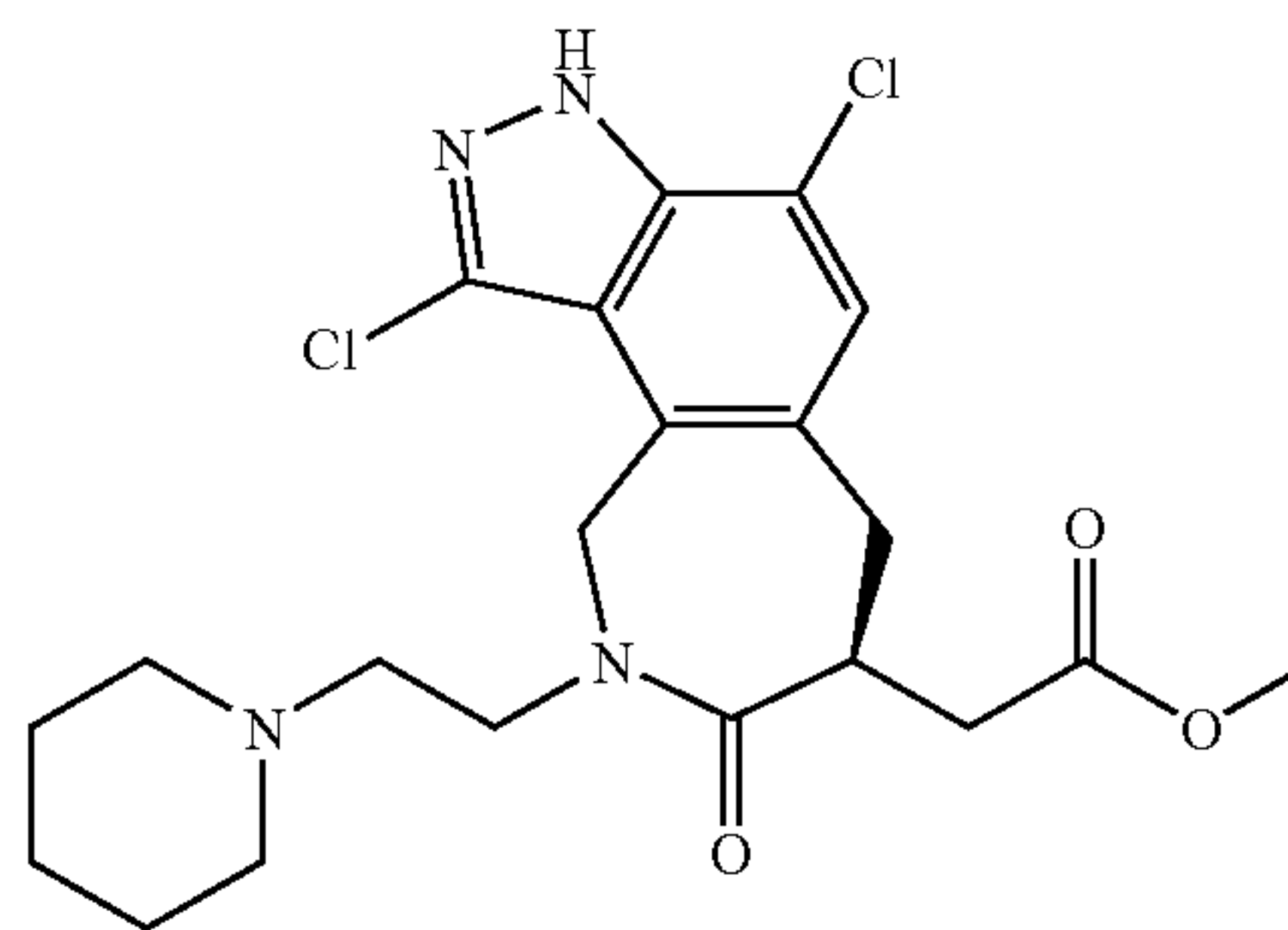
Intermediate 471
