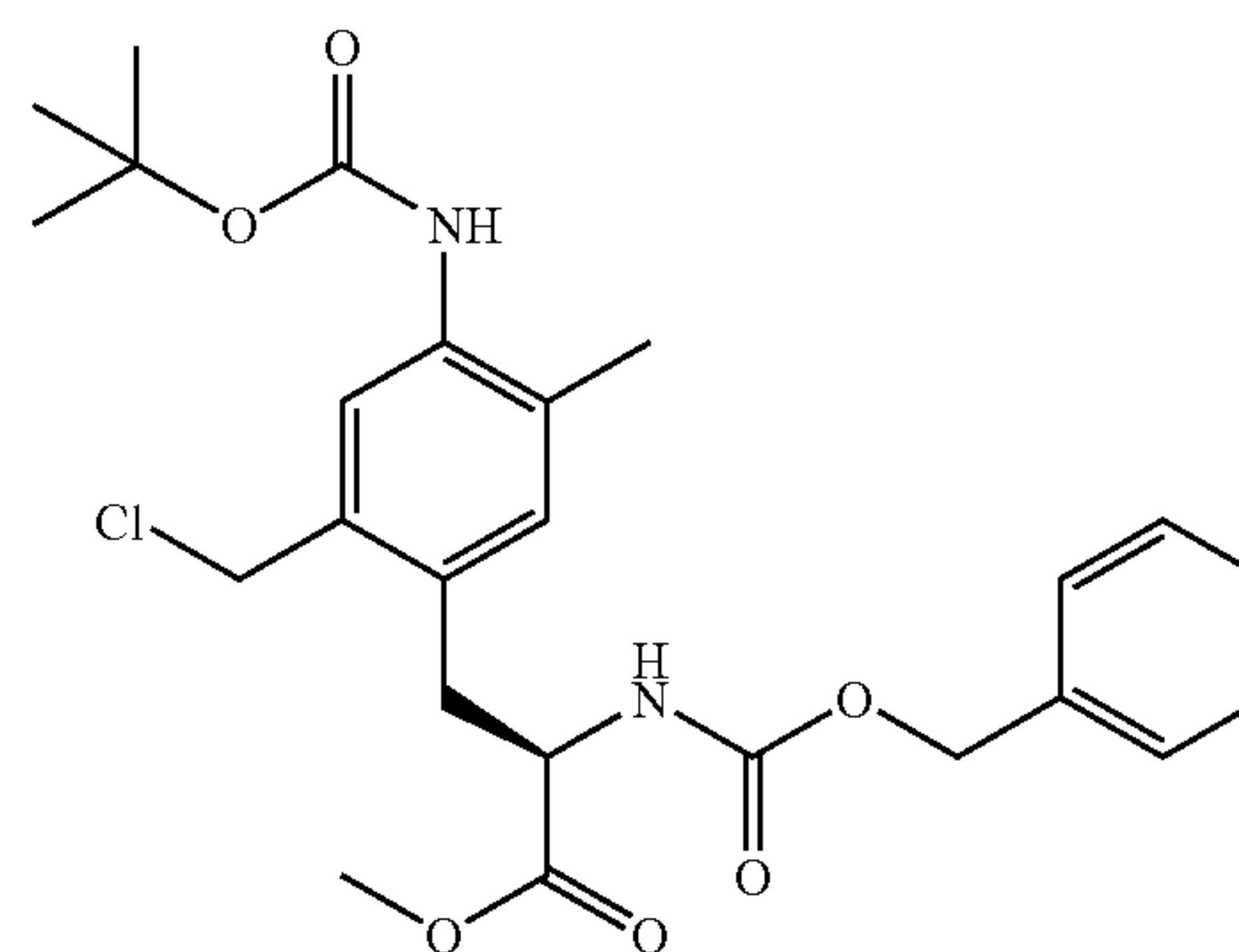
Intermediate 302
