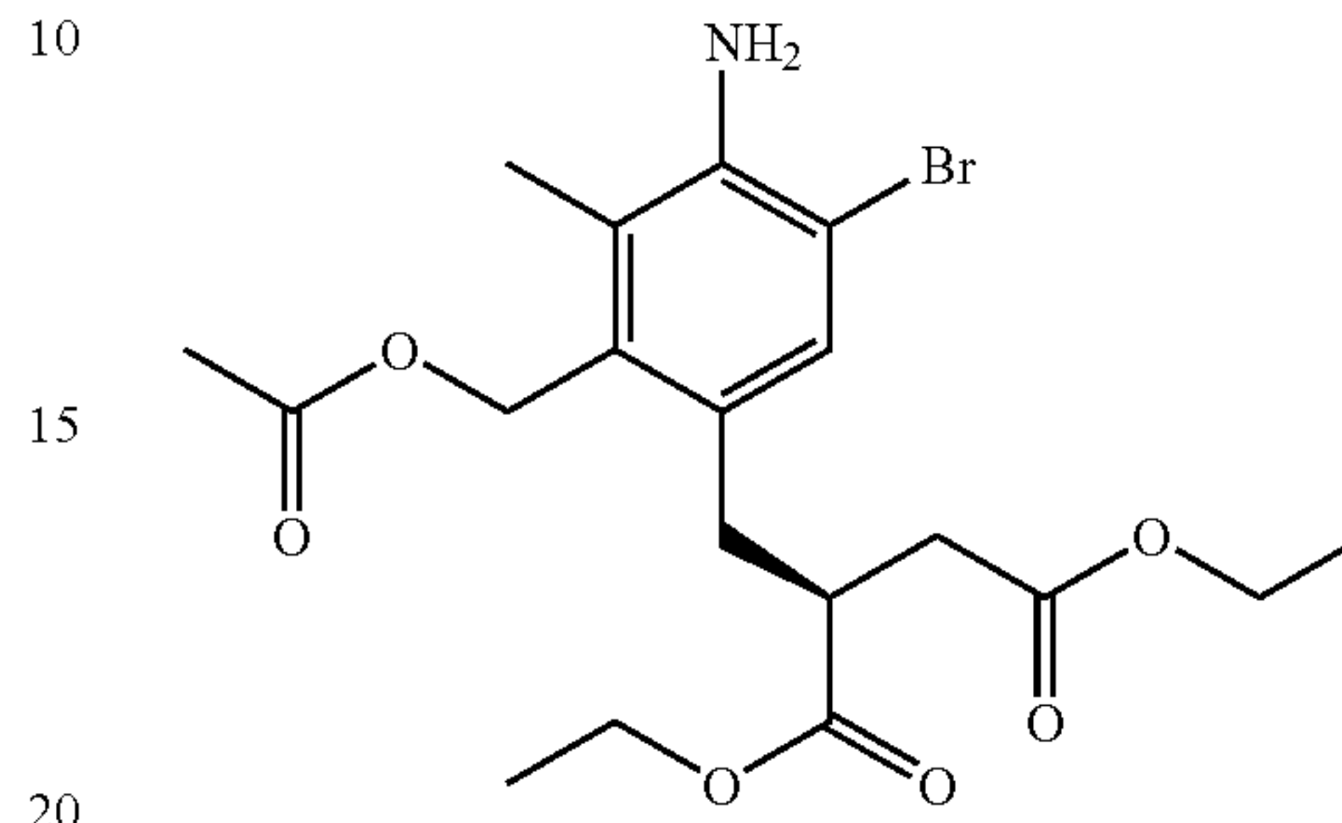
Intermediate 403
