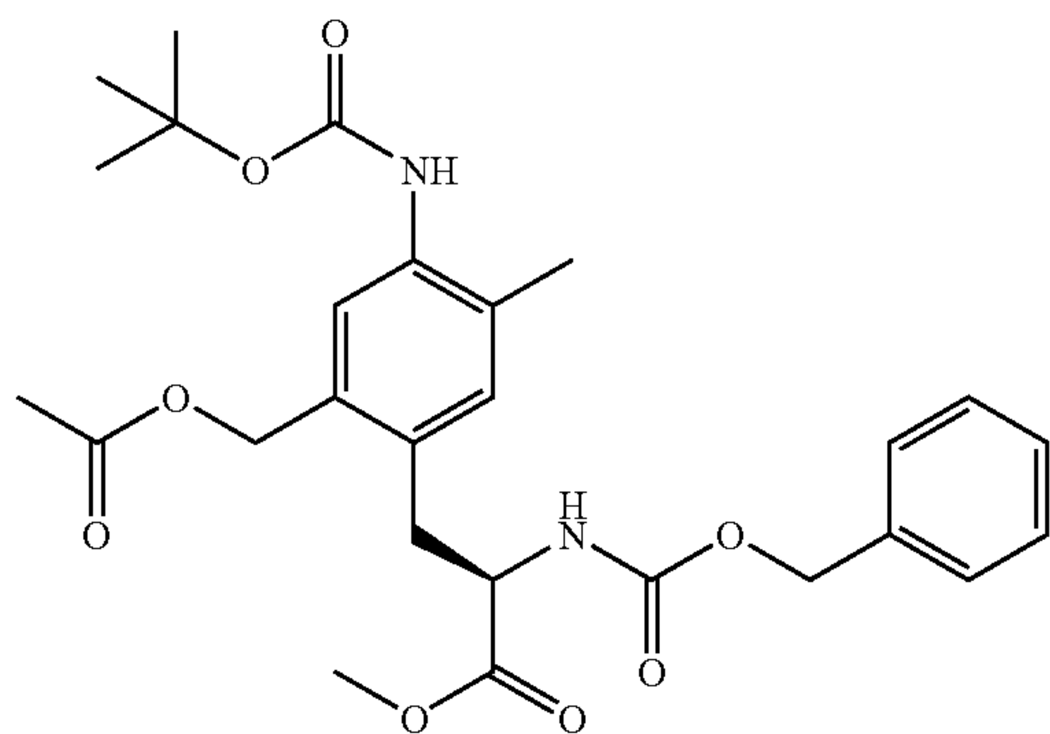
Intermediate 300
