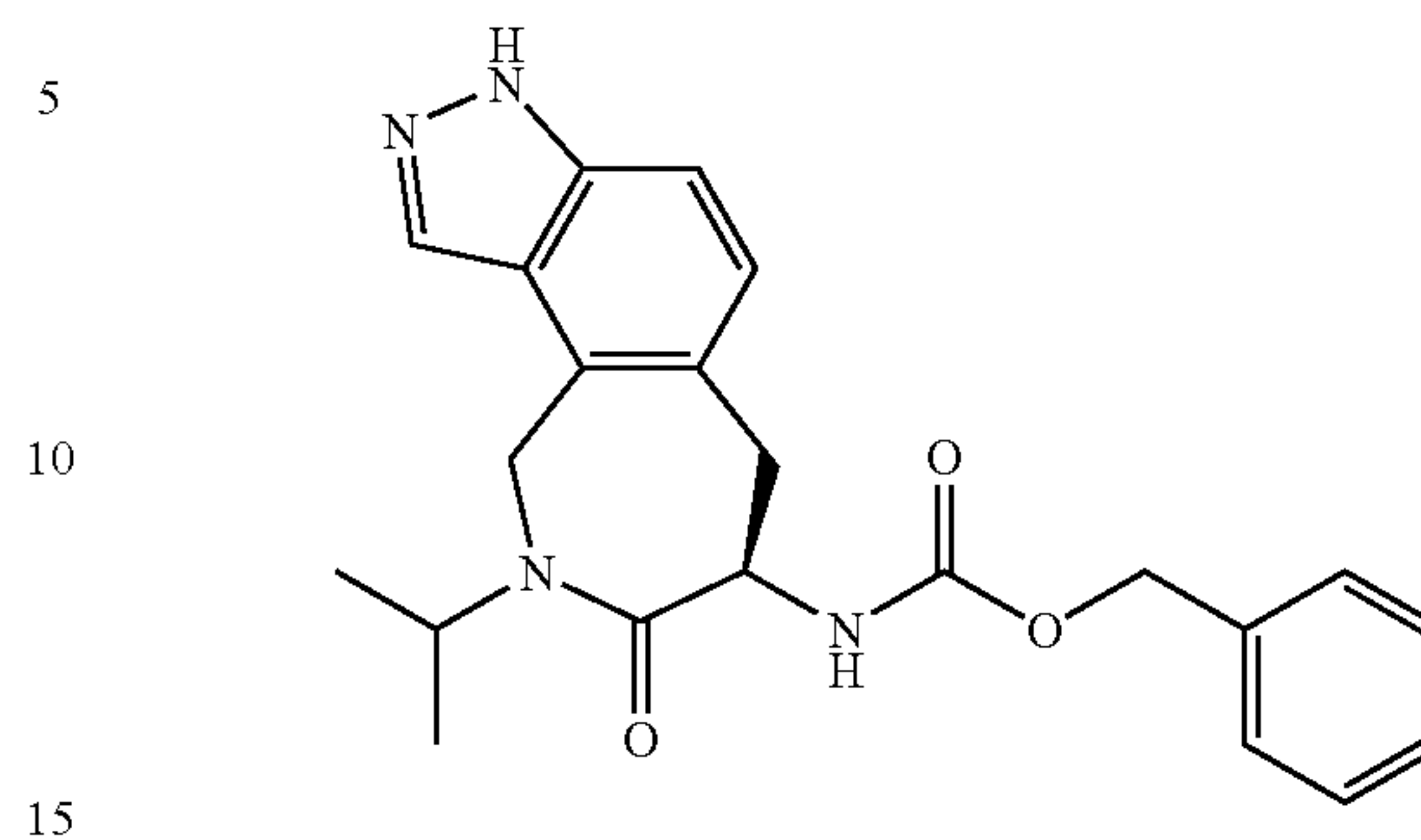
Intermediate 251
