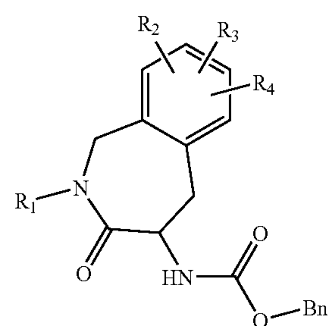
Scheme 2.
