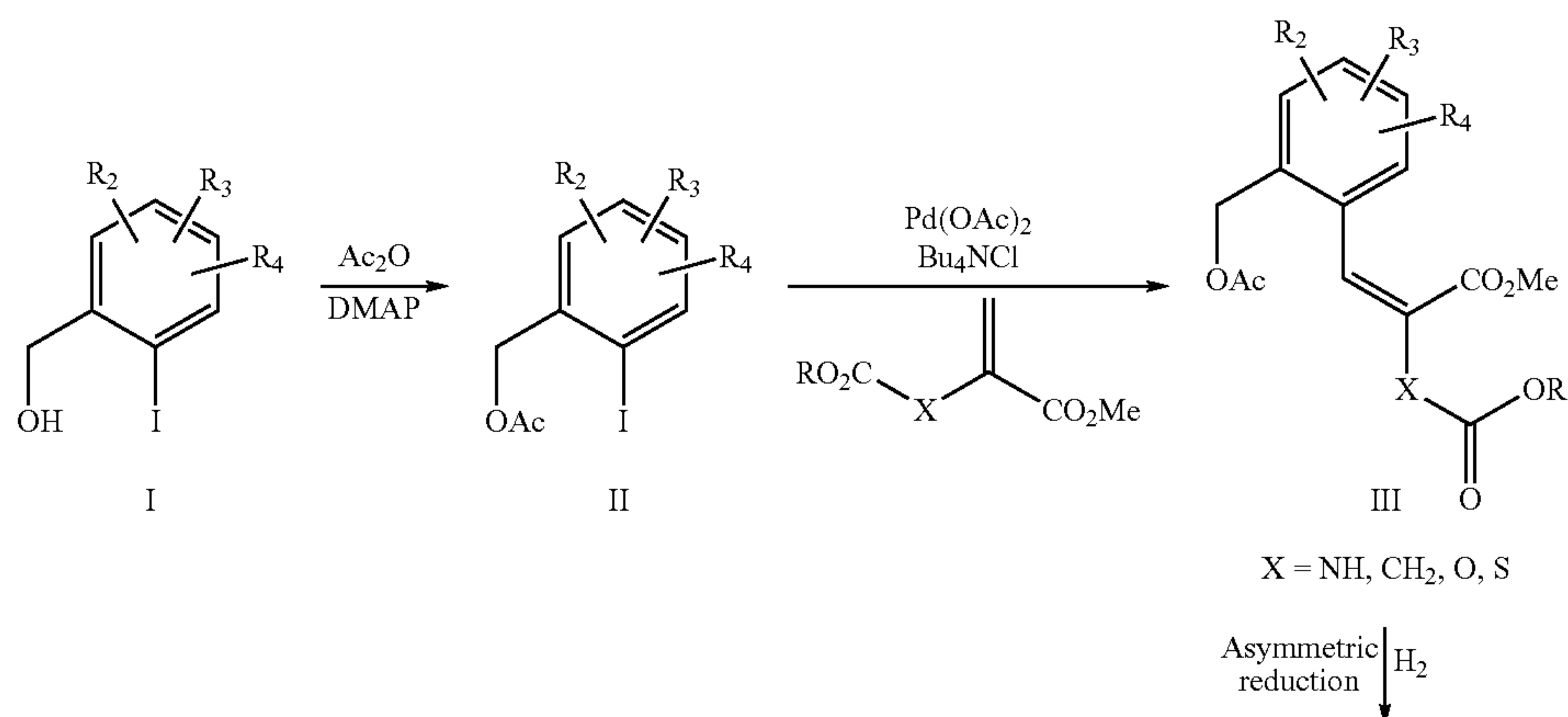
Scheme 1.
