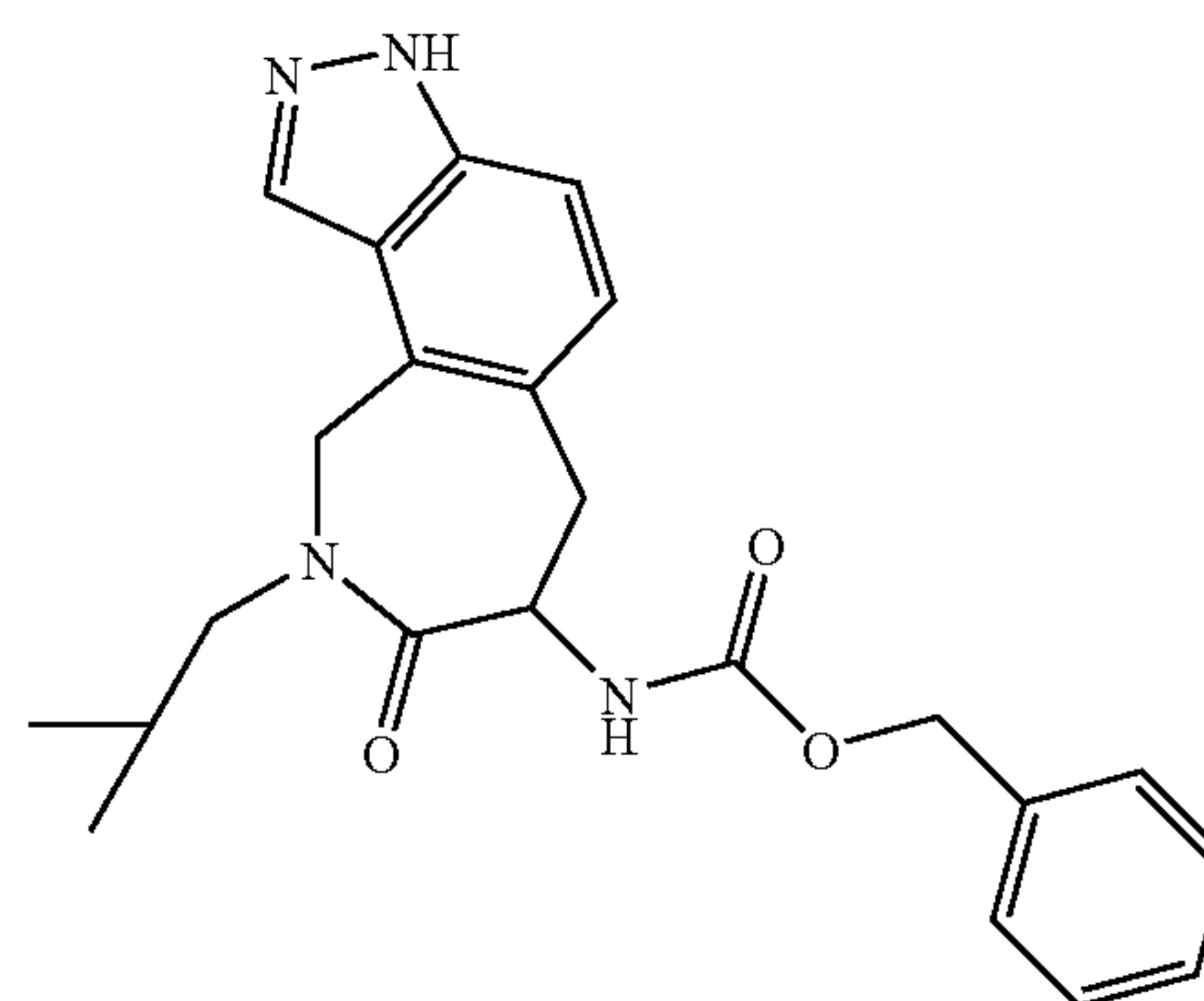
Intermediate 59
