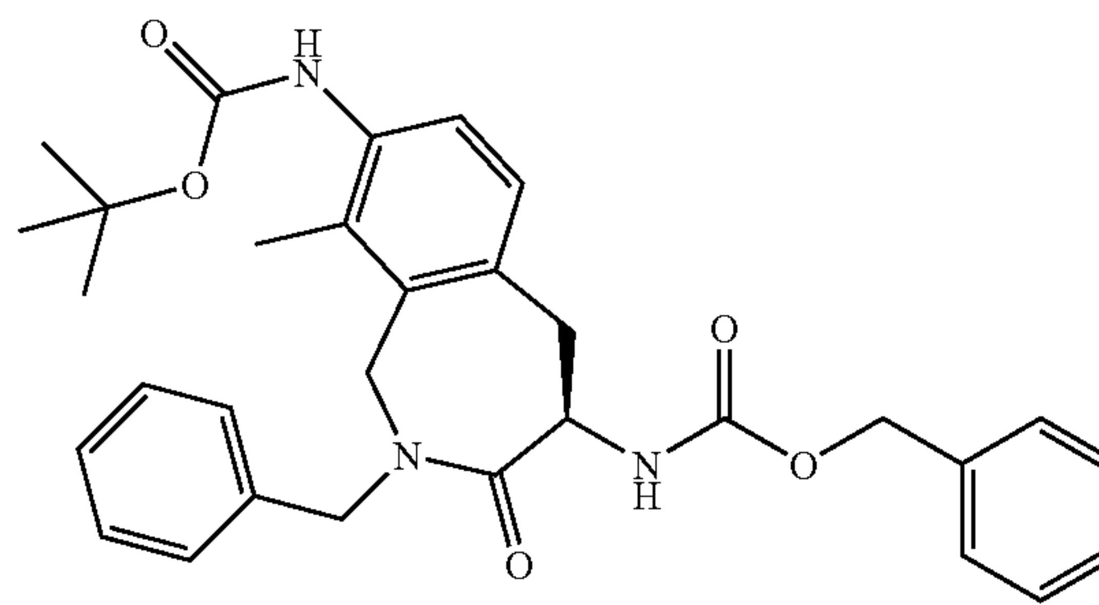
Intermediate 82
