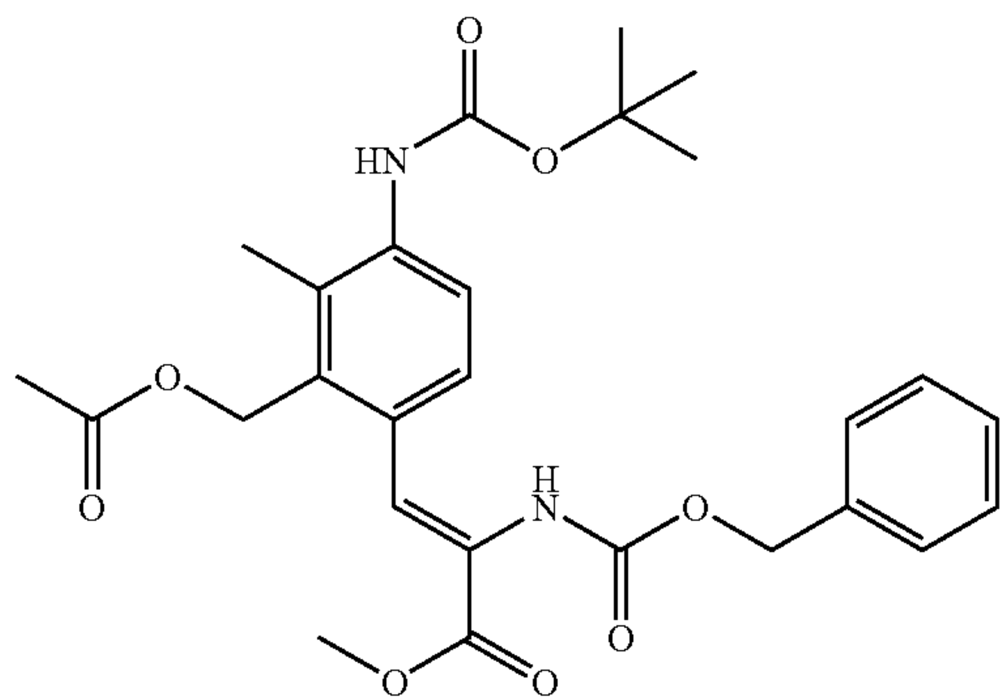
Intermediate 228
