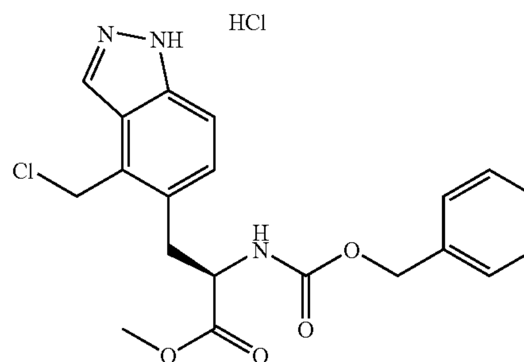
Intermediate 17
