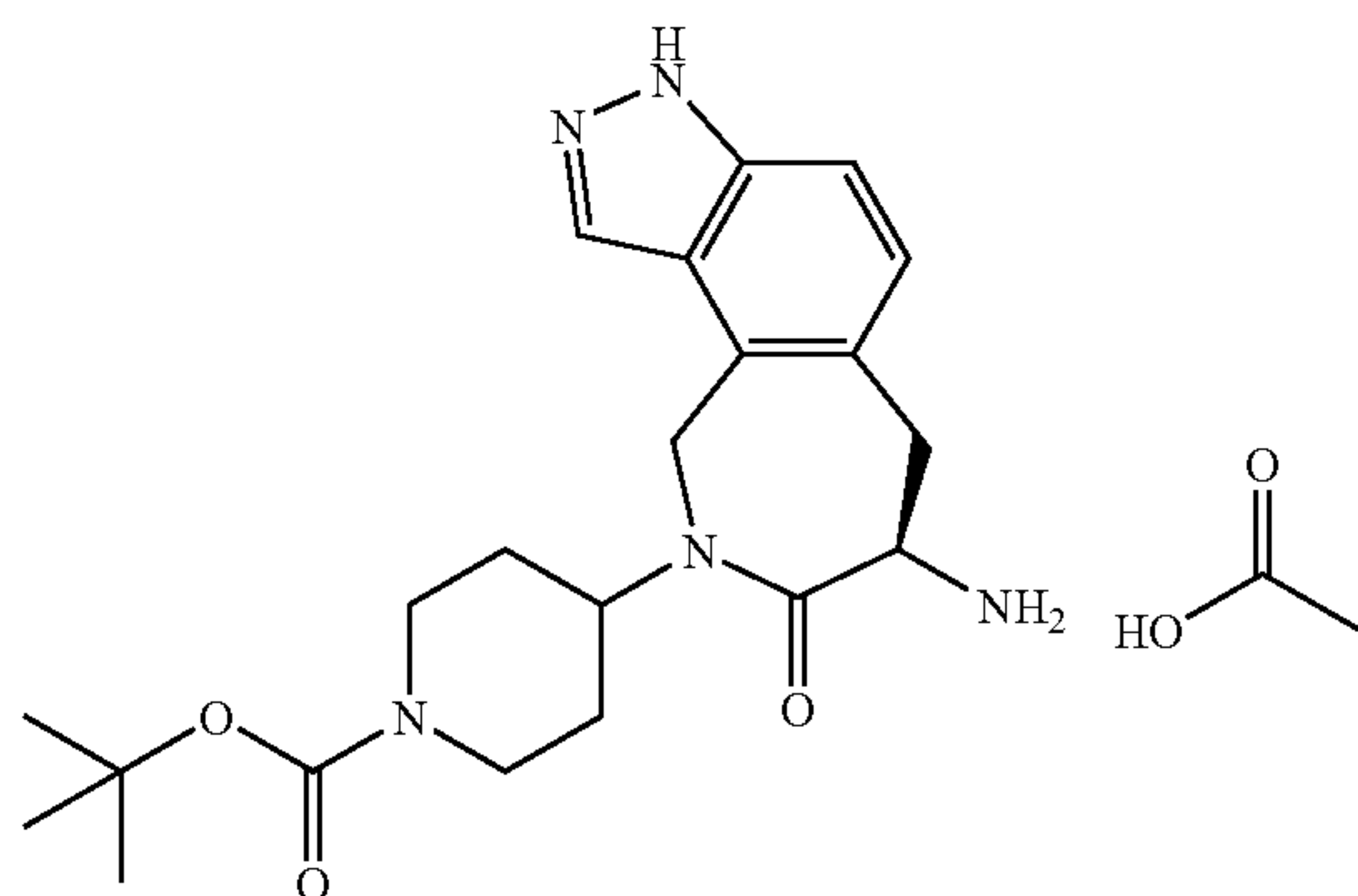
Intermediate 42
