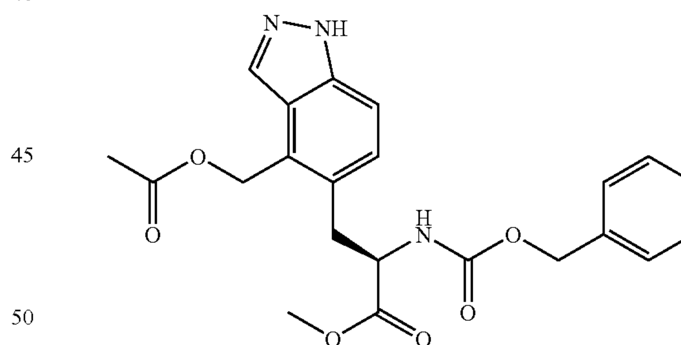
Intermediate 230
