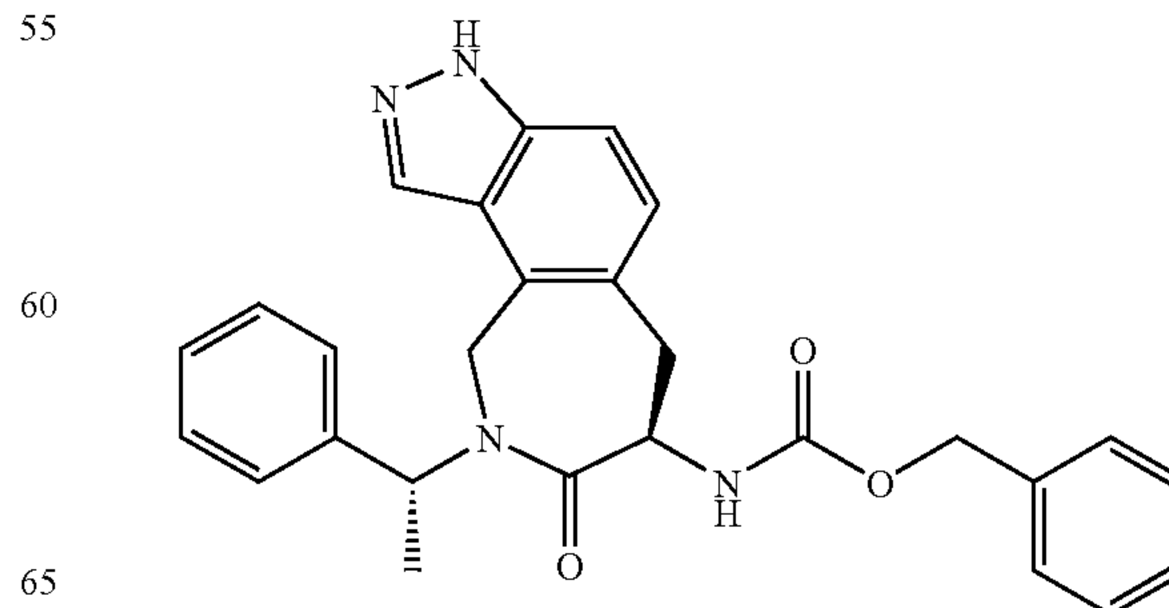
Intermediate 33
