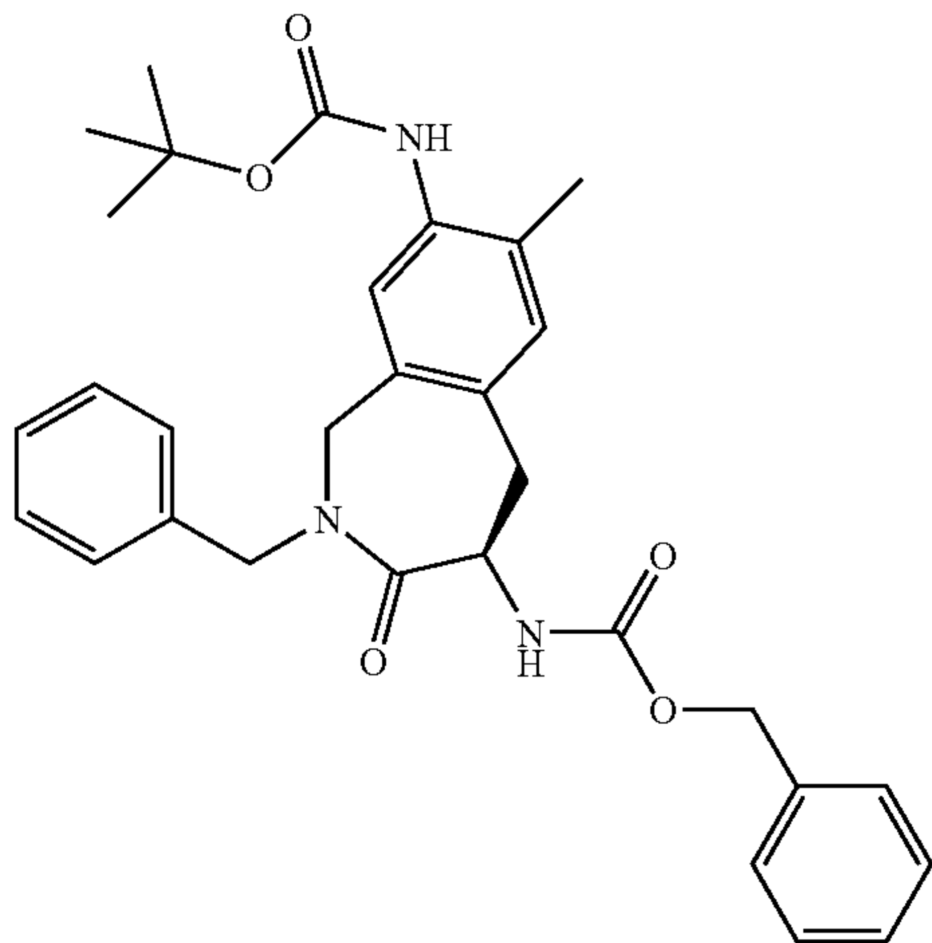
Intermediate 303
