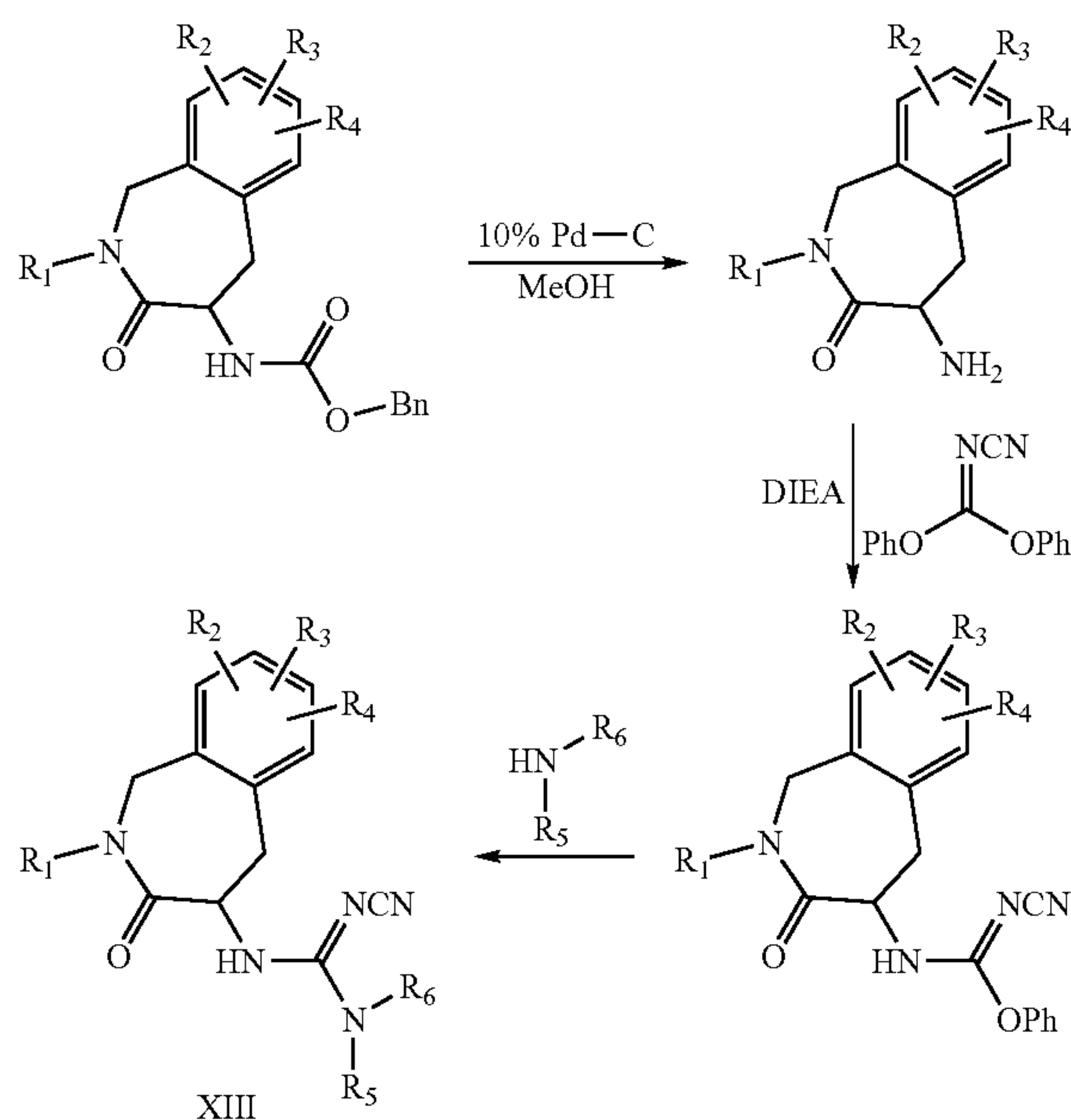
Scheme 4.
