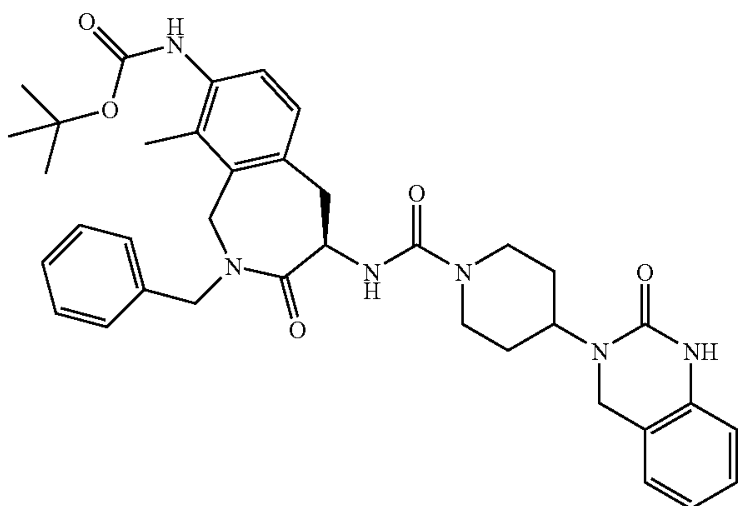
Intermediate 84
