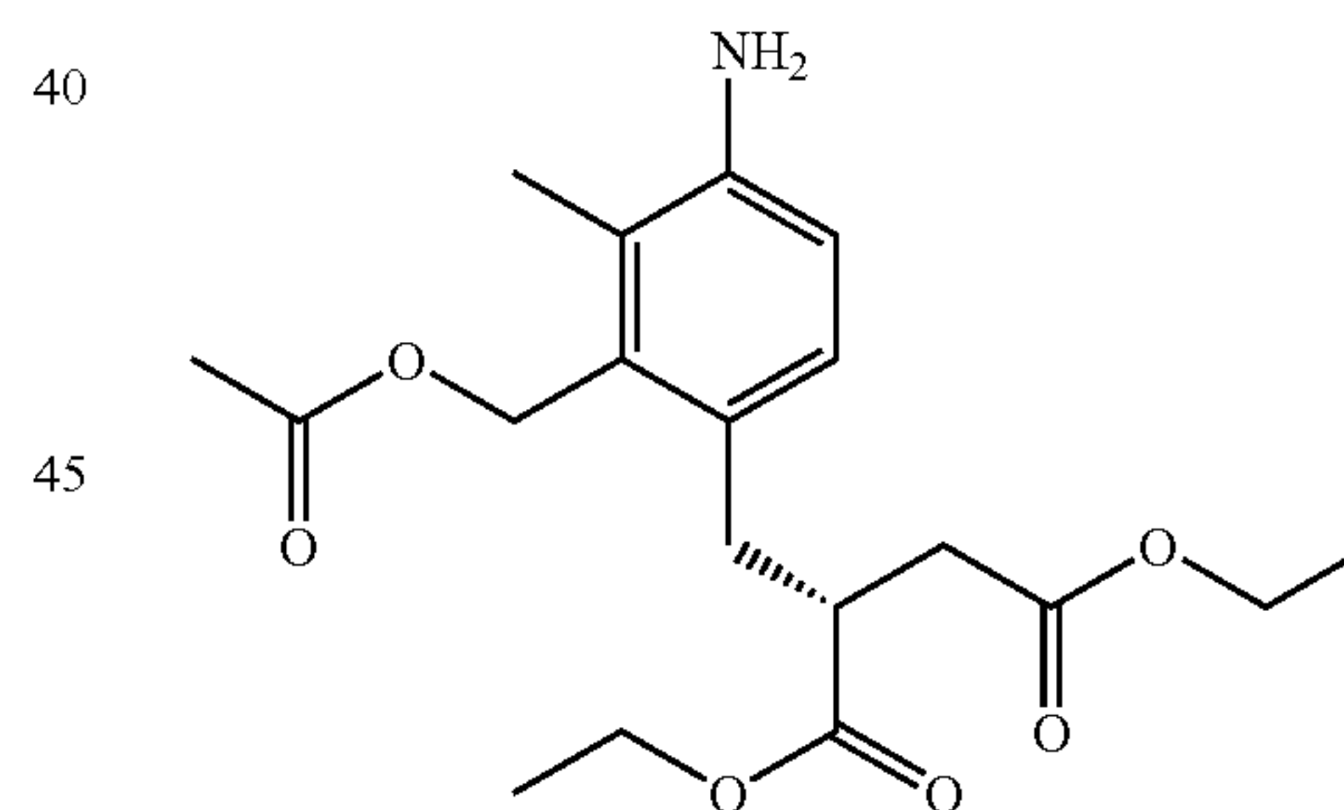
Intermediate 101
