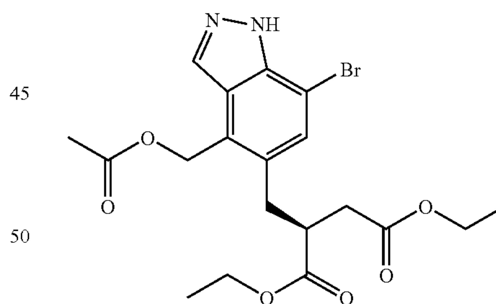
Intermediate 404
