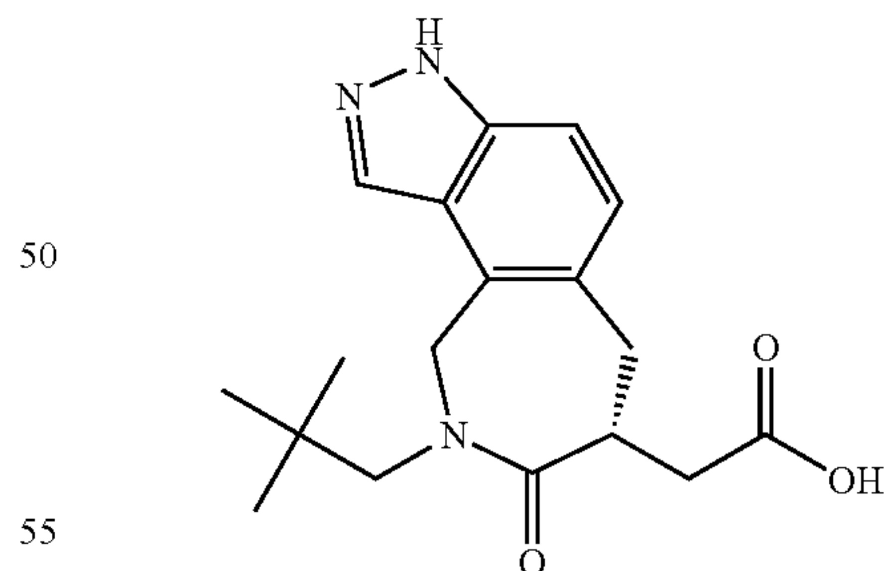
Intermediate 106
