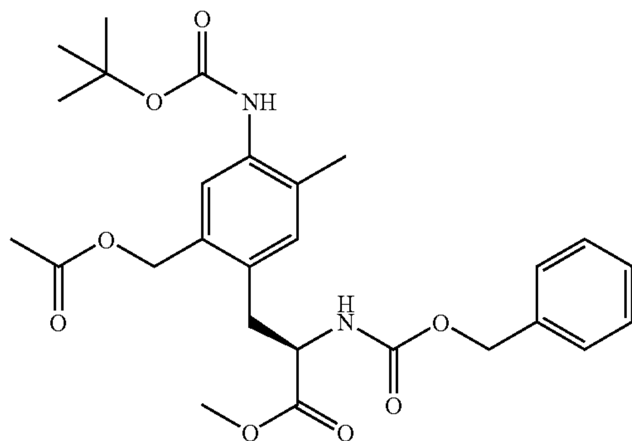
Intermediate 76
