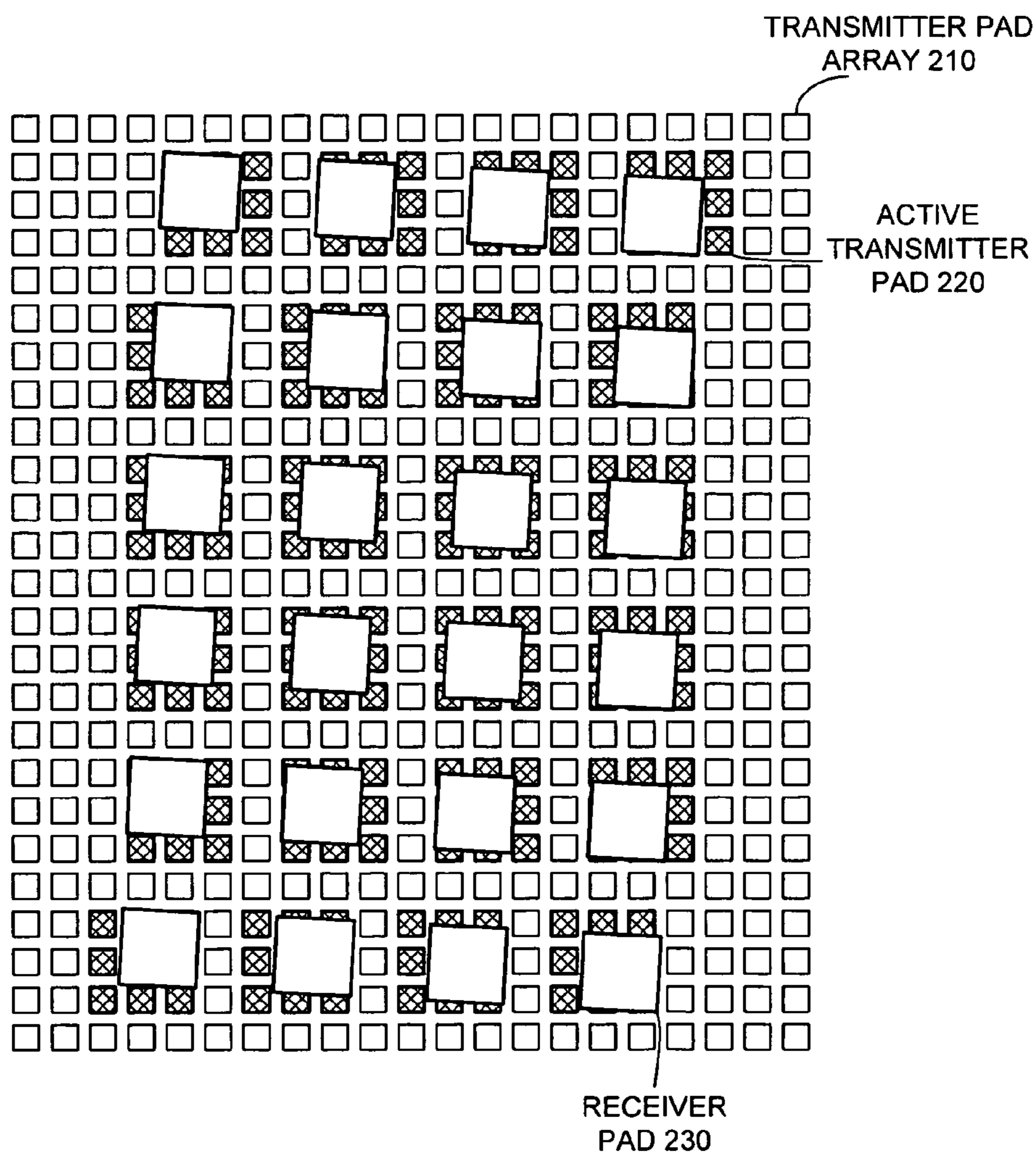
FIG. 2 (PRIOR ART)
