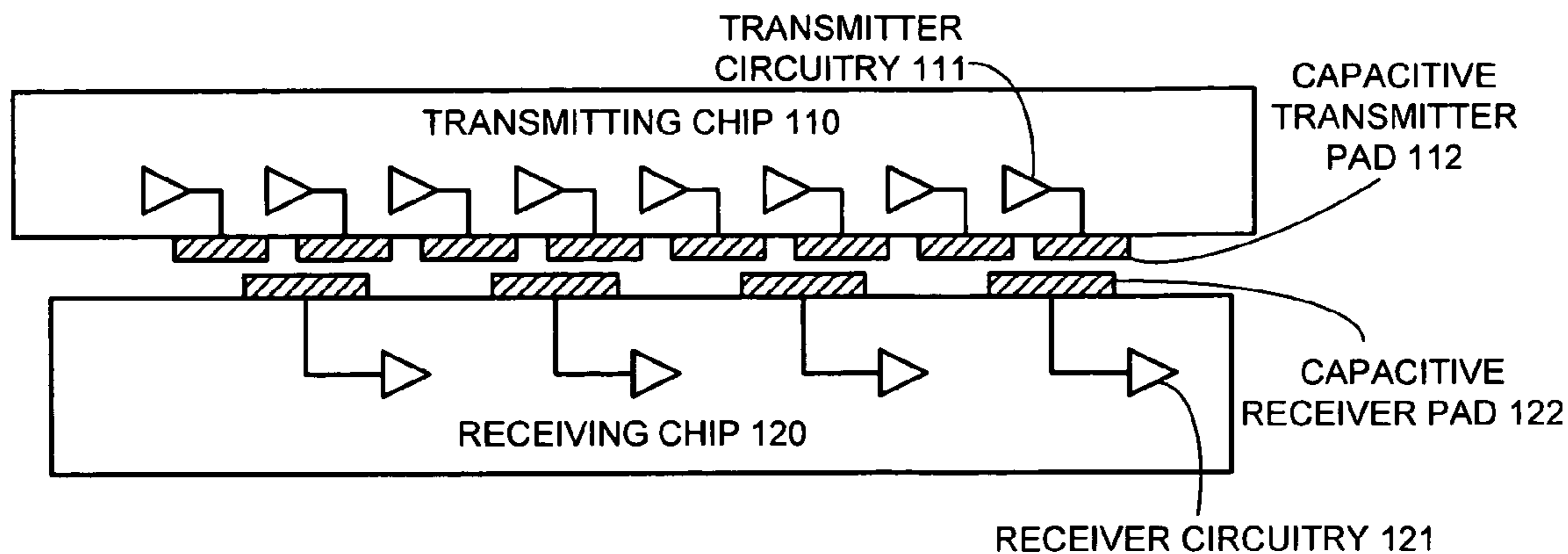
FIG. 1 (PRIOR ART)
