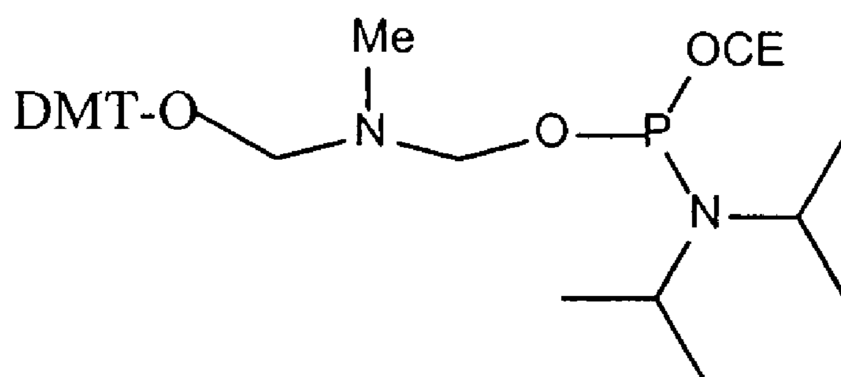
Neutral Phosphoramidite
