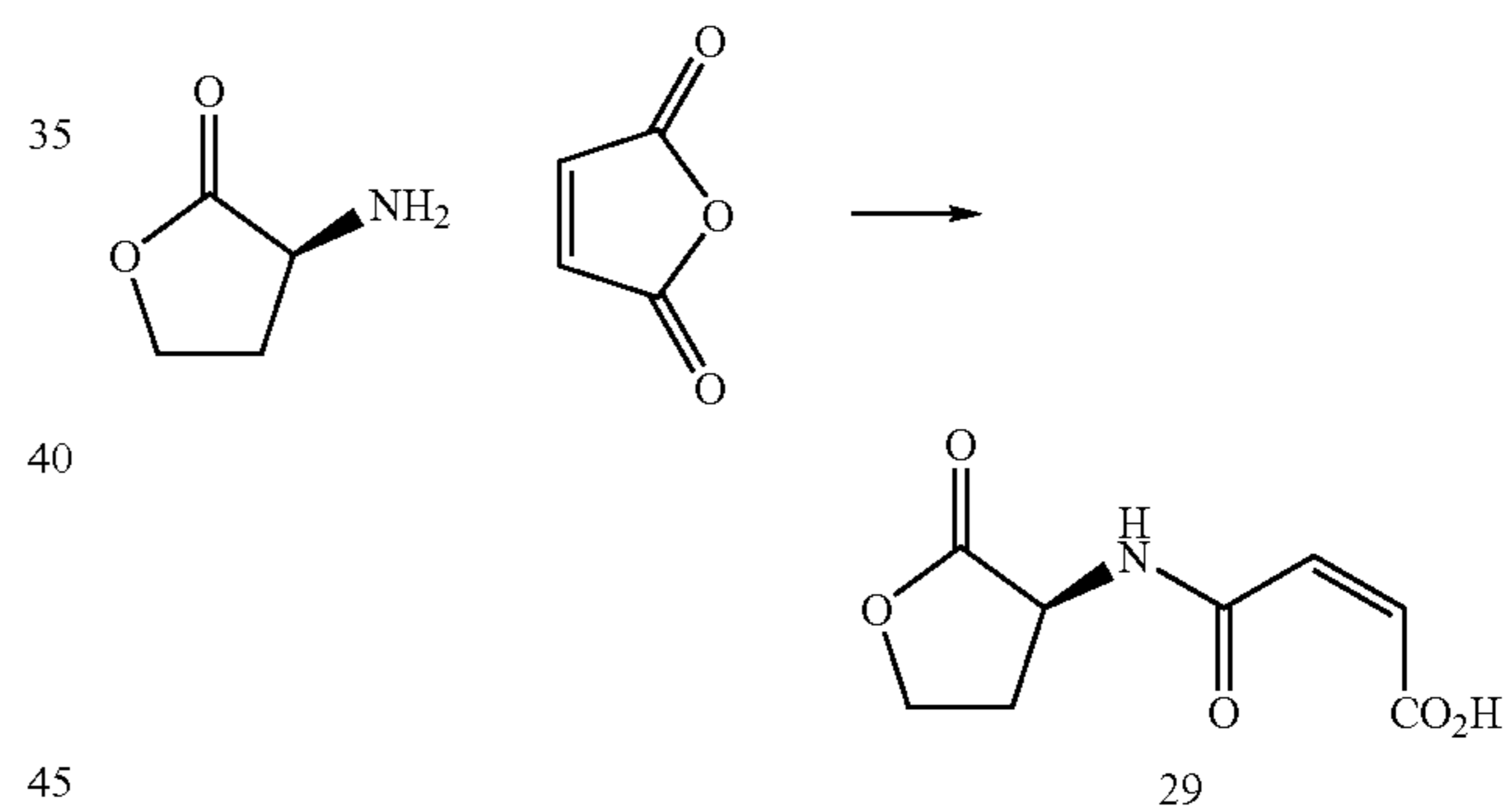
Scheme 7
