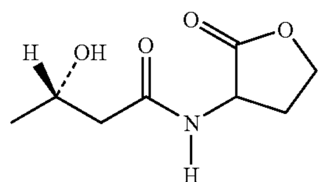
N-(3-hydroxy)-butanoyl-L-homoserine lactone
