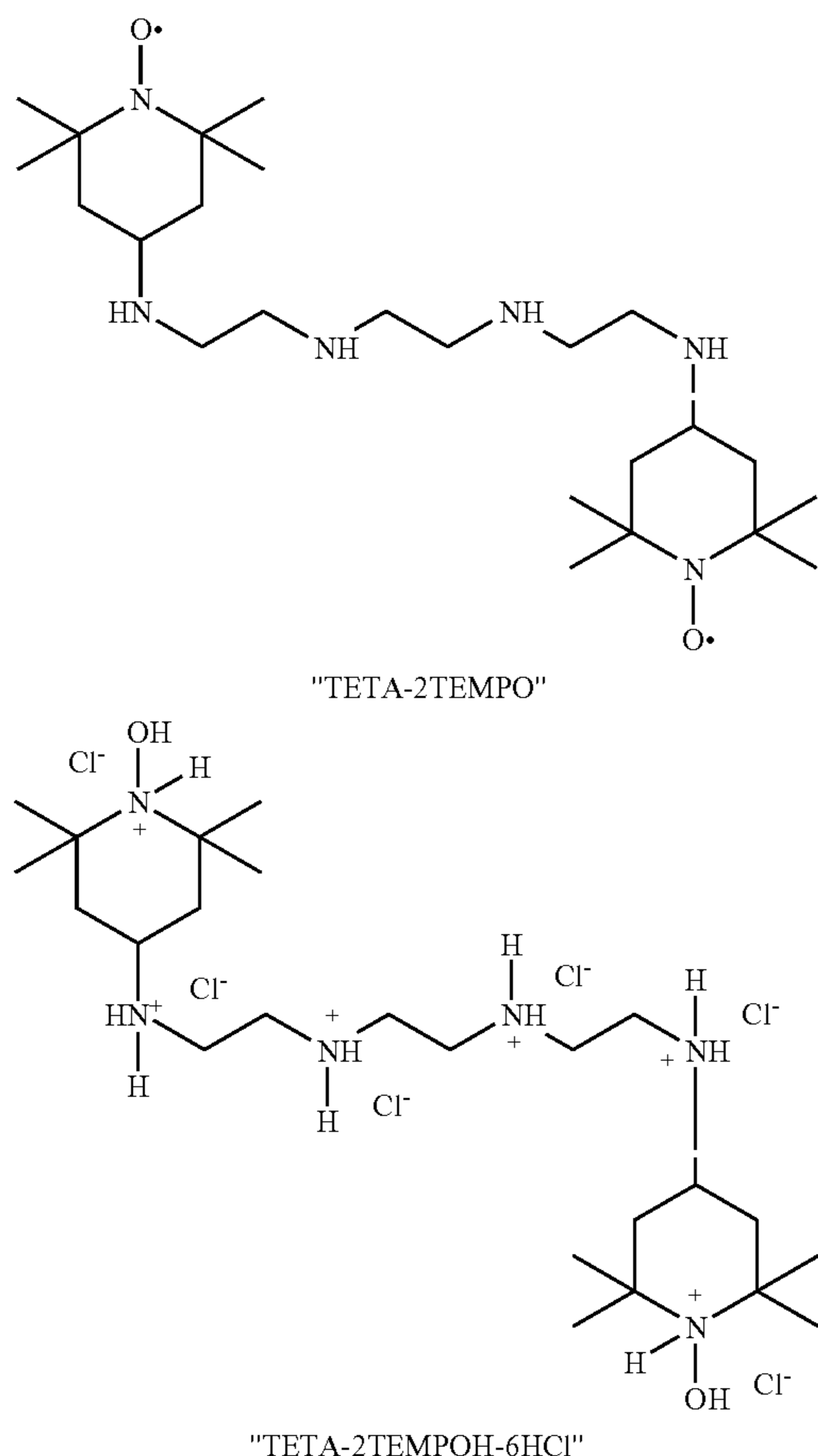
Scheme 1. Structures of TETA-2TEMPO and TETA-2TEMPOH-6HCl.
