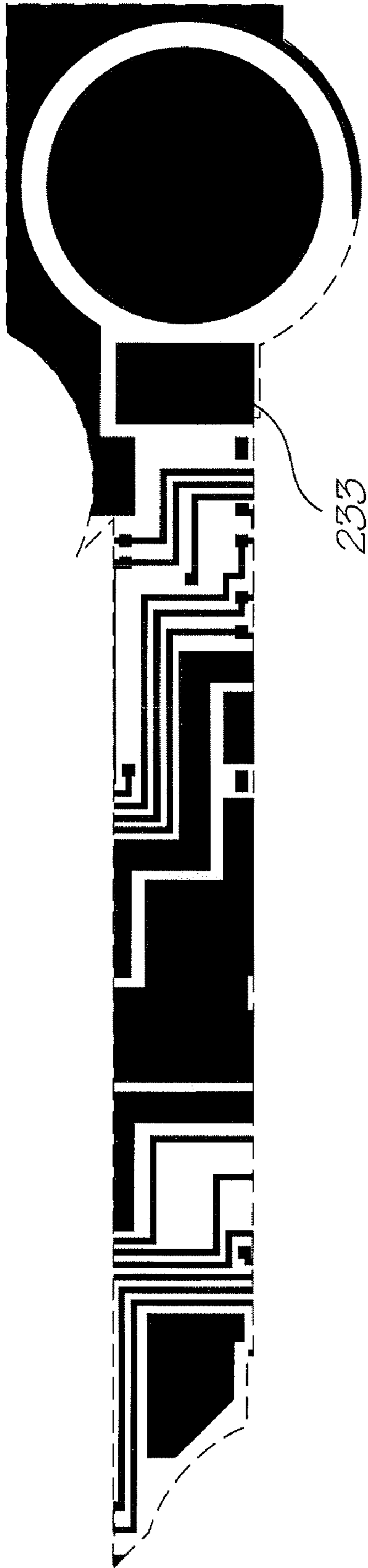
Metal 2 mask
