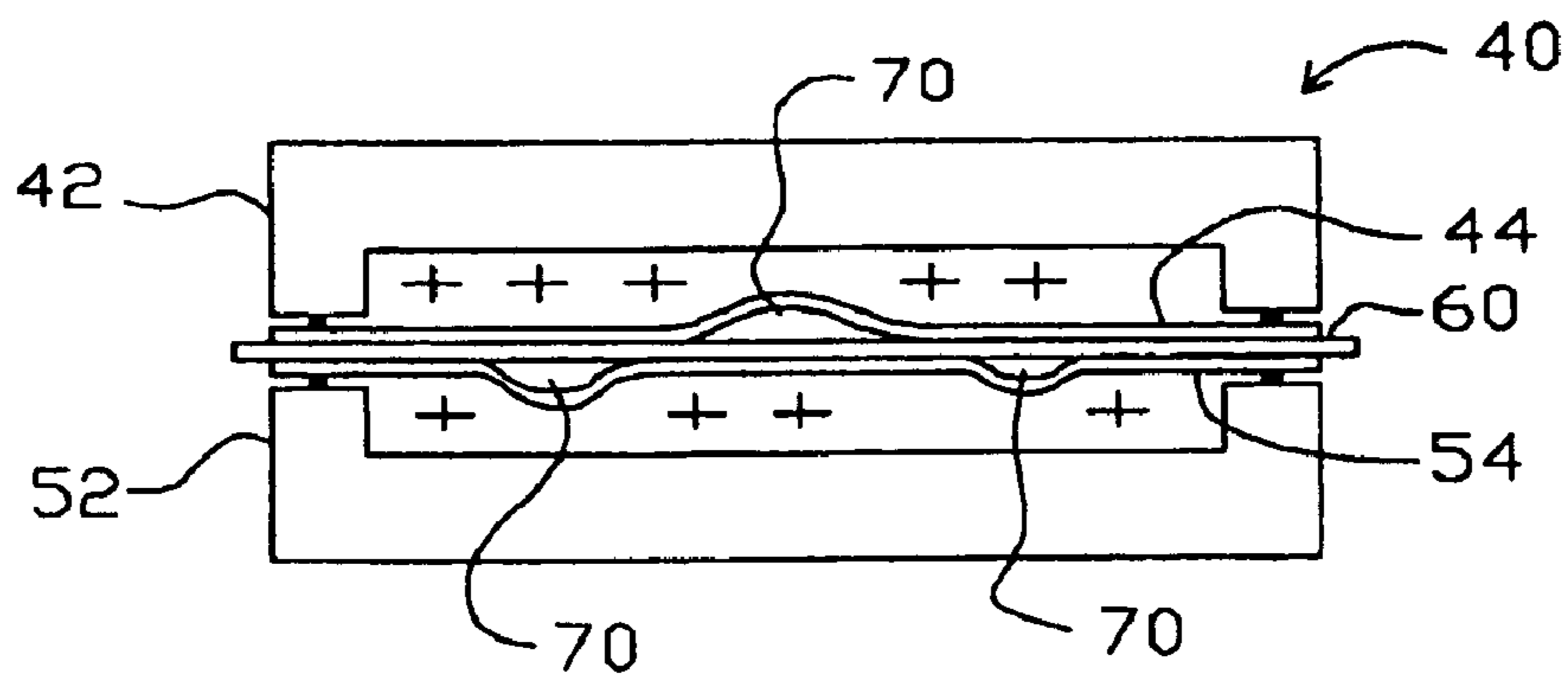
FIG 5 PRIOR ART
