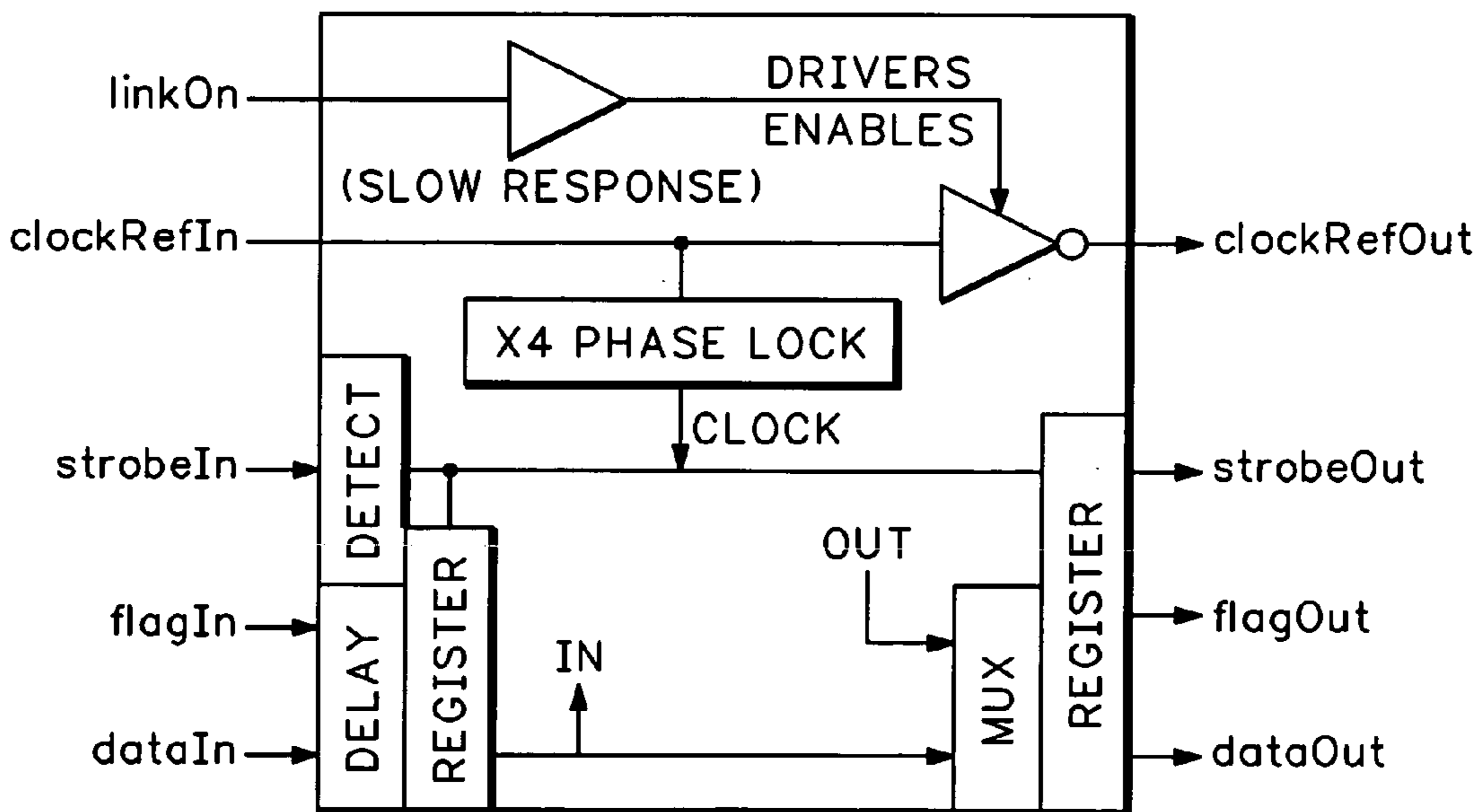
FIG. 2 (PRIOR ART)
