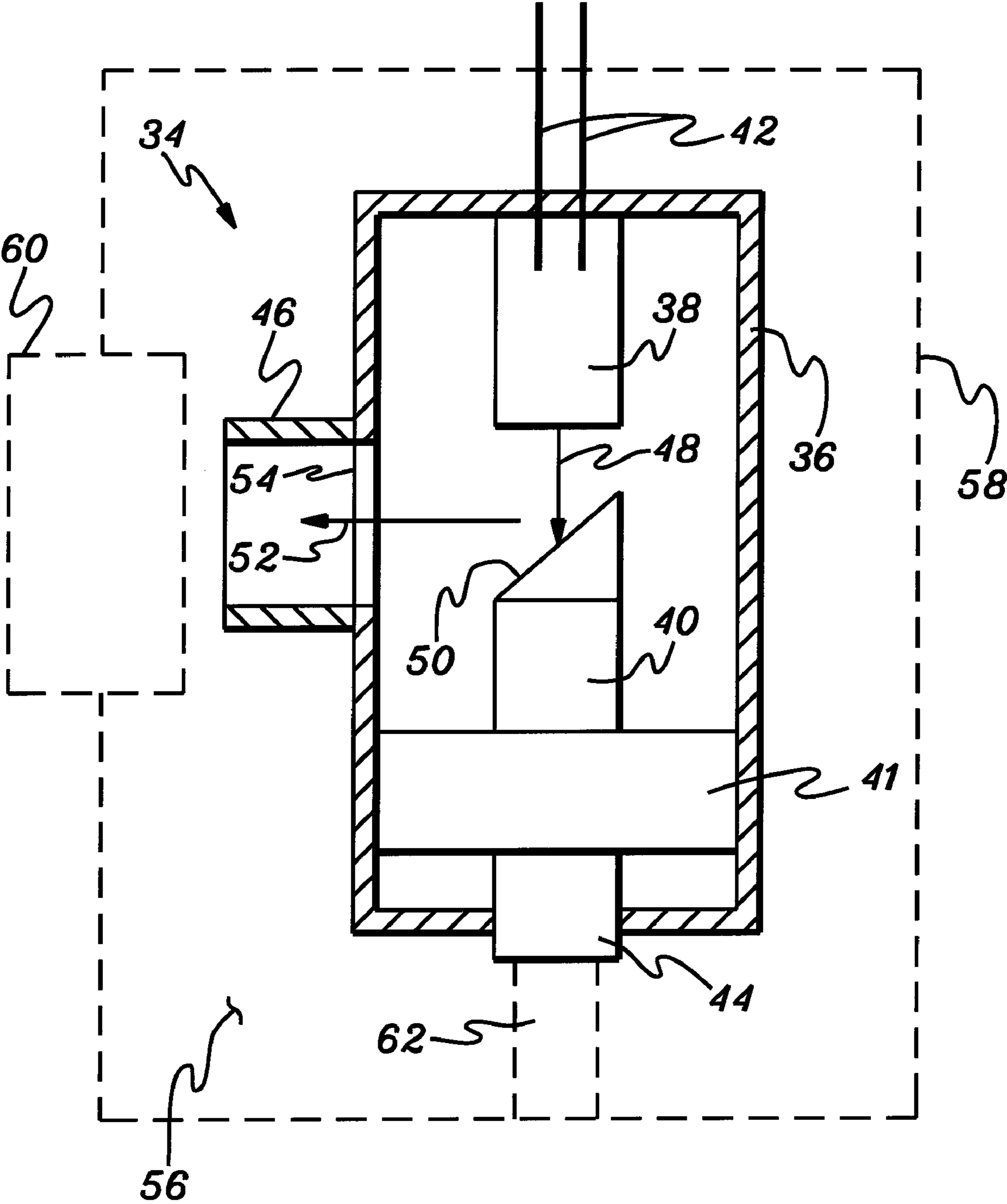
fig. 2 (PRIOR ART)
