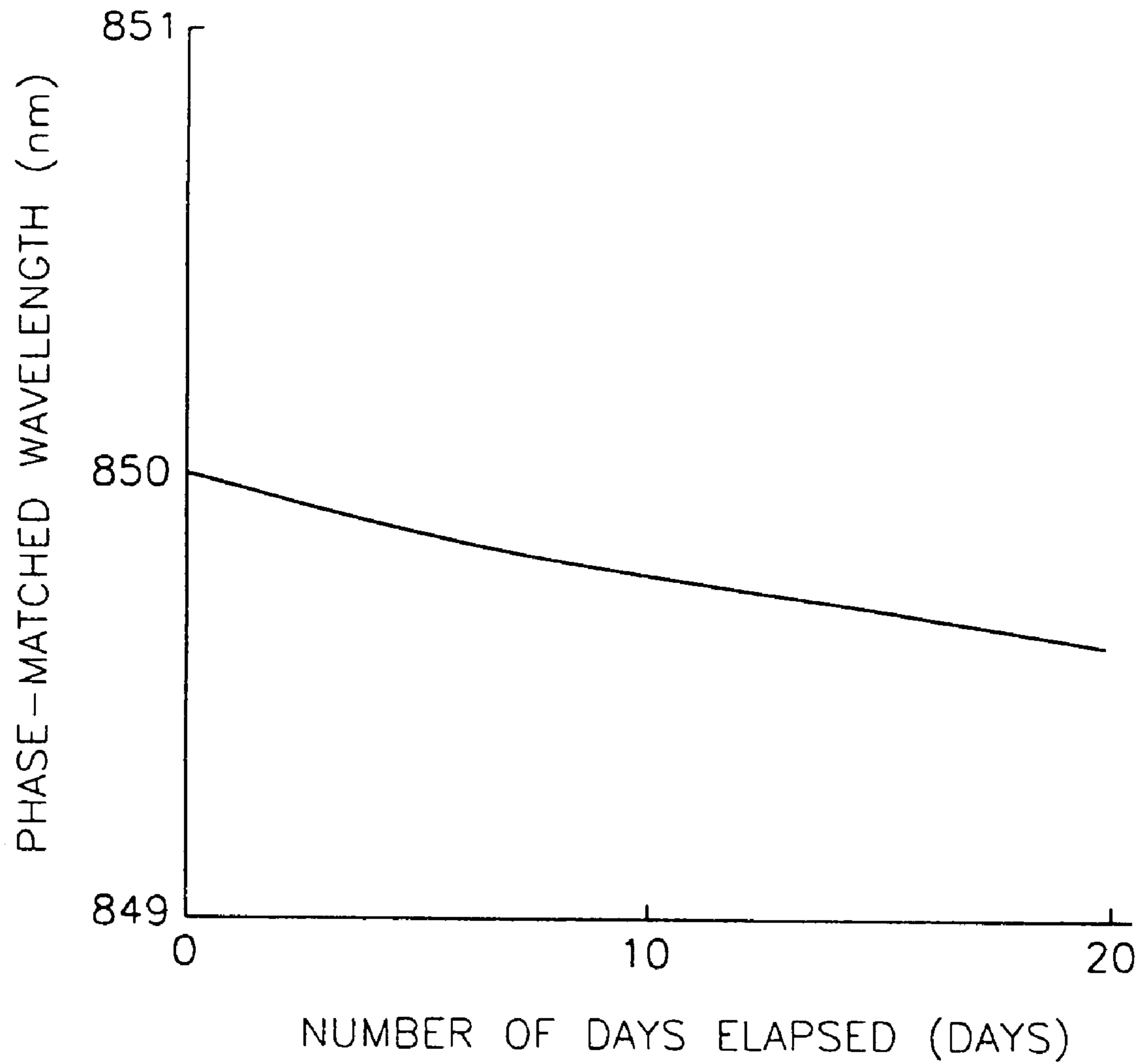
FIG. 5 (Prior Art)
