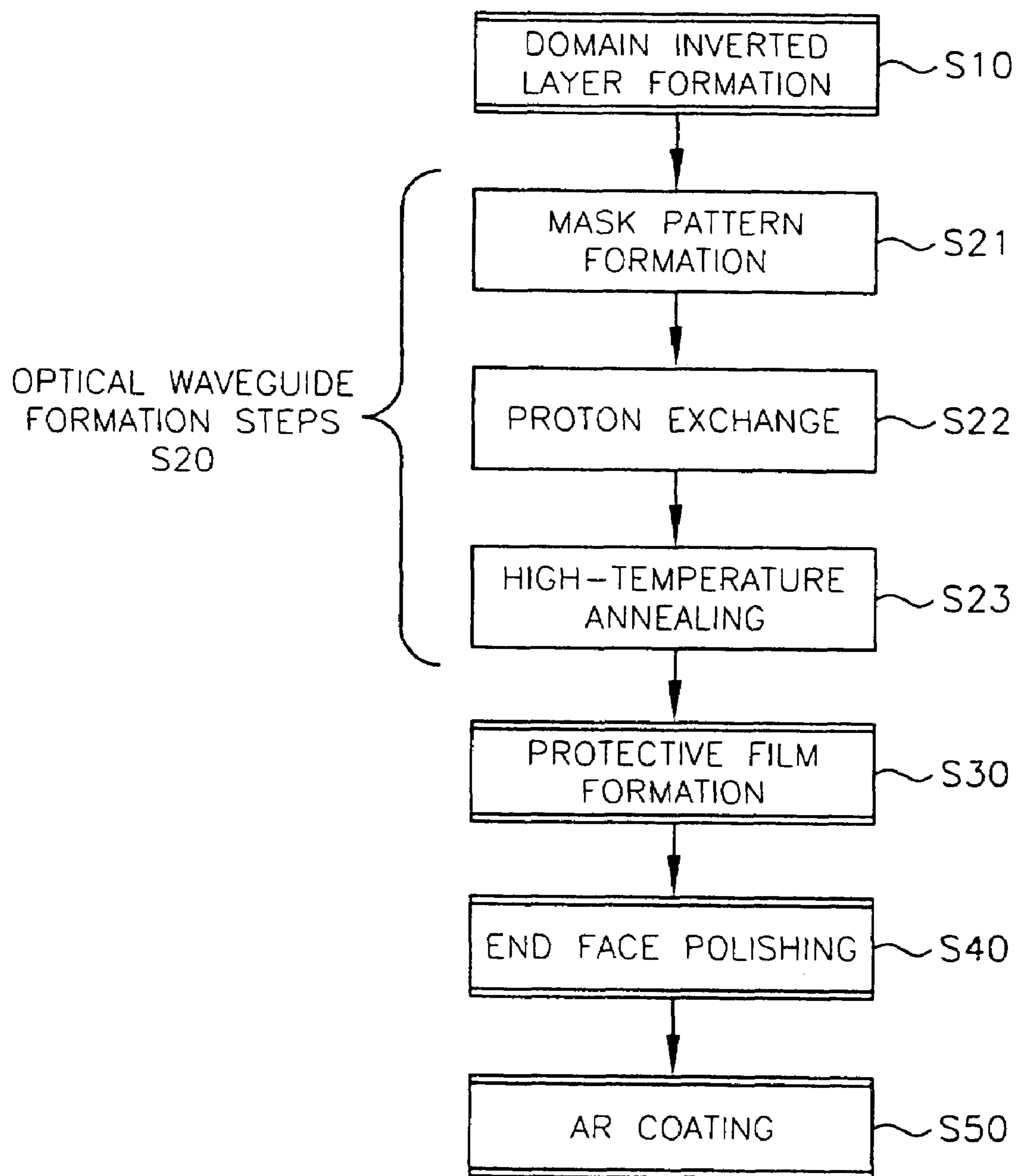
FIG. 3 (Prior Art)
