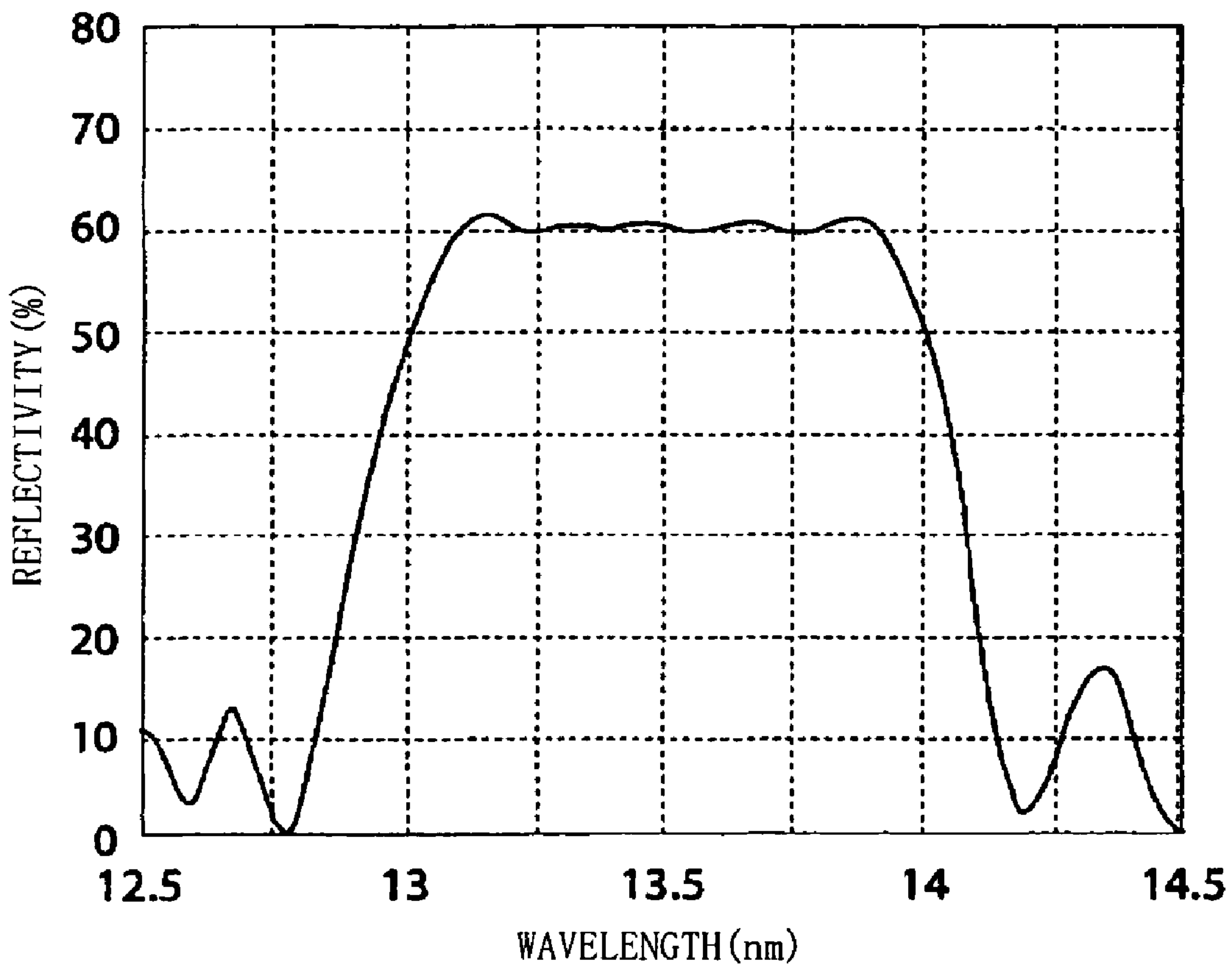
SPECTRAL REFLECTIVITY (AT VERTICAL INCIDENCE)
