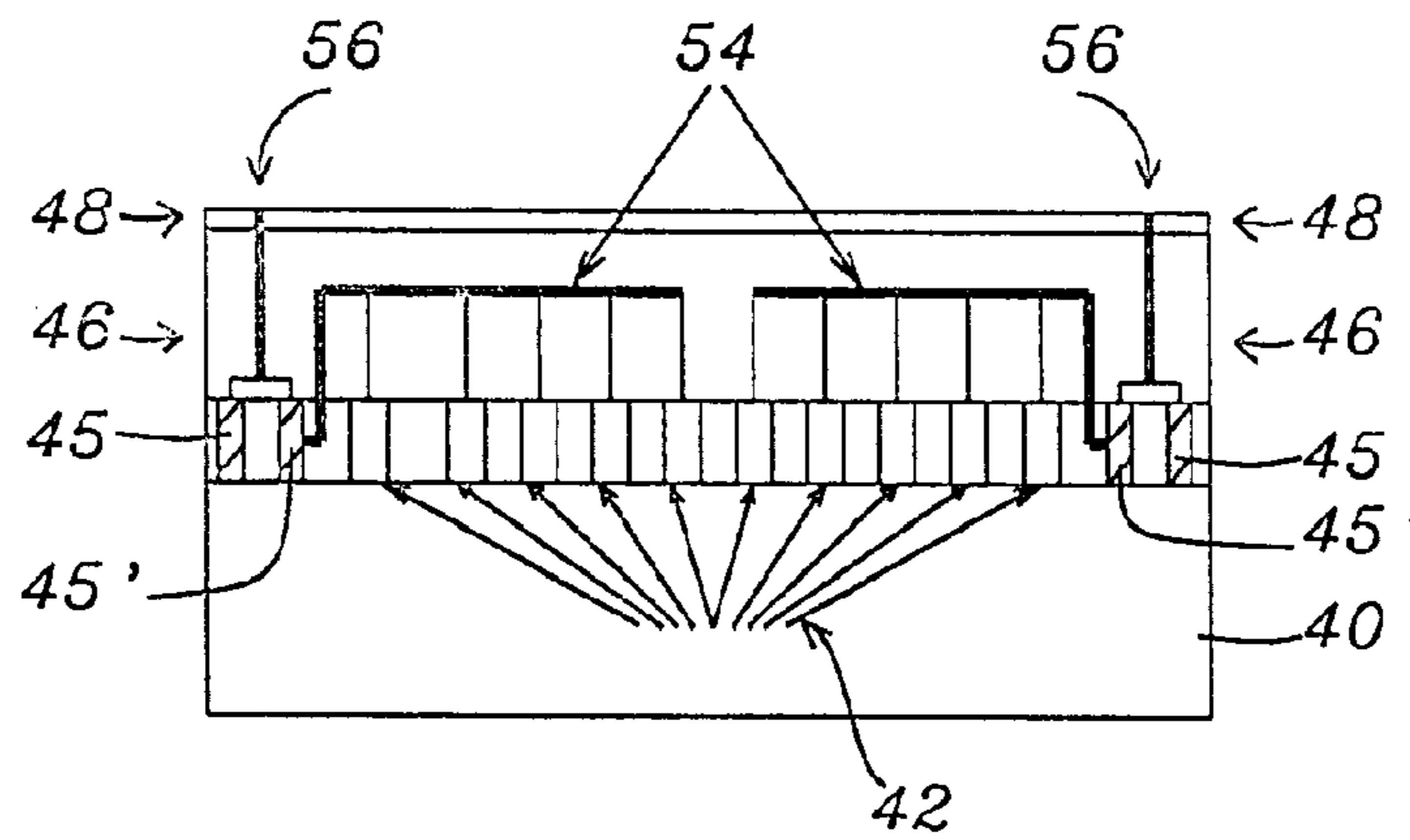
FIG. 2 - Prior Art
