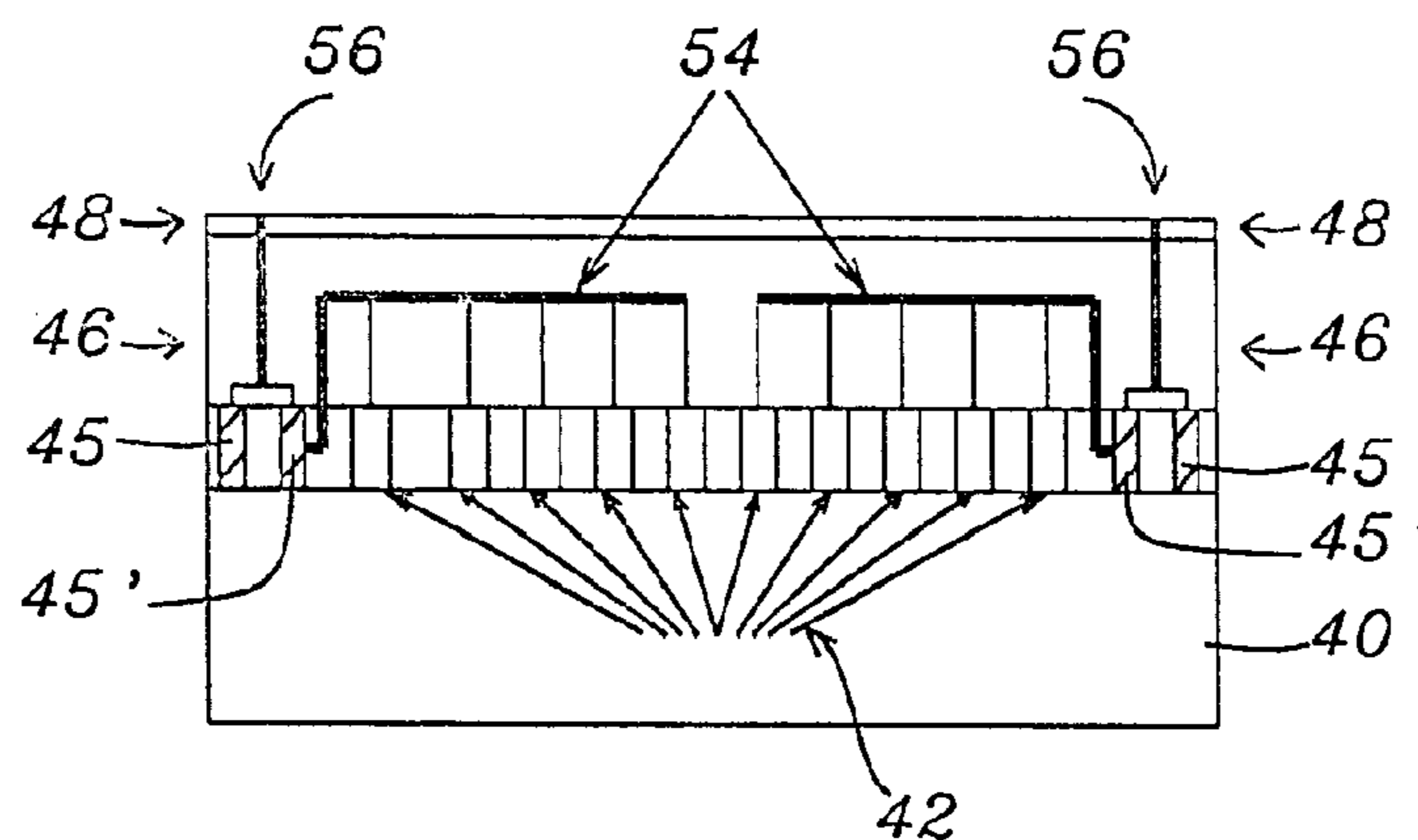
FIG. 2 - Prior Art
