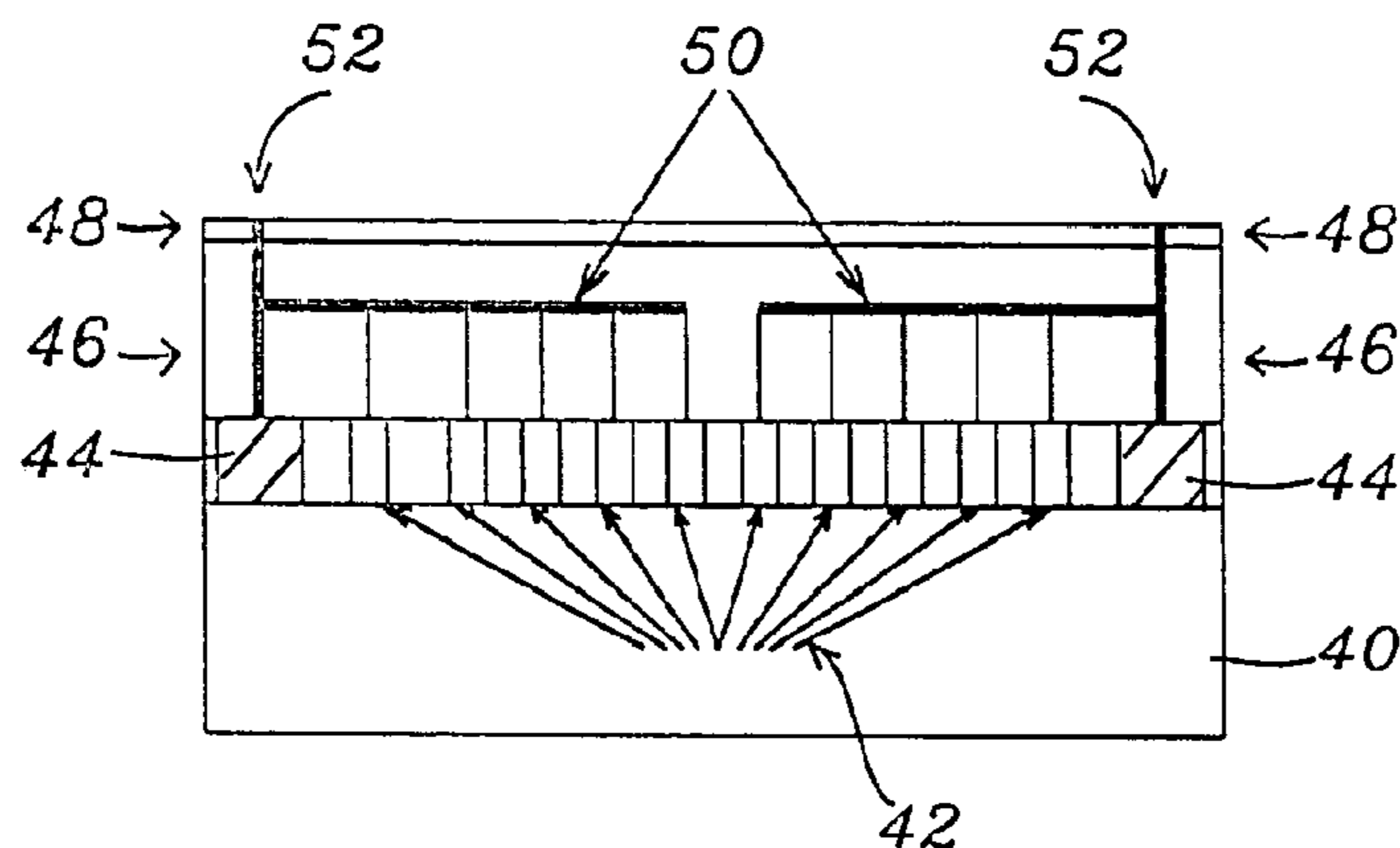
FIG. 1 - Prior Art
