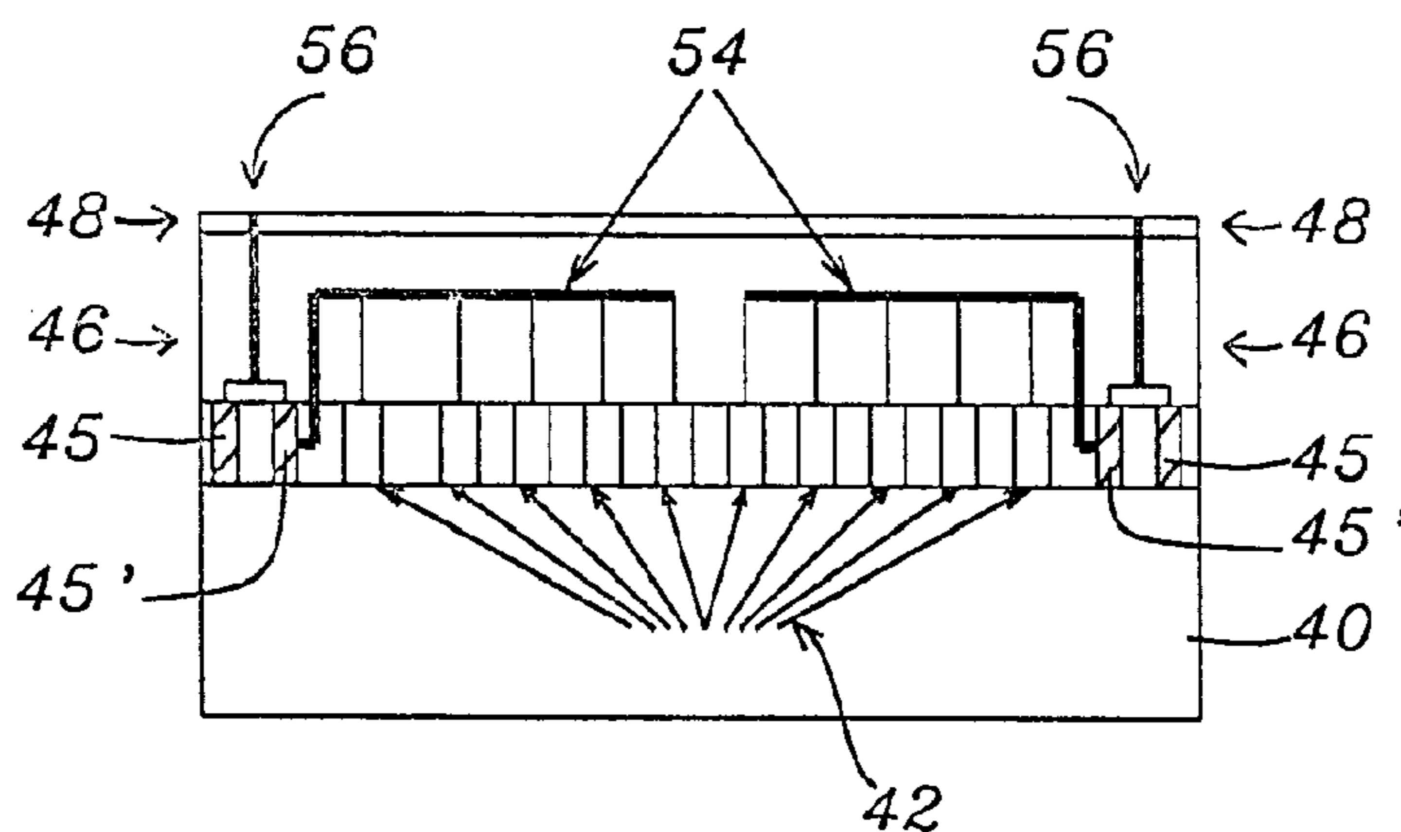
FIG. 2 - Prior Art
