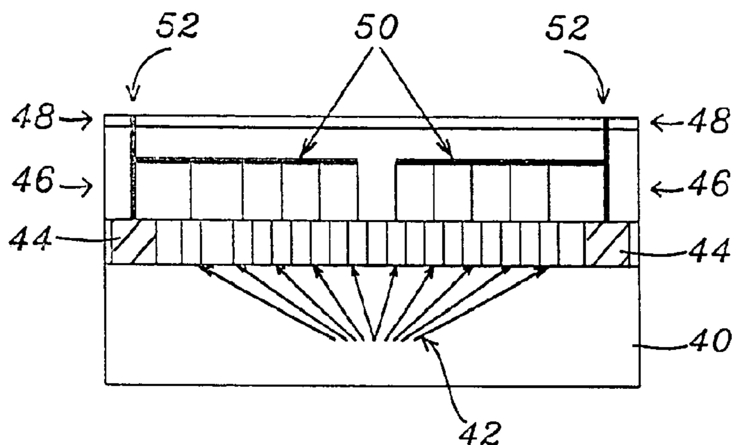
FIG. 1 - Prior Art
