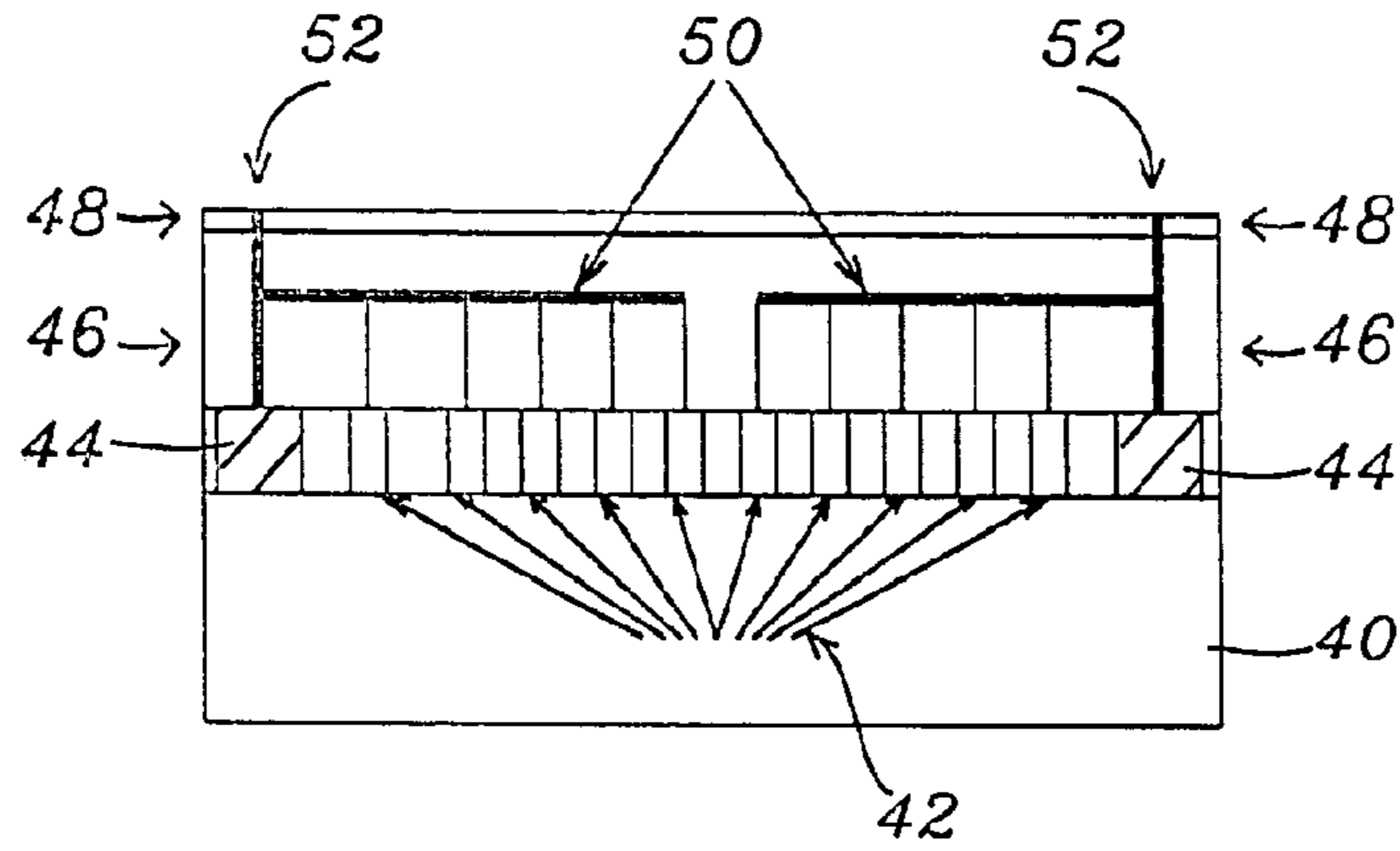
FIG. 1 - Prior Art
