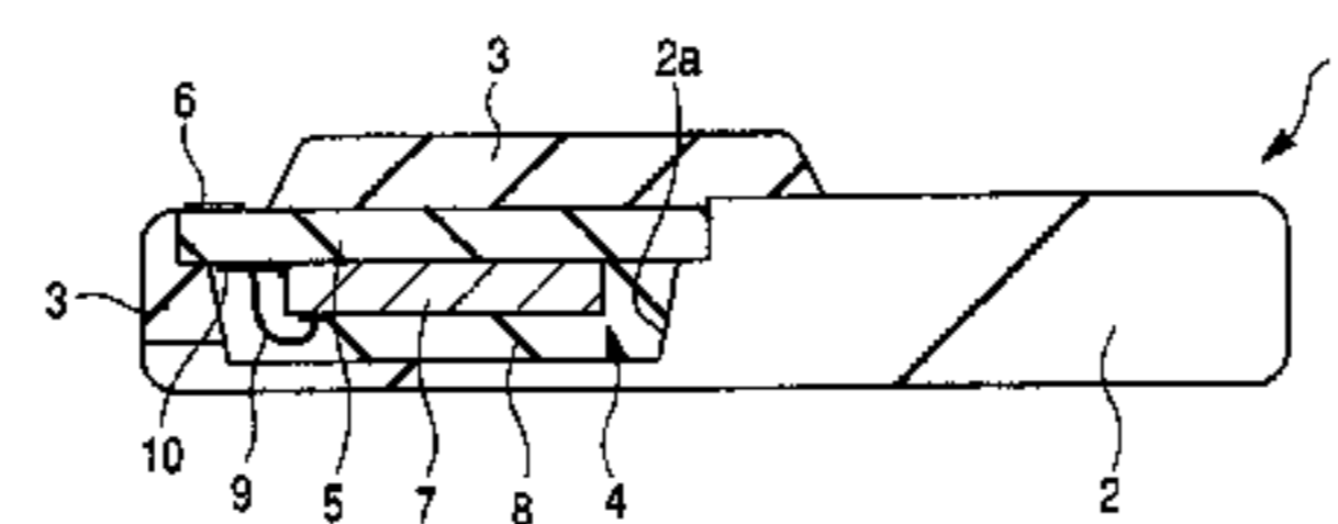
1: IC CARD 2: CASE 3: SEALING PORTION 4: IC BODY 5: WIRING SUBSTRATE 6: EXTERNAL CONNECTION TERMINAL 7: SEMICONDUCTOR CHIP 8: SEALING PORTION 9: BONDING WIRE
