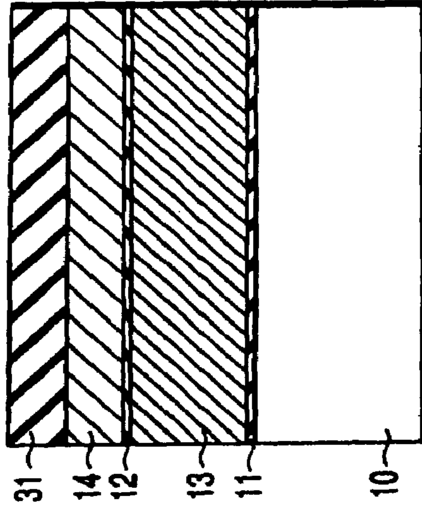
Section of memory cell area in direction of gate length (B-B line section of FIG.1)
