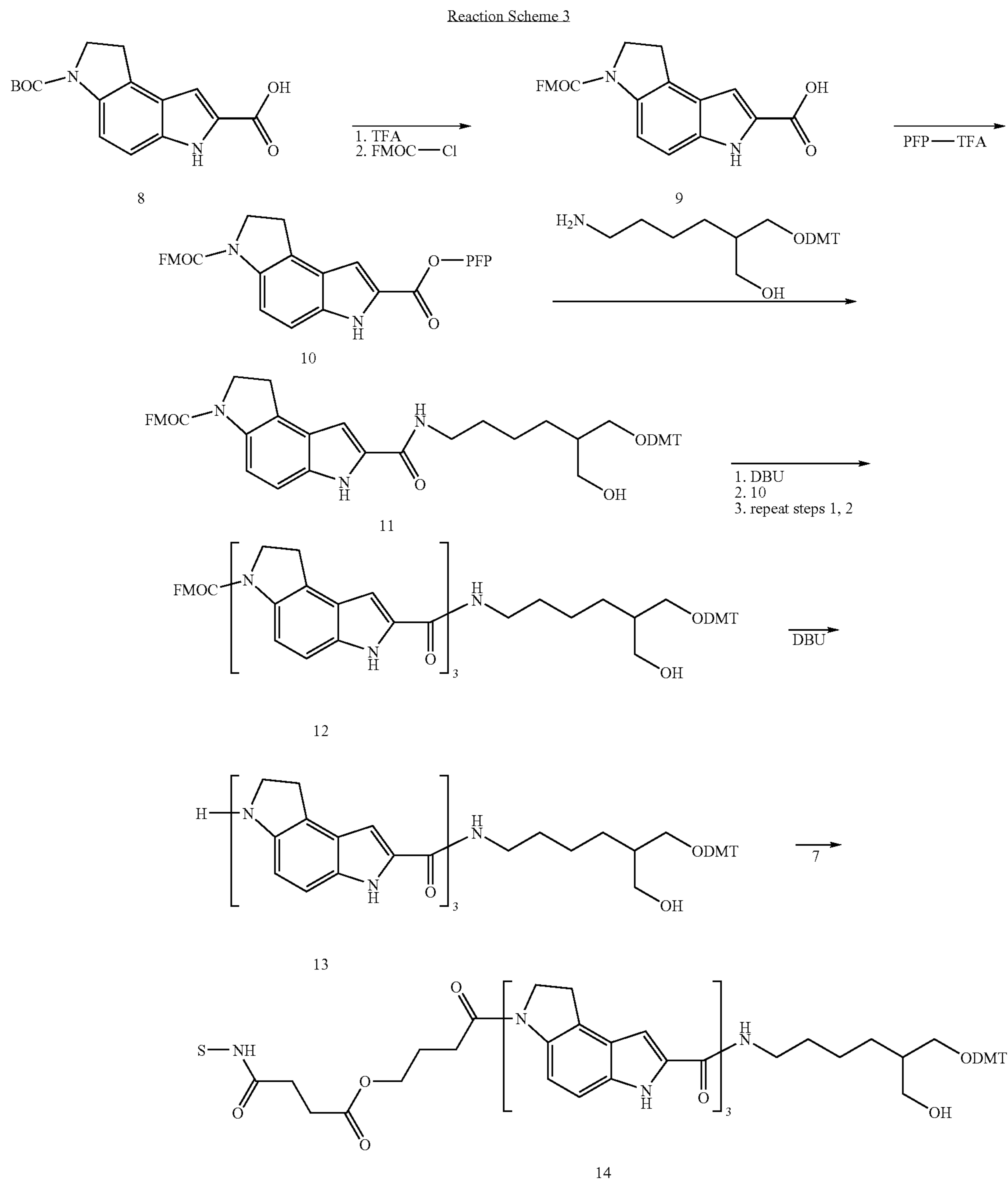
FIG. 7 schematically shows a particularly preferred way to assemble the MB-FI-ODN-Q conjugates on a synthesizer.
